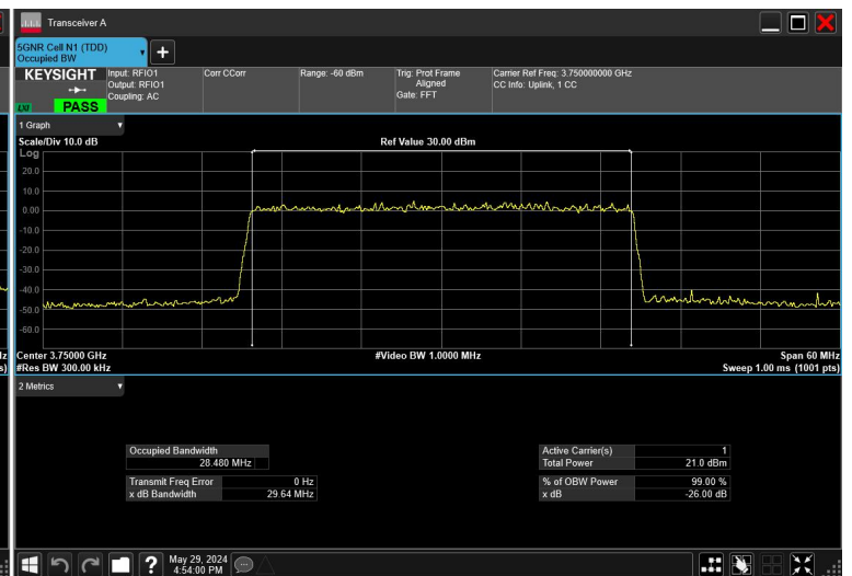
30MHz_15kHz_3750MHz_DFT-s-OFDM 64 QAM_RB160@0
