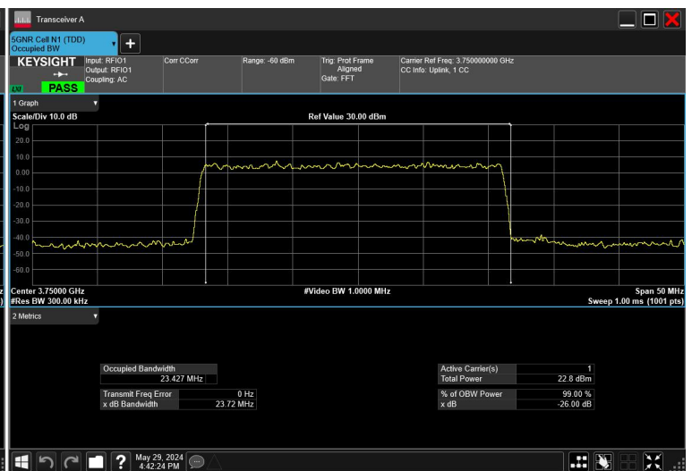
25MHz_15kHz_3750MHz_DFT-s-OFDM \pi/2 BPSK_RB128@0
