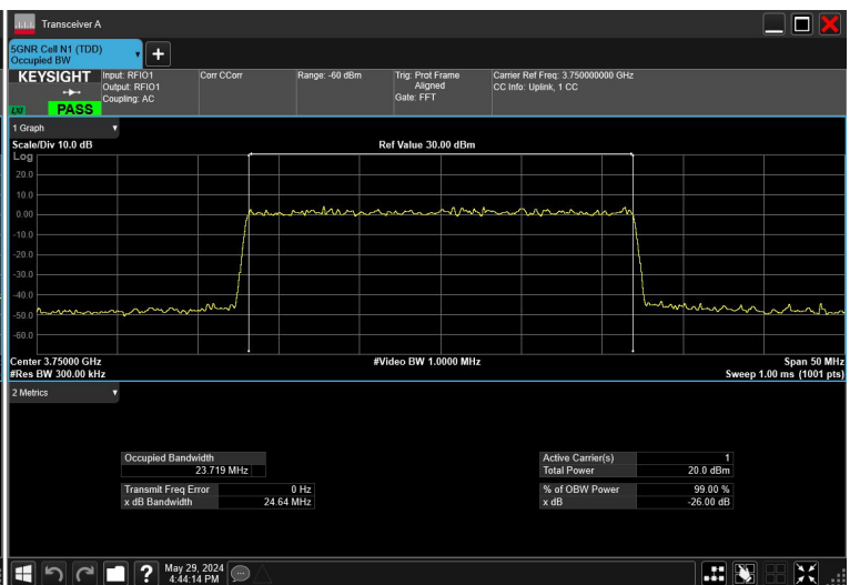
25MHz_15kHz_3750MHz_CP-OFDM 64 QAM_RB133@0
