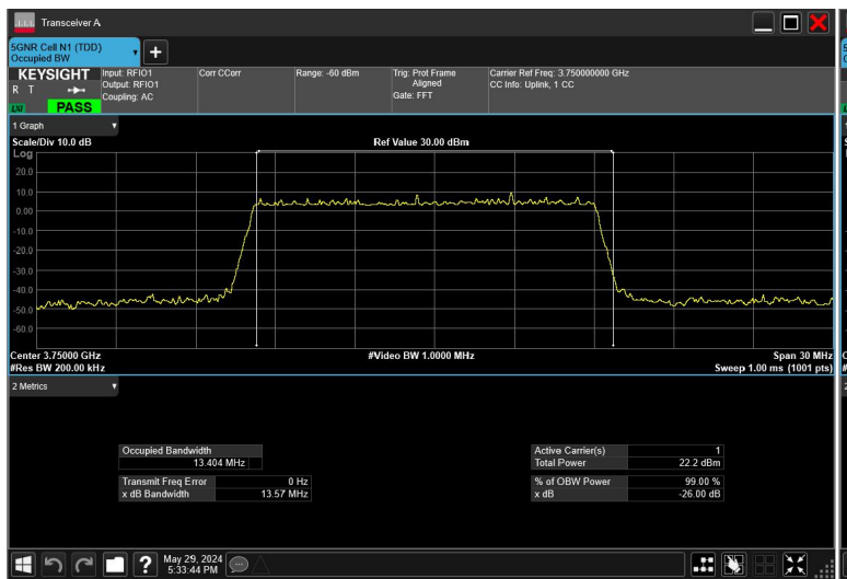
15MHz_30kHz_3750MHz_DFT-s-OFDM \pi/2 BPSK_RB36@0
