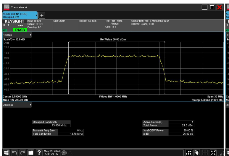
15MHz_30kHz_3750MHz_DFT-s-OFDM 16 QAM_RB36@0
