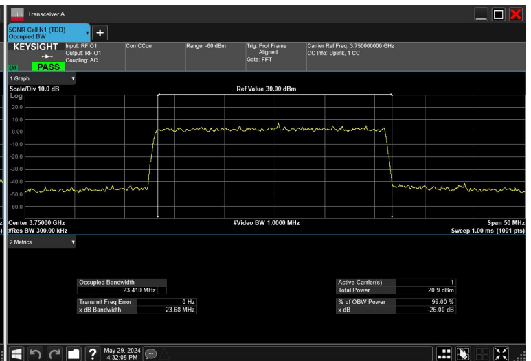
25MHz_15kHz_3750MHz_DFT-s-OFDM 64 QAM_RB128@0
