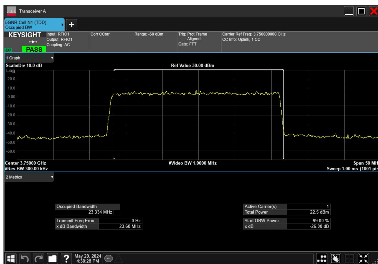
25MHz_15kHz_3750MHz_DFT-s-OFDM QPSK_RB128@0
