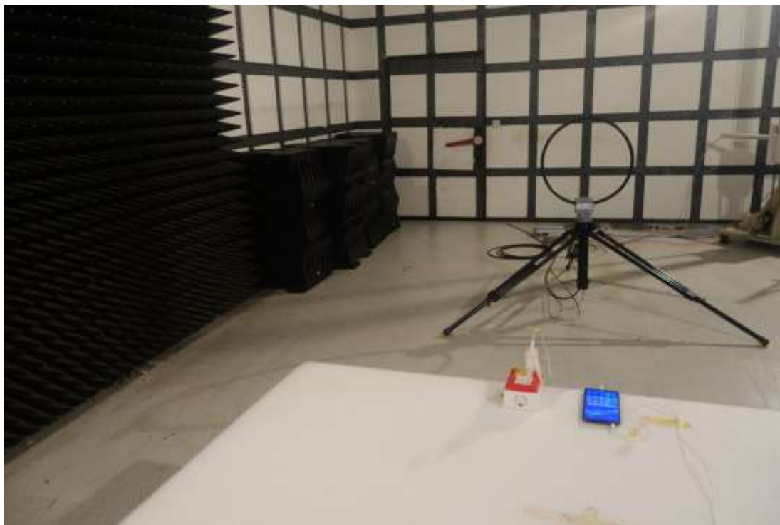
Radiated Spurious Emission (9K-30MHz)
