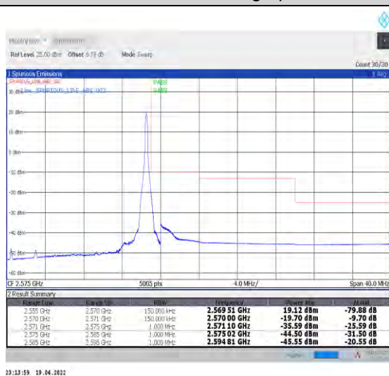
1-N7--15-15-H-5-CP-QPSK-Edge_1RB_Right-1@78-A nt0-PASS-see graph
