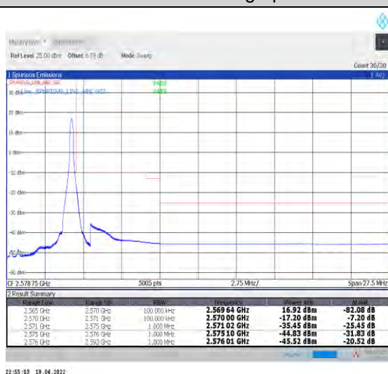
1-N7--15-5-H-5-CP-QPSK-Edge_1RB_Right-1@24-Ant 0-PASS-see graph
