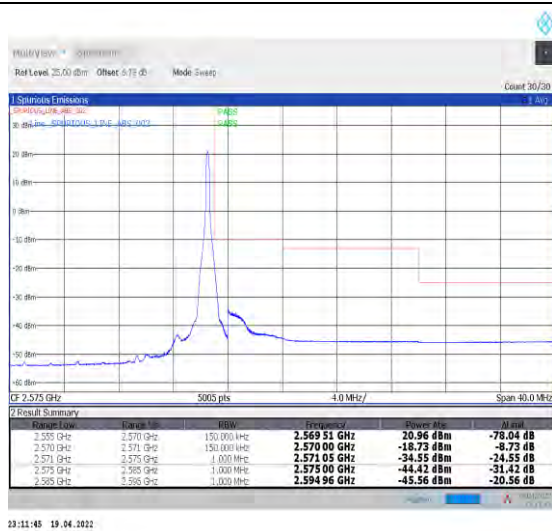
1-N7--15-15-H-2-DFT-PI2BPSK-Edge_1RB_Right-1@7 8-Ant0-PASS-see graph
