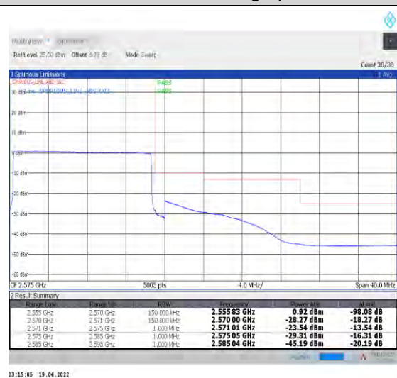
1-N7--15-15-H-6-CP-QPSK-Outer_Full-79@0-Ant 0-PASS-see graph
