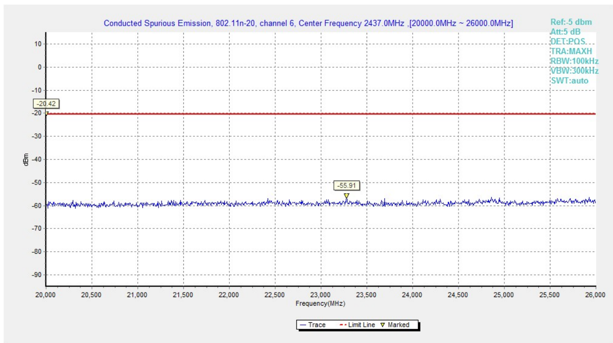
Fig. 79 Conducted Spurious Emission (802.11n-HT20, Ch6, 20 GHz-26 GHz)
