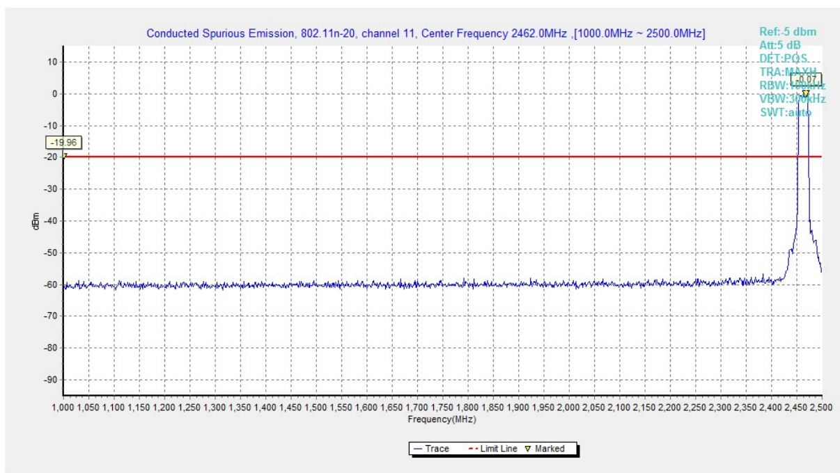
Fig. 82 Conducted Spurious Emission (802.11n-HT20, Ch11, 1 GHz-2.5 GHz)
