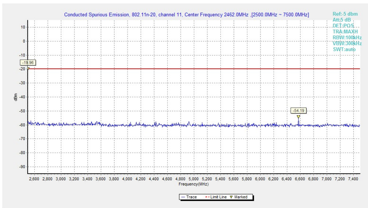
Fig. 83 Conducted Spurious Emission (802.11n-HT20, Ch11, 2.5 GHz-7.5 GHz)
