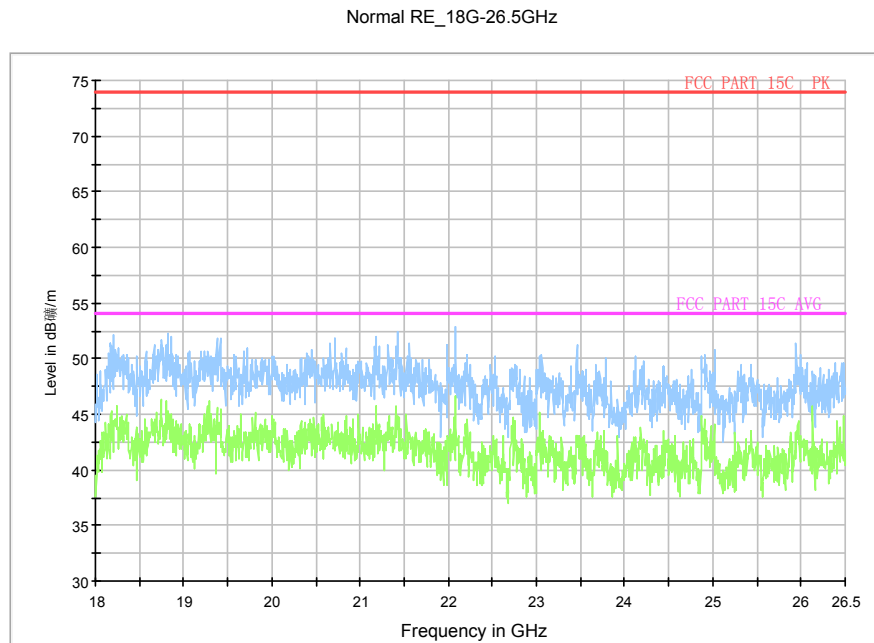
Fig. 130 Radiated emission: 18 GHz – 26.5 GHz
