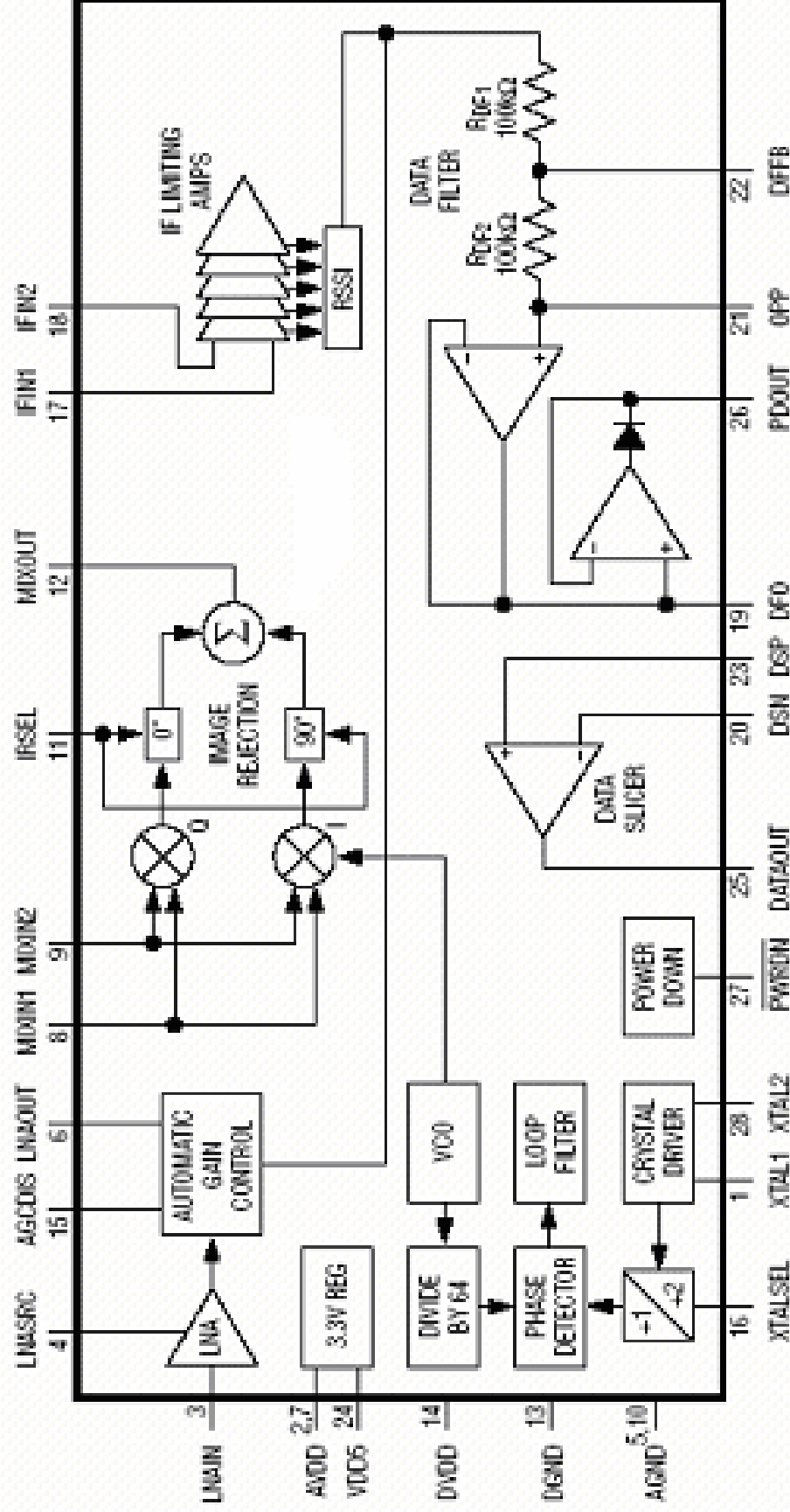
Superhetrodyne Receiver IC Internal Block Diagram
