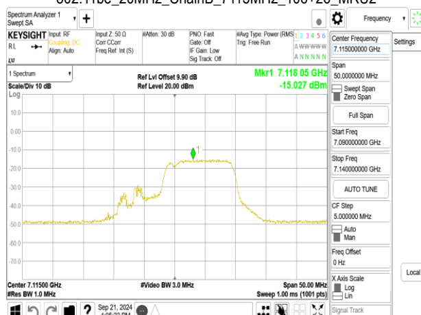
802.11be_20MHz_ChainB_7115MHz_106+26_MR2
