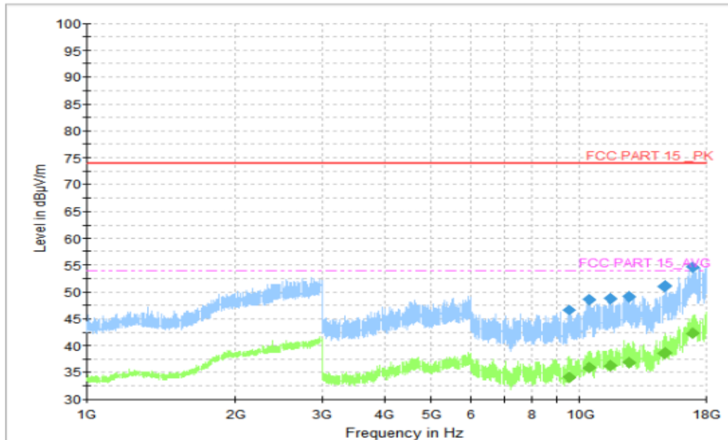
Figure A.1.12. Radiated Emission (Data Transfer: TF Card TO PC, 1GHz to 18GHz) Final_Results_PK
