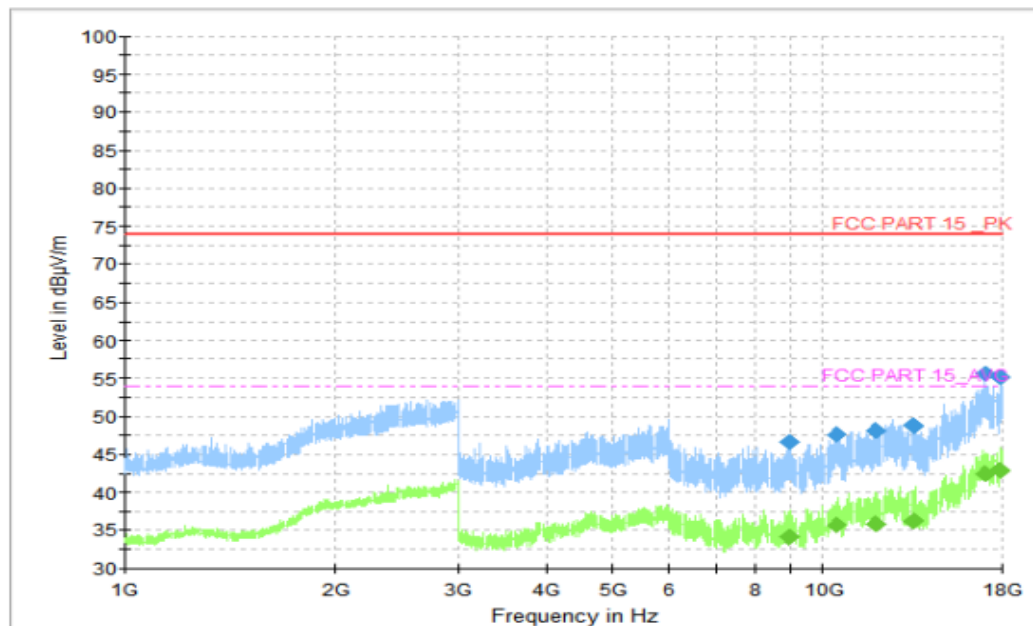
Figure A.1.8. Radiated Emission (Data Transfer: PC TO TF Card, 1GHz to 18GHz) Final_Results_PK
