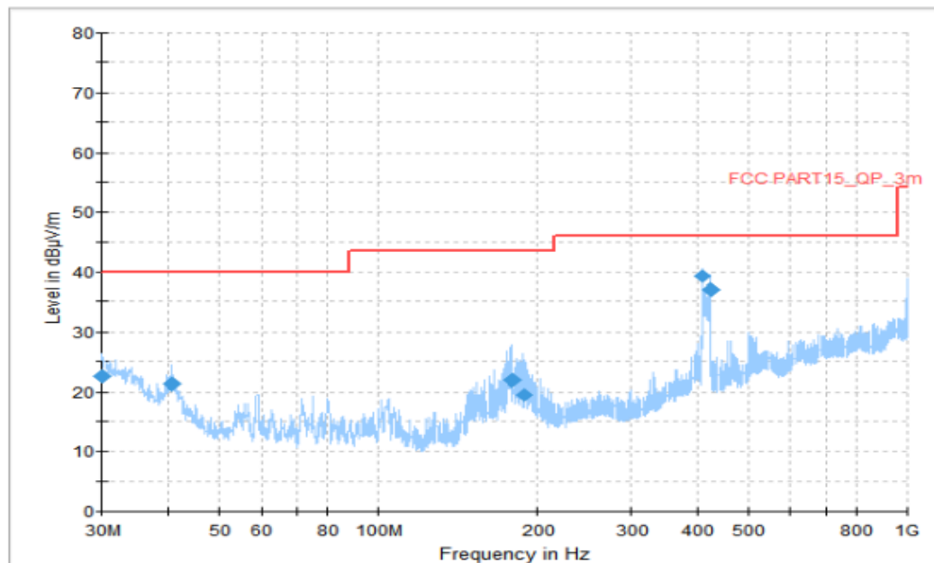
Figure A.1.11. Radiated Emission (Data Transfer: TF Card TO PC, 30MHz to 1GHz) Final_Results
