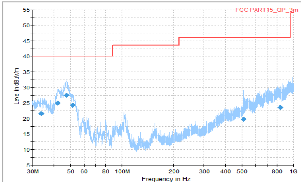
Figure A.1.5. Radiated Emission (GSM receiver 850MHz, 30MHz to 1GHz) Final_Results
