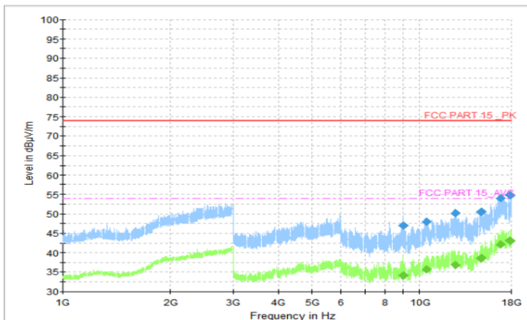
Figure A.1.10. Radiated Emission (Data Transfer: TF Card TO PC, 1GHz to 18GHz) Final_Results_PK
