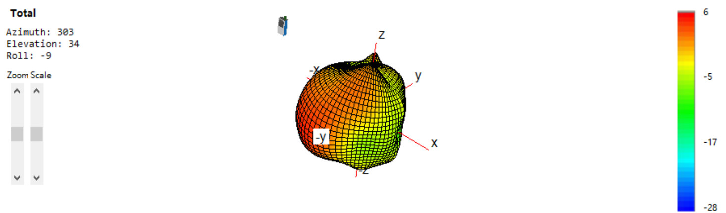
3D Antenna pattern
