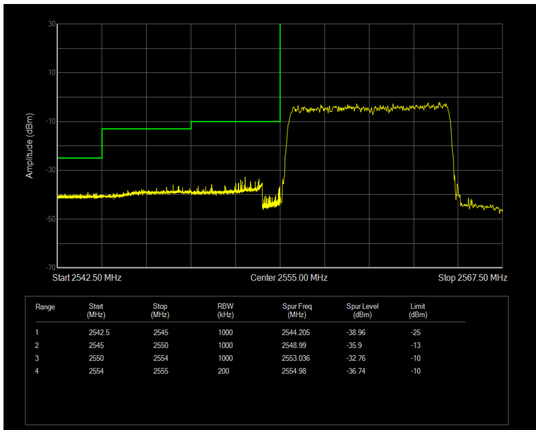
Band41 QPSK BW=10MHz Channel=40290 RB Size=1 Position=#Max
