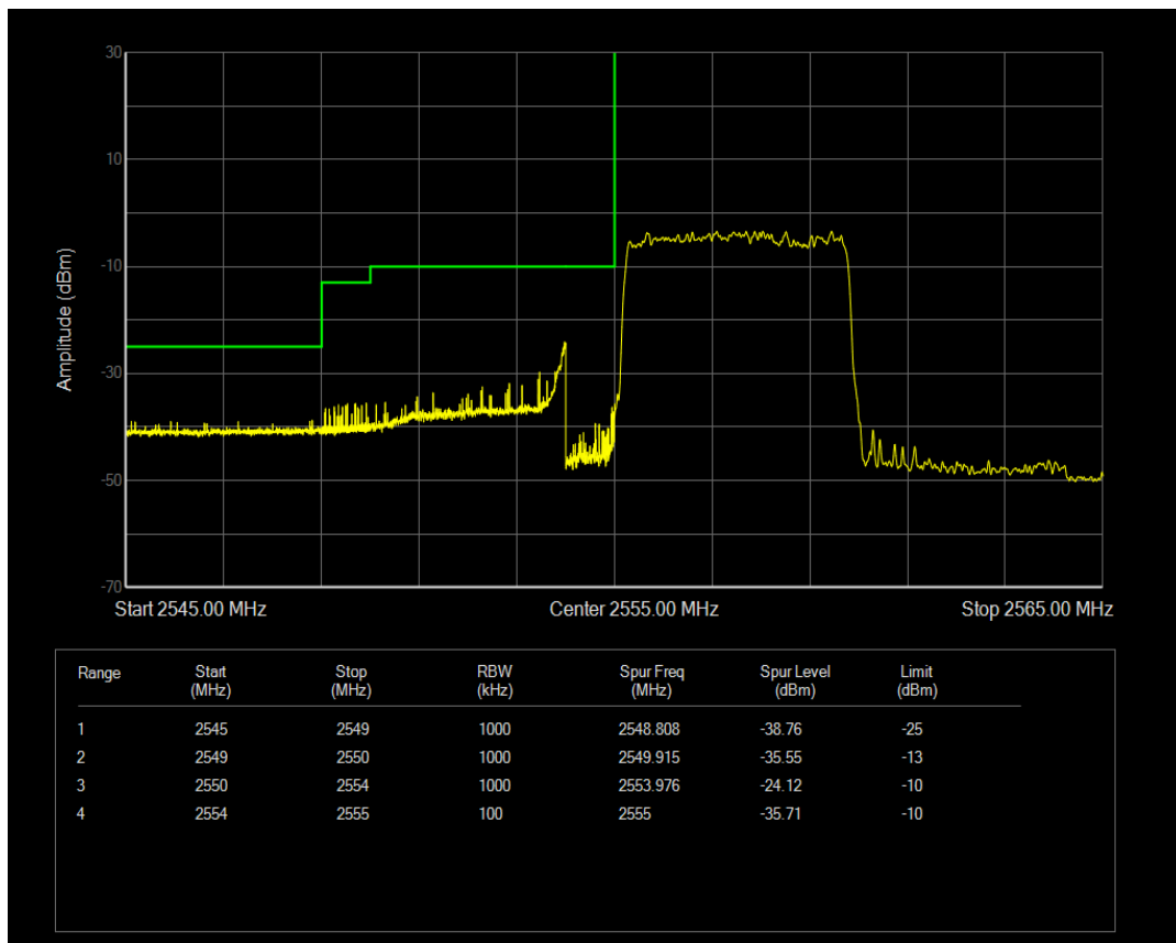
Band41 QAM16 BW=5MHz Channel=40265 RB Size=1 Position=#Max
