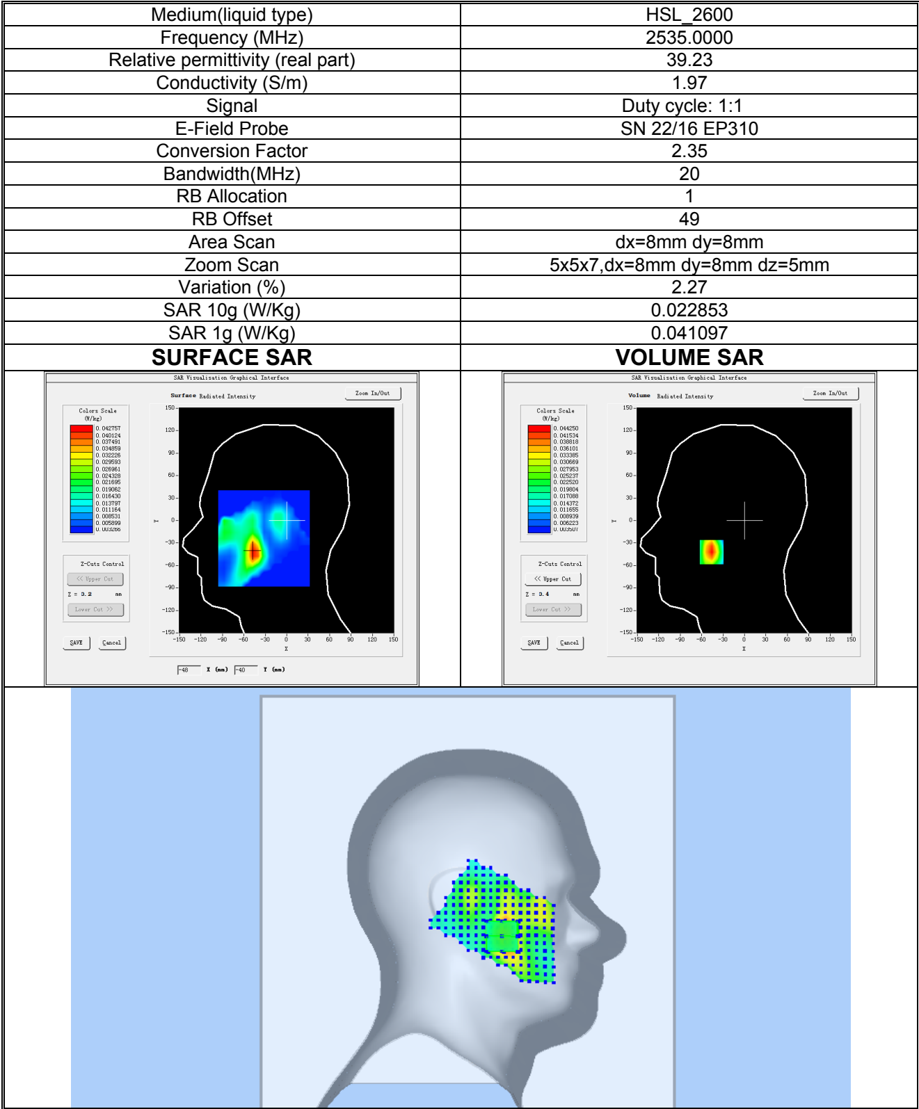
Plot 11:LTE BAND 7, Mid channel (Left Head Cheek) Product Description: Smartphone Test Date: 2021-06-04
