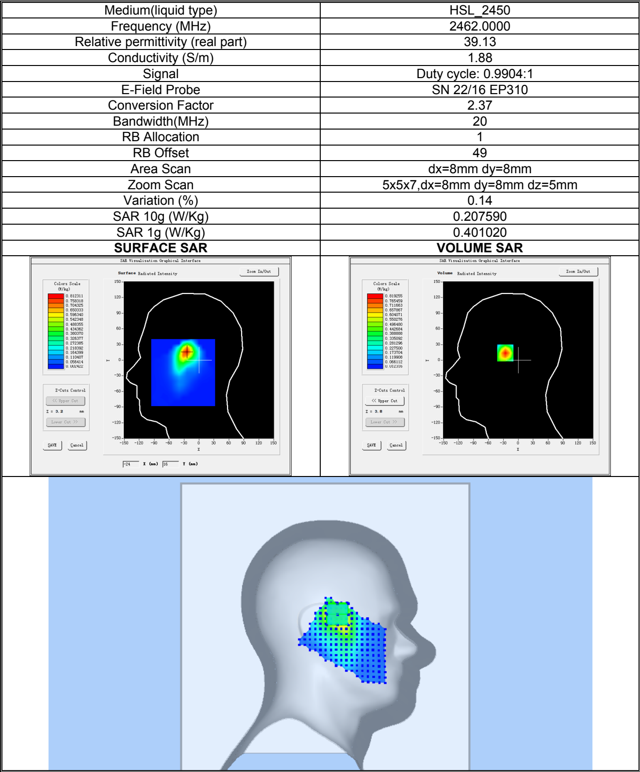
Plot 13:802.11b, High channel (Left Head Cheek) Product Description: Smartphone Test Date: 2021-05-20
