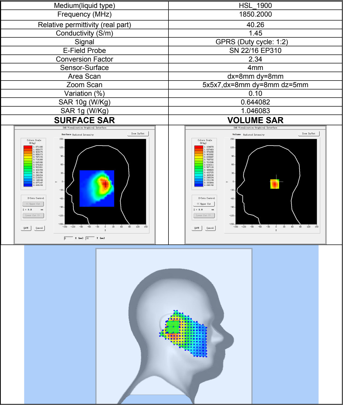
Plot 3: GPRS1900, Low channel (Left Head Cheek) Product Description: Smartphone Test Date: 2021-05-14
