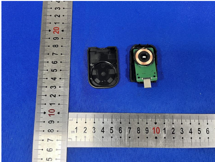
Coil Antenna-Watch
