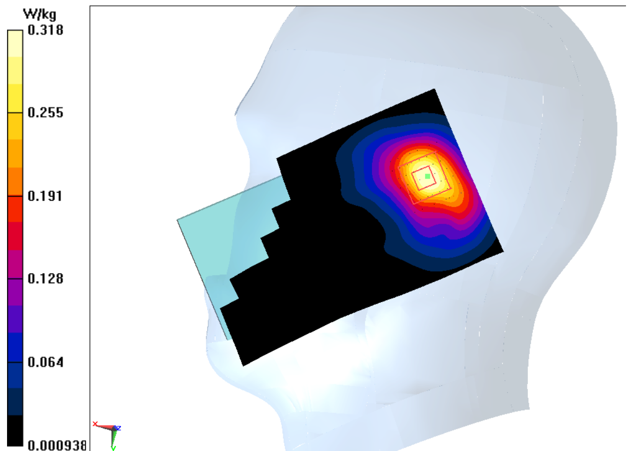
Fig.15 2450 MHz
