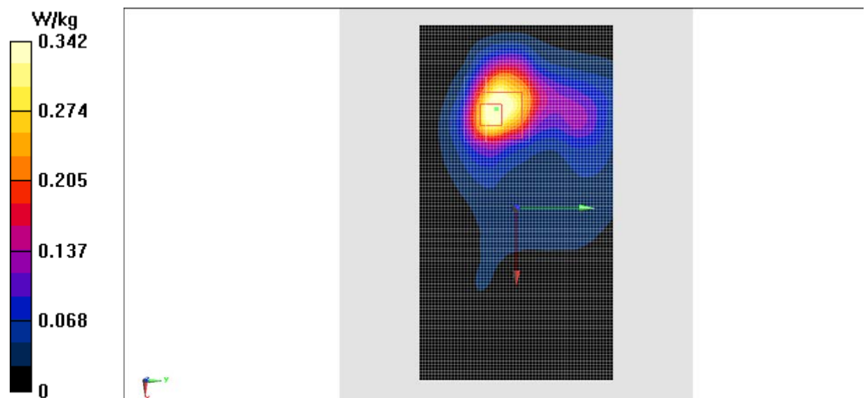
Fig.16 2450 MHz
