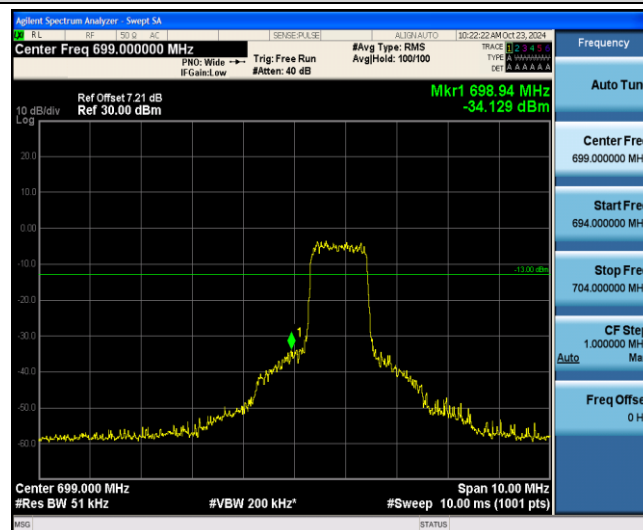
Band12-3MHz-QPSK-23025-6-0-Low--34.13-PASS
