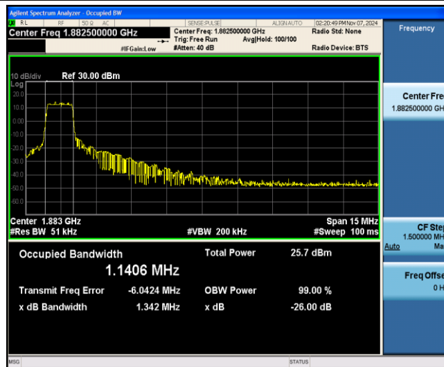
Band25-15MHz-QPSK-26365-6-0-Low-1.1406-1.342-PASS
