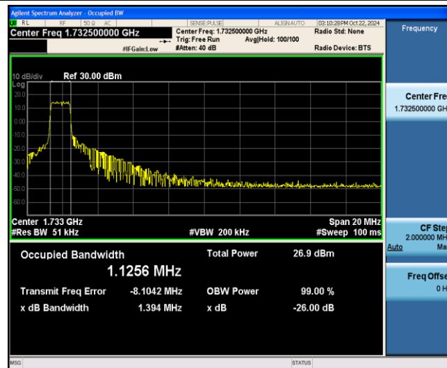
Band4-20MHz-QPSK-20175-6-0-Low-1.1256-1.394-PASS
