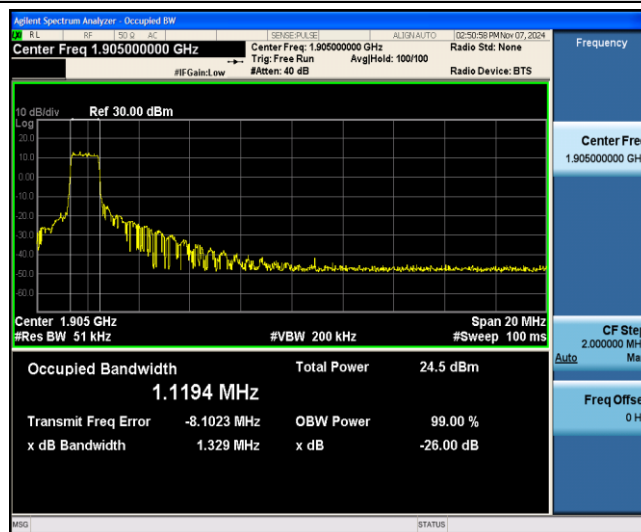
Band25-20MHz-16QAM-26590-6-0-Low-1.1194-1.329-PASS
