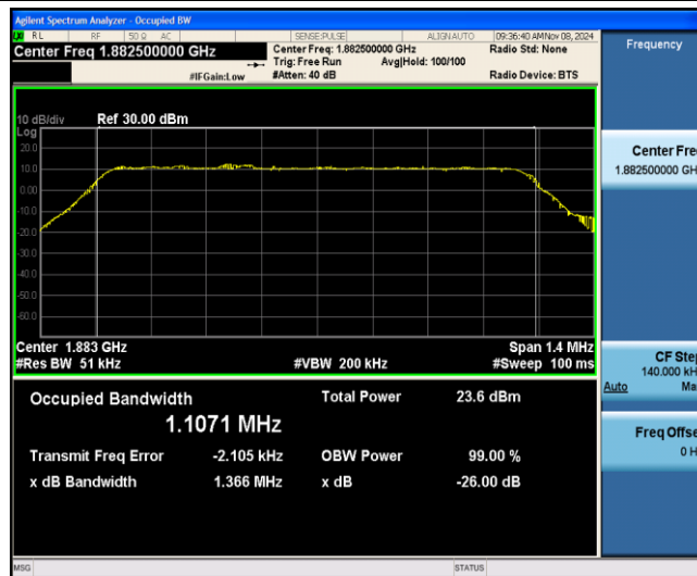
Band25-1.4MHz-QPSK-26365-6-0-Low-1.1071-1.366-PASS
