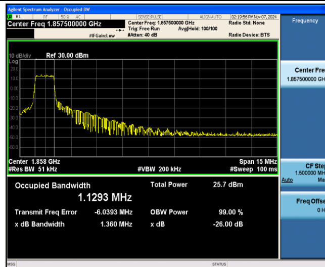
Band25-15MHz-QPSK-26115-6-0-Low-1.1293-1.360-PASS
