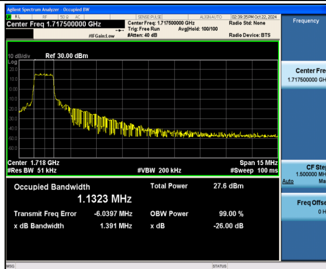
Band4-15MHz-16QAM-20025-6-0-Low-1.1323-1.391-PASS
