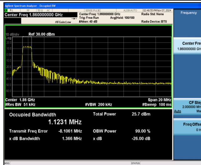
Band25-20MHz-16QAM-26140-6-0-Low-1.1231-1.366-PASS
