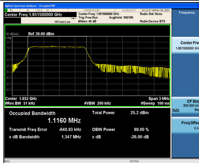
Band25-3MHz-16QAM-26055-6-0-Low-1.1160-1.347-PASS
