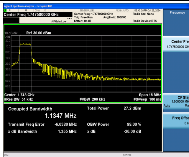
Band4-15MHz-16QAM-20325-6-0-Low-1.1347-1.355-PASS
