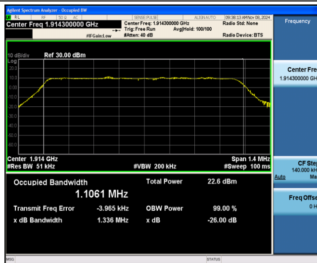
Band25-1.4MHz-QPSK-26683-6-0-Low-1.1061-1.336-PASS
