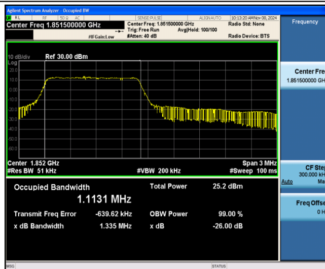
Band25-3MHz-QPSK-26055-6-0-Low-1.1131-1.335-PASS
