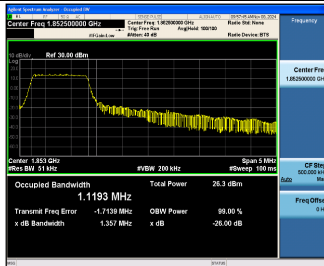
Band25-5MHz-QPSK-26065-6-0-Low-1.1193-1.357-PASS
