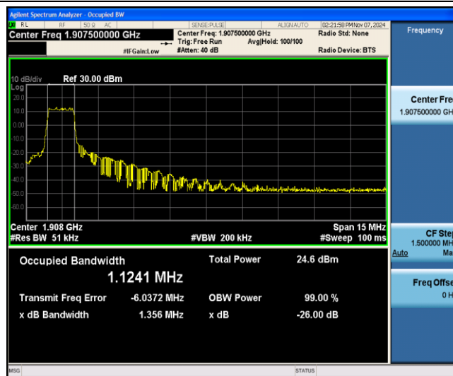
Band25-15MHz-16QAM-26615-6-0-Low-1.1241-1.356-PASS
