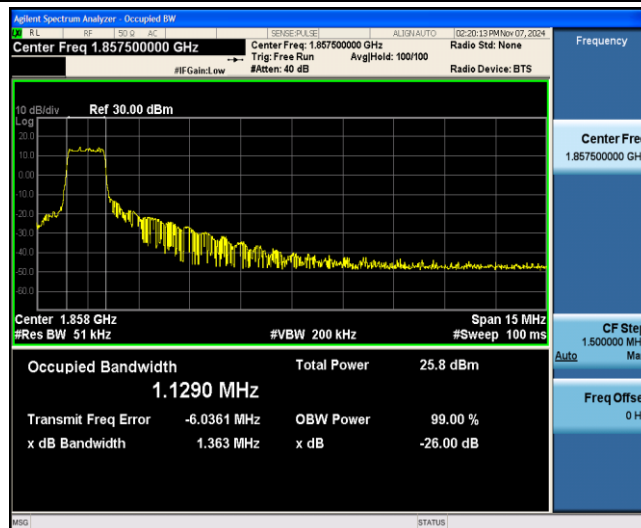
Band25-15MHz-16QAM-26115-6-0-Low-1.1290-1.363-PASS
