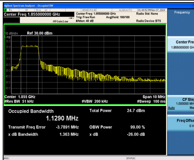
Band25-10MHz-QPSK-26090-6-0-Low-1.1290-1.363-PASS
