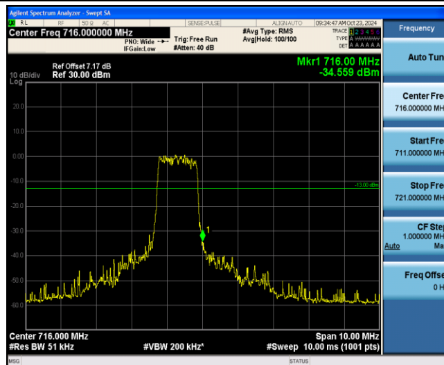
Band12-1.4MHz-QPSK-23173-6-0-High--34.56-PASS
