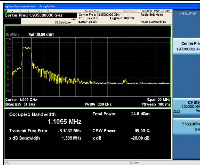
Band25-20MHz-QPSK-26590-6-0-Low-1.1055-1.385-PASS
