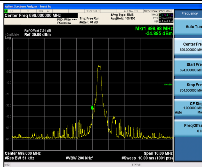
Band12-3MHz-QPSK-23025-1-0-Low--34.90-PASS
