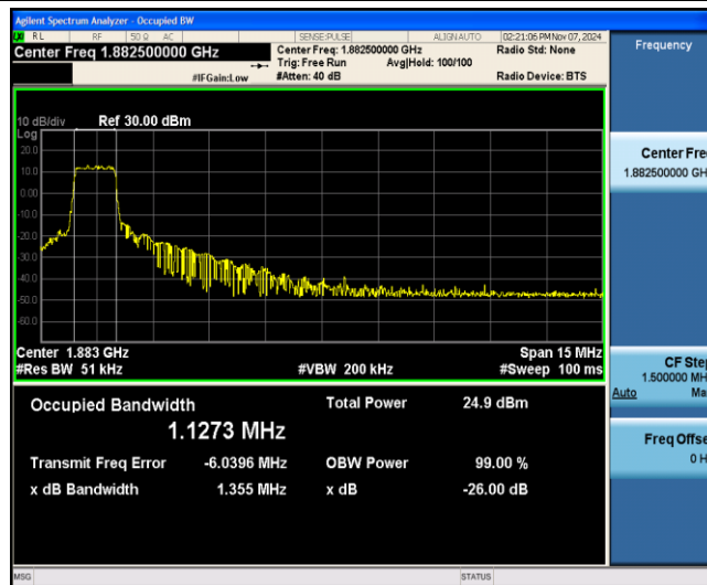
Band25-15MHz-16QAM-26365-6-0-Low-1.1273-1.355-PASS
