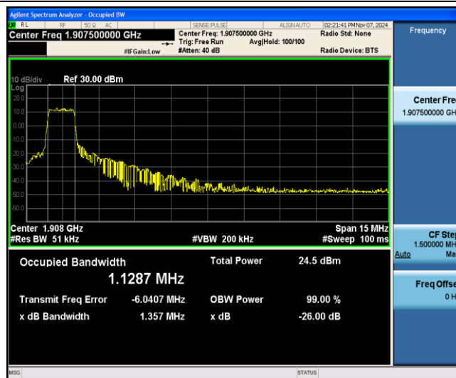
Band25-15MHz-QPSK-26615-6-0-Low-1.1287-1.357-PASS
