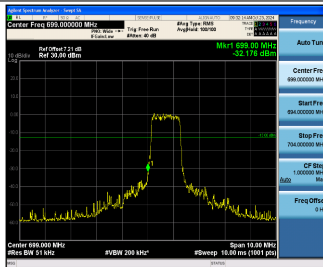
Band12-1.4MHz-16QAM-23017-6-0-Low--32.18-PASS
