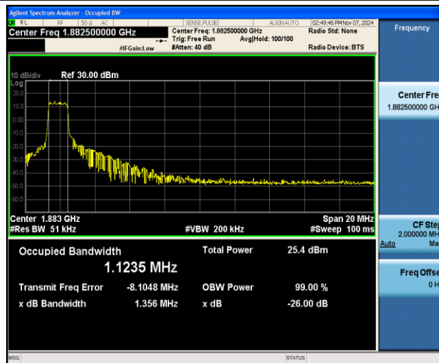
Band25-20MHz-16QAM-26365-6-0-Low-1.1235-1.356-PASS
