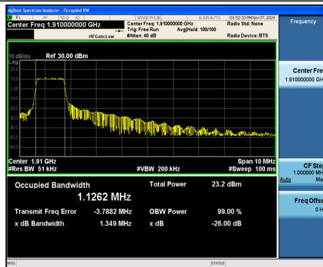
Band25-10MHz-QPSK-26640-6-0-Low-1.1262-1.349-PASS
