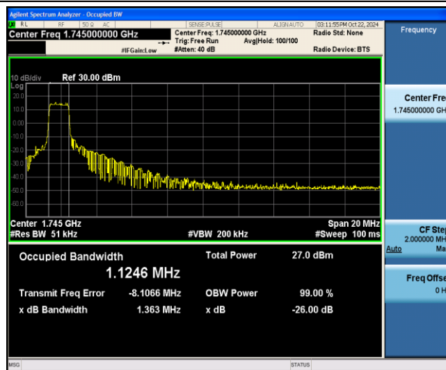
Band4-20MHz-16QAM-20300-6-0-Low-1.1246-1.363-PASS
