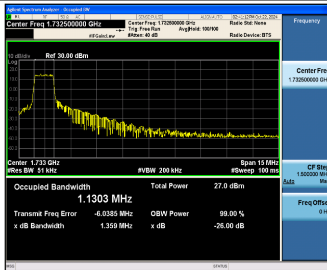
Band4-15MHz-QPSK-20175-6-0-Low-1.1303-1.359-PASS
