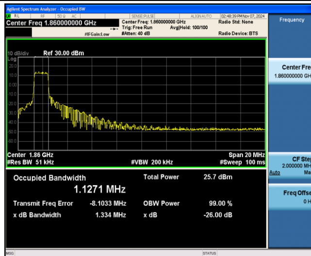
Band25-20MHz-QPSK-26140-6-0-Low-1.1271-1.334-PASS
