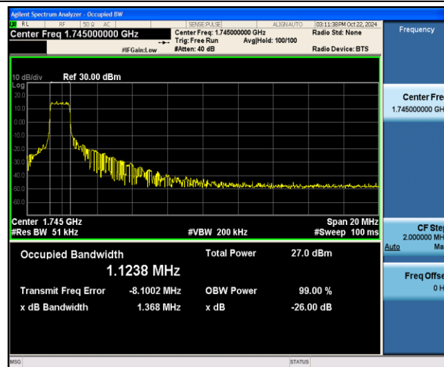
Band4-20MHz-QPSK-20300-6-0-Low-1.1238-1.368-PASS
