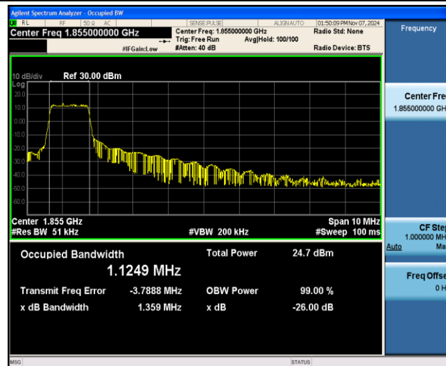
Band25-10MHz-16QAM-26090-6-0-Low-1.1249-1.359-PASS
