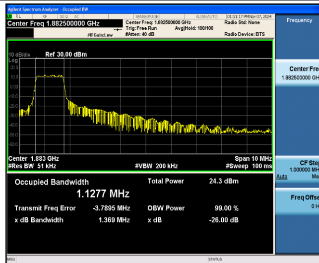
Band25-10MHz-16QAM-26365-6-0-Low-1.1277-1.369-PASS
