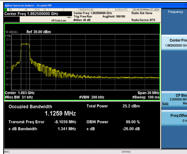
Band25-20MHz-QPSK-26365-6-0-Low-1.1259-1.341-PASS
