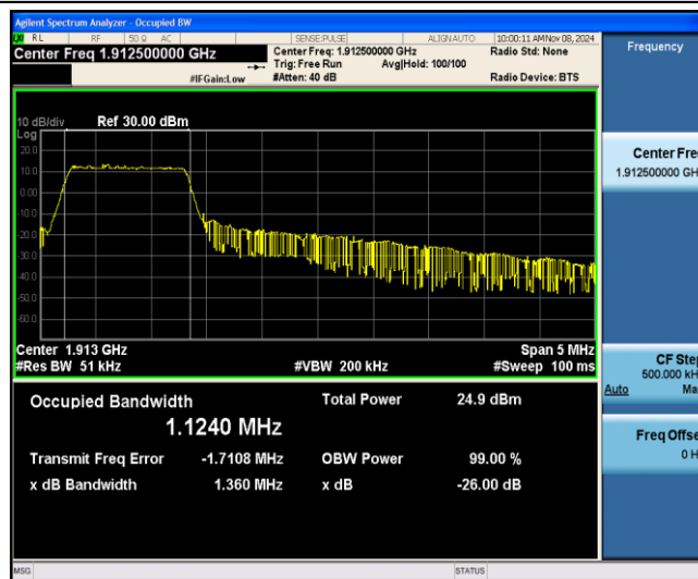
Band25-5MHz-16QAM-26665-6-0-Low-1.1240-1.360-PASS
