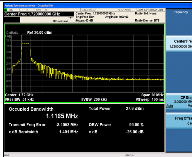
Band4-20MHz-16QAM-20050-6-0-Low-1.1165-1.401-PASS
