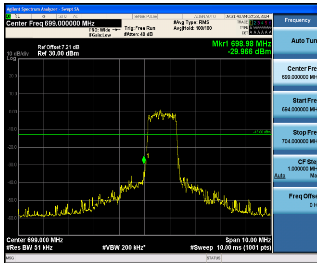
Band12-1.4MHz-QPSK-23017-6-0-Low--29.97-PASS
