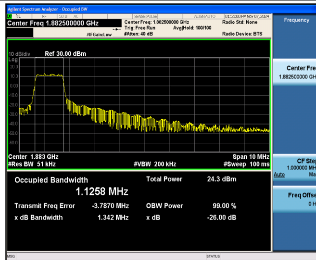
Band25-10MHz-QPSK-26365-6-0-Low-1.1258-1.342-PASS
