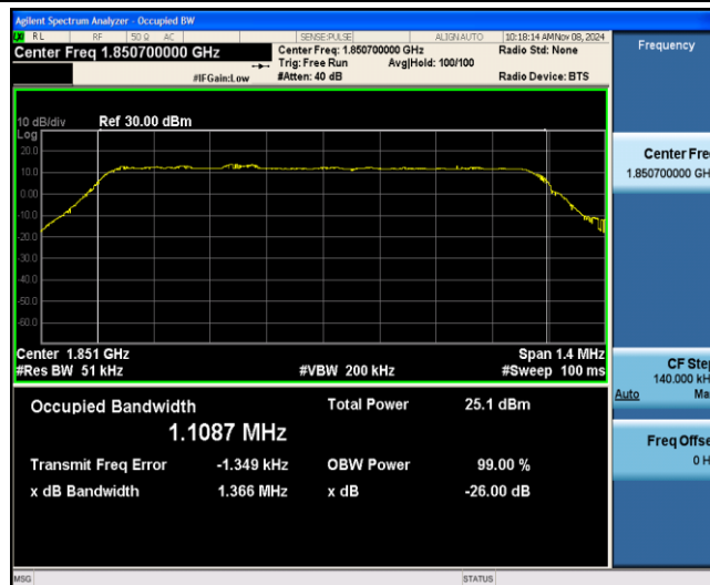
Band25-1.4MHz-16QAM-26047-6-0-Low-1.1087-1.366-PASS
