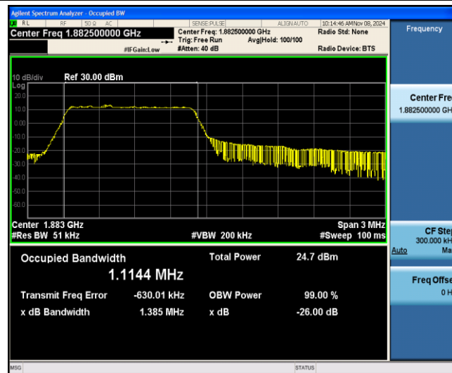
Band25-3MHz-16QAM-26365-6-0-Low-1.1144-1.385-PASS
