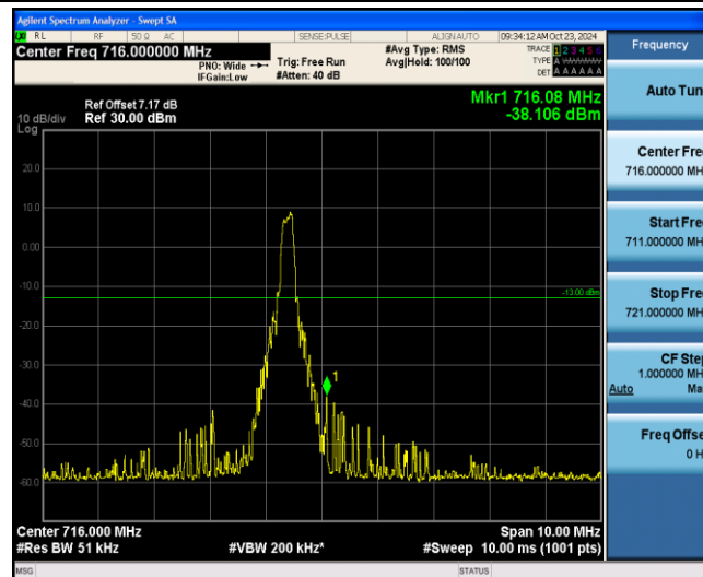
Band12-1.4MHz-16QAM-23173-1-5-High--38.11-PASS
