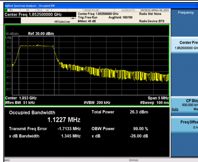
Band25-5MHz-16QAM-26065-6-0-Low-1.1227-1.345-PASS
