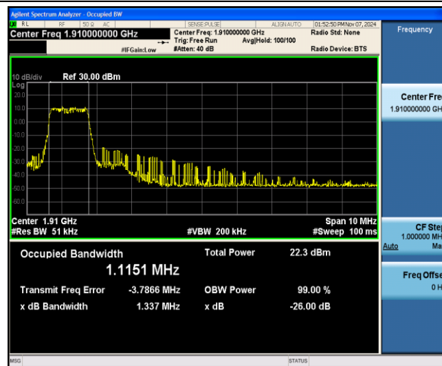
Band25-10MHz-16QAM-26640-6-0-Low-1.1151-1.337-PASS
