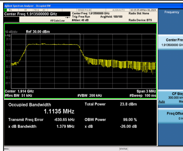
Band25-3MHz-QPSK-26675-6-0-Low-1.1135-1.379-PASS
