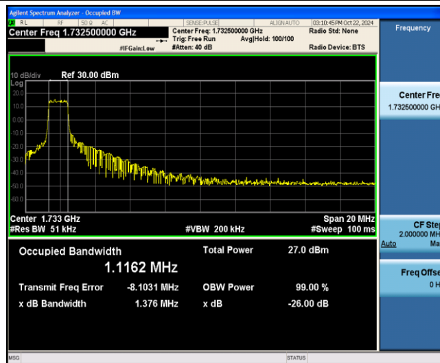
Band4-20MHz-16QAM-20175-6-0-Low-1.1162-1.376-PASS
