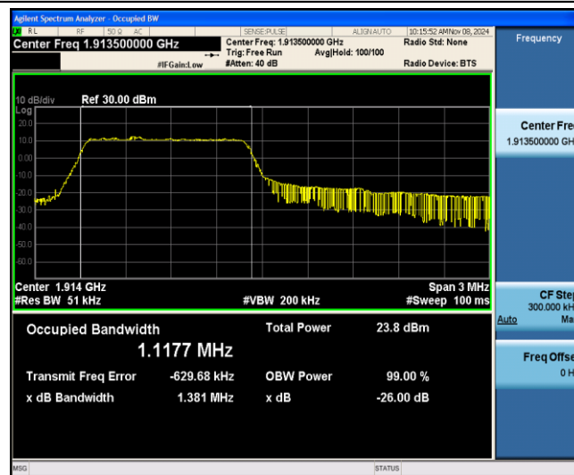
Band25-3MHz-16QAM-26675-6-0-Low-1.1177-1.381-PASS
