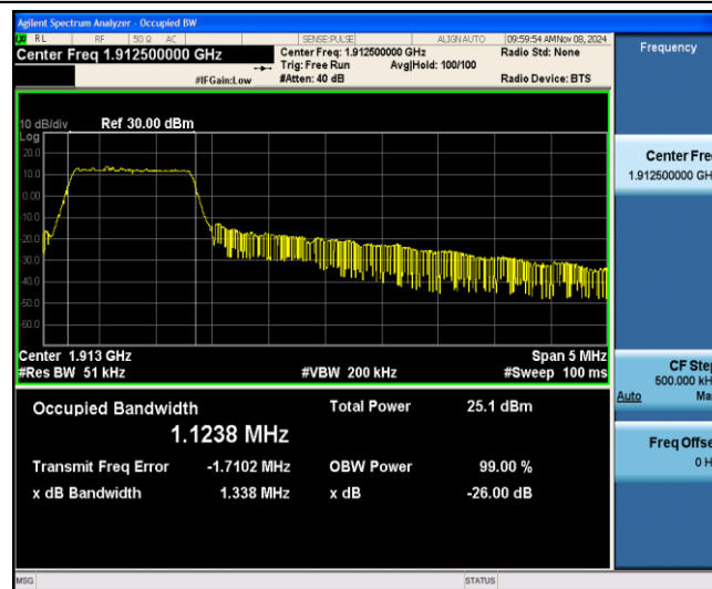
Band25-5MHz-QPSK-26665-6-0-Low-1.1238-1.338-PASS
