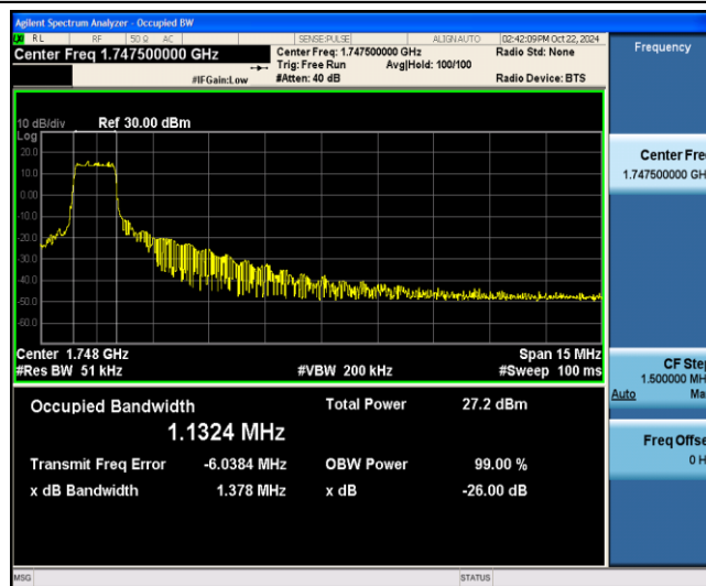
Band4-15MHz-QPSK-20325-6-0-Low-1.1324-1.378-PASS
