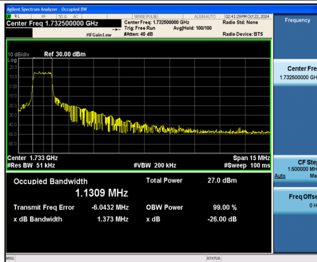
Band4-15MHz-16QAM-20175-6-0-Low-1.1309-1.373-PASS
