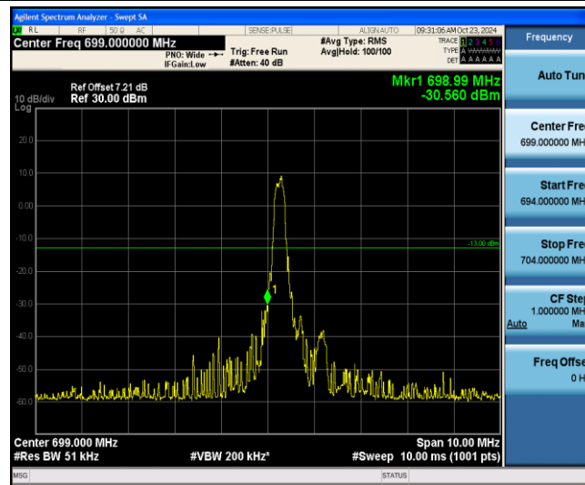
Band12-1.4MHz-16QAM-23017-1-0-Low--30.56-PASS
