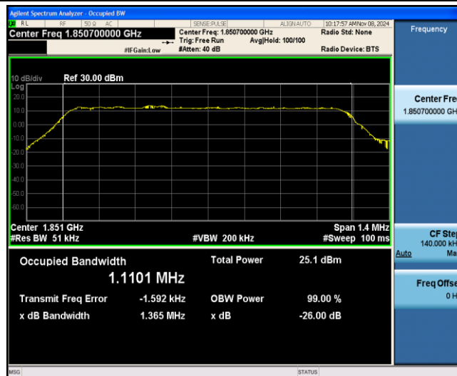
Band25-1.4MHz-QPSK-26047-6-0-Low-1.1101-1.365-PASS
