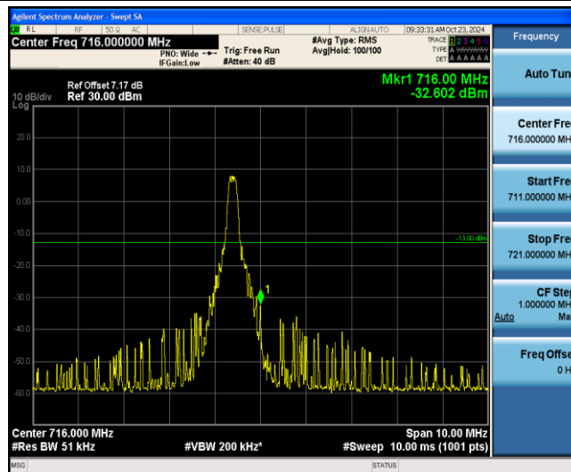
Band12-1.4MHz-QPSK-23173-1-5-High--32.60-PASS
