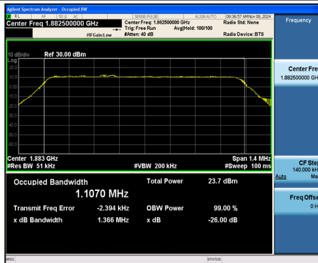
Band25-1.4MHz-16QAM-26365-6-0-Low-1.1070-1.366-PASS
