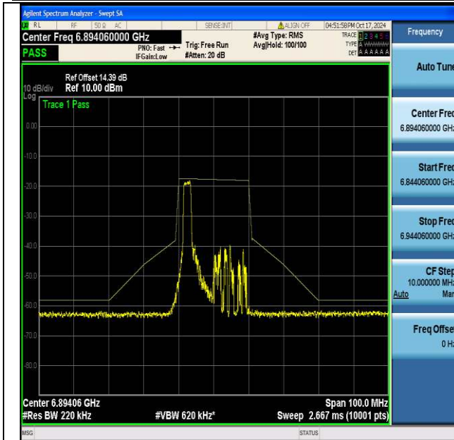
NTNV-11be20MIMO-Ant1-6895-26Tone-RU0-PASS
