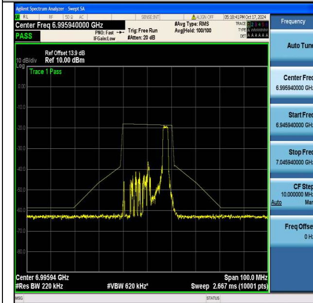
NTVN-11be20MIMO-Ant1-6995-26Tone-RU8-PASS
