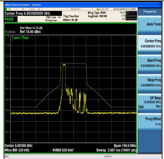
NTNV-11be20MIMO-Ant2-6895-26Tone-RU0-PASS
