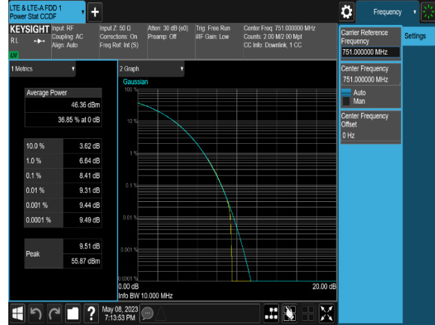
Plot 8-272. Peak To Average Power Ratio Plot (LTE B13_1C_10M_256QAM - Mid Channel_4T, Port 0)
