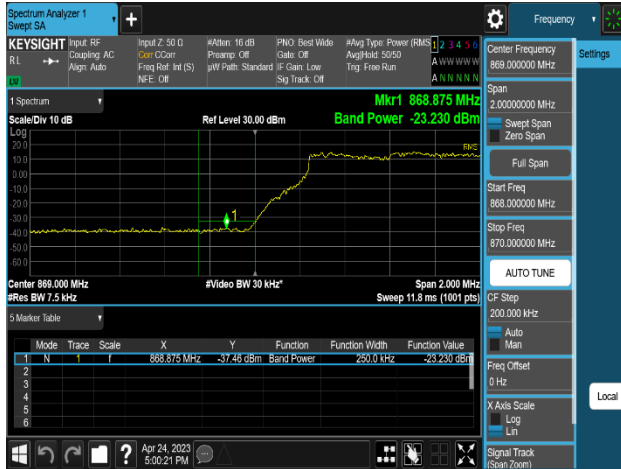
Plot 8-283. Band Edge Emission Summary Data Plot (LTE B5 3C 5M+10M+10M 16QAM - Low Channel 2T, Port 1)
