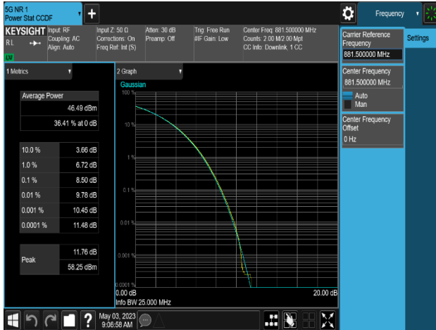
Plot 8-267. Peak To Average Power Ratio Plot (MSR 3C_DSS B(n)5_1C_10M+NR n5_1C_10M+LTE B5_1C_5M_QPSK - Mid Channel_4T, Port 0)
