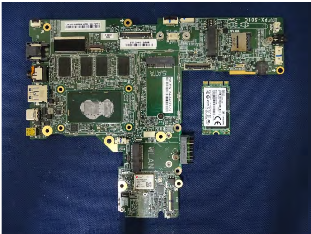
(68) EUT Photo
