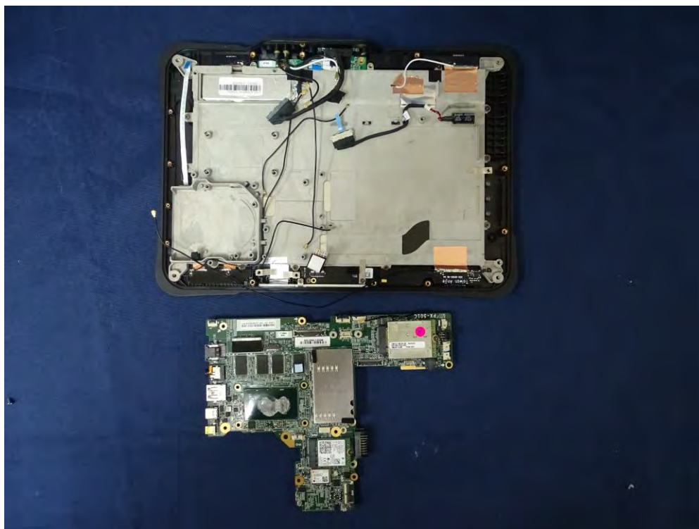
(55) EUT Photo
