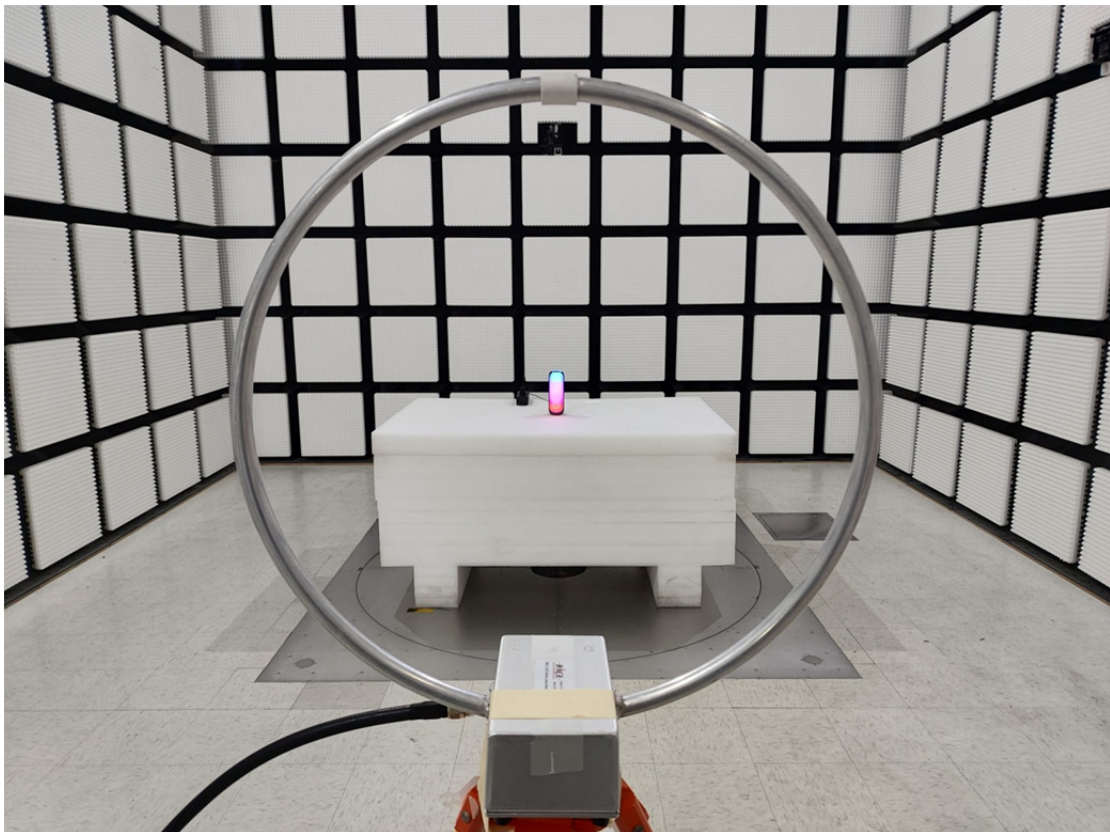
Radiated Emission 9k-30MHz Parallel View
