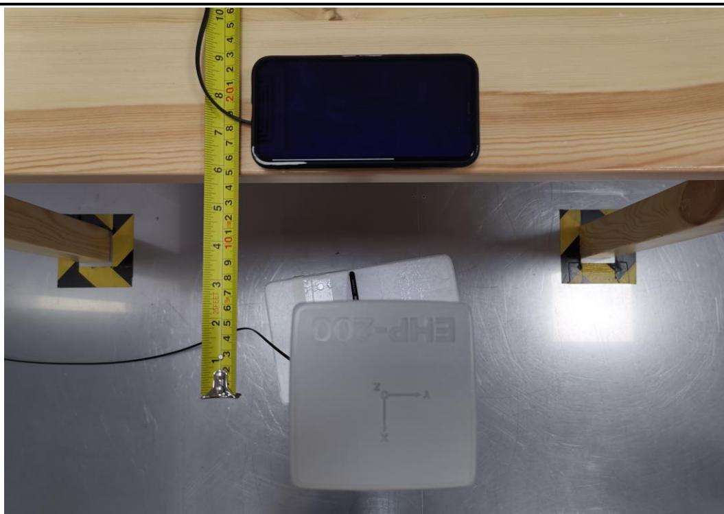
Test setup of C side
