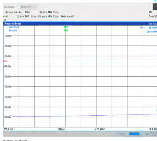
1-N66-PC3-15-40-H-1-DFT-PI2BPSK-Inner_1RB_Lef t-1@1-0.15-30-Ant1--86.92--33-PASS
