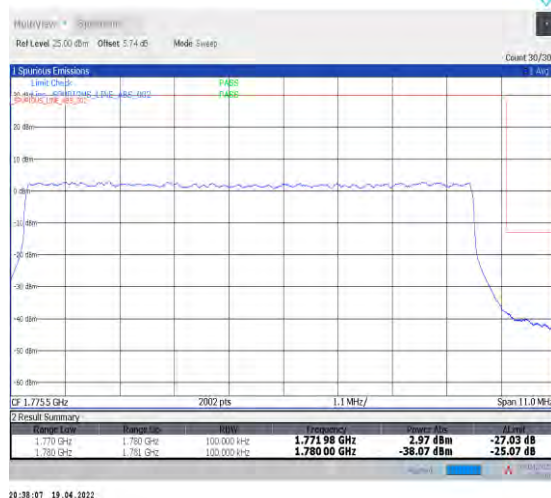
1-N66-PC3-15-10-H-3-DFT-PI2BPSK-Outer_Full-50@0-Ant1-seegraph-PASS-see graph
