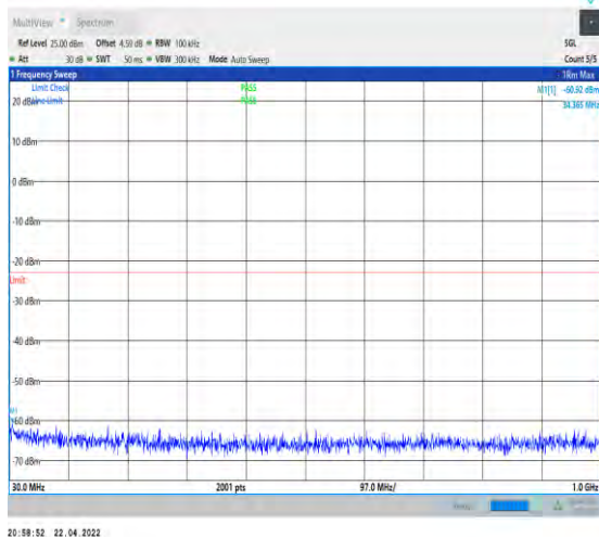
1-N66-PC3-15-40-L-1-DFT-PI2BPSK-Inner_1RB_Le ft-1@1-30-1000-Ant1--60.92--23-PASS
