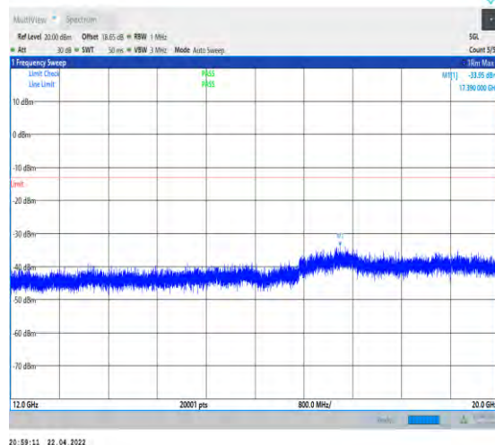
1-N66-PC3-15-40-L-1-DFT-PI2BPSK-Inner_1RB_Lef t-1@1-12000-20000-Ant1--33.95--13-PASS
