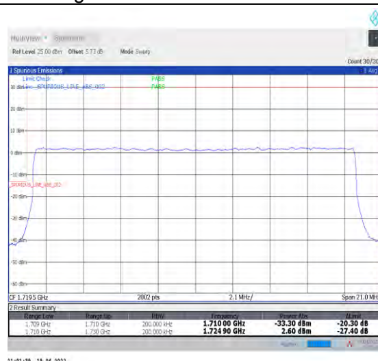
1-N66-PC3-15-20-L-3-DFT-PI2BPSK-Outer_Full-100@0-Ant1-seegraph-PASS-see graph
