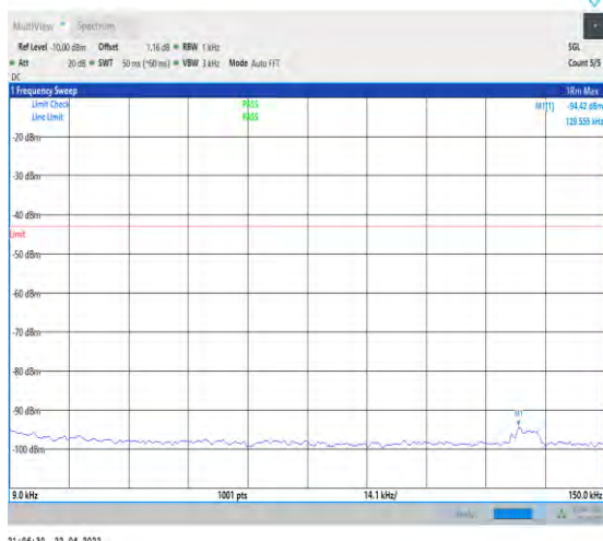
1-N66-PC3-15-40-H-1-DFT-PI2BPSK-Inner_1RB_Le ft-1@1-0.009-0.15-Ant1--94.42--43-PASS
