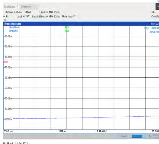
1-N66-PC3-15-40-L-1-DFT-PI2BPSK-Inner_1RB_Lef t-1@1-0.15-30-Ant1--86.88--33-PASS
