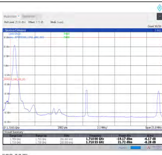
1-N66-PC3-15-20-L-1-DFT-PI2BPSK-Edge_1RB_Left-1@0-Ant1-seegraph-PASS-see graph
