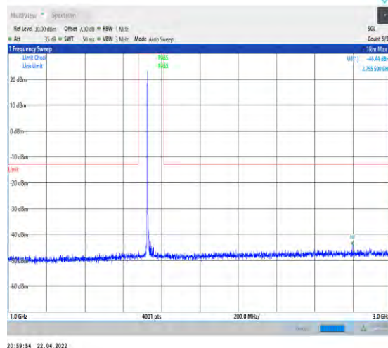
1-N66-PC3-15-40-M-1-DFT-PI2BPSK-Inner_1RB_Le ft-1@1-1000-3000-Ant1--44.44--13-PASS
