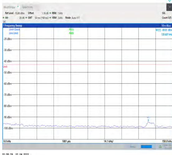
1-N66-PC3-15-40-L-1-DFT-PI2BPSK-Inner_1RB_Le ft-1@1-0.009-0.15-Ant1--93.81--43-PASS
