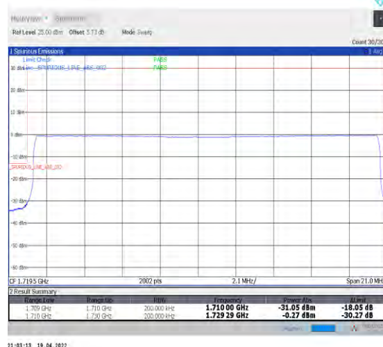
1-N66-PC3-15-20-L-6-CP-QPSK-Outer_Full-106@0-Ant1-seegraph-PASS-see graph
