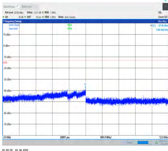
1-N66-PC3-15-40-L-1-DFT-PI2BPSK-Inner_1RB_Le ft-1@1-3000-12000-Ant1--37.90--13-PASS
