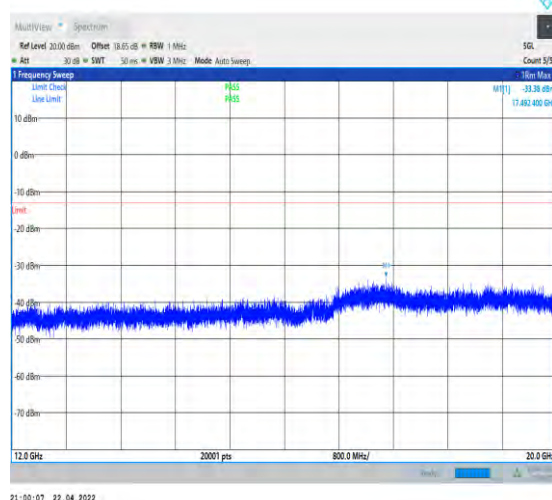
1-N66-PC3-15-40-M-1-DFT-PI2BPSK-Inner_1RB_Le ft-1@1-12000-20000-Ant1--33.38--13-PASS
