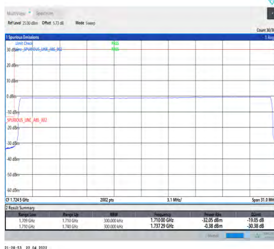
1-N66-PC3-15-30-L-6-CP-QPSK-Outer_Full-160@0-Ant1-seegraph-PASS-see graph
