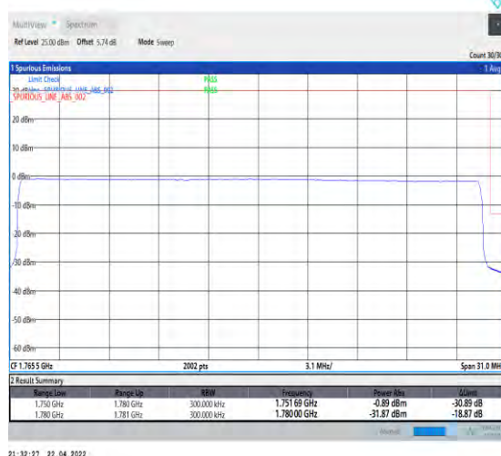
1-N66-PC3-15-30-H-6-CP-QPSK-Outer_Full-160@0-Ant1-seegraph-PASS-see graph
