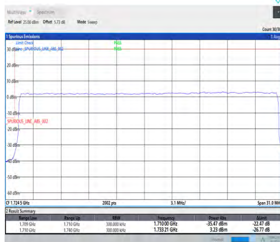
1-N66-PC3-15-30-L-3-DFT-PI2BPSK-Outer_Full-160@0-Ant1-seegraph-PASS-see graph
