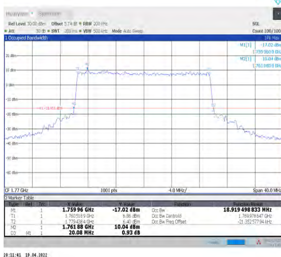
1-N66-PC3-15-20-H-8-CP-64QAM-Outer_Full-106@0-Ant1-18.919-20.080-≤20-PASS
