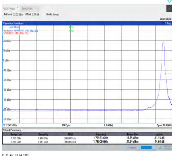
1-N66-PC3-15-30-H-5-CP-QPSK-Edge_1RB_Right-1@159-Ant1-seegraph-PASS-see graph
