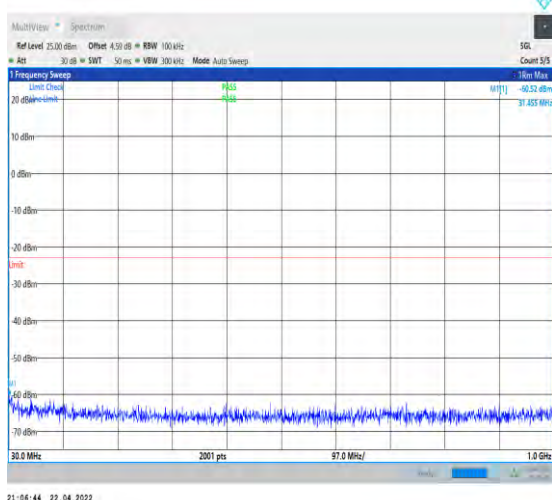
1-N66-PC3-15-40-H-1-DFT-PI2BPSK-Inner_1RB_Le ft-1@1-30-1000-Ant1--60.52--23-PASS
