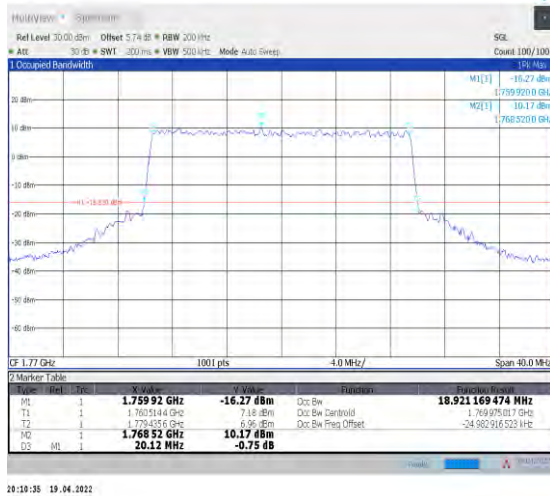
1-N66-PC3-15-20-H-6-CP-QPSK-Outer_Full-106@0 -Ant1-18.921-20.120-≤20-PASS
