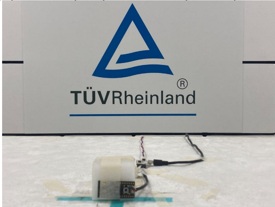
Photograph 7: Test Setup for Spurious Emissions (Close View)
