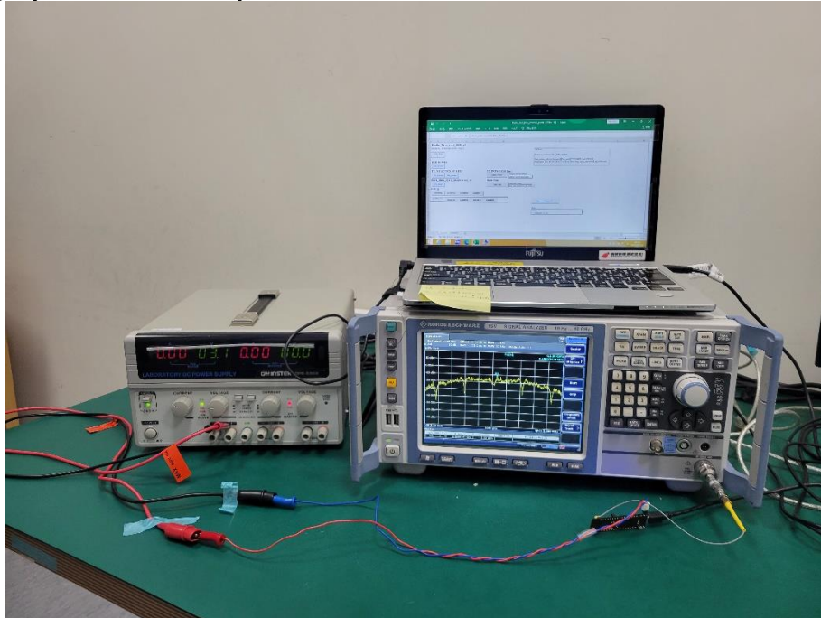
Photograph 10: Test Setup for Conducted
