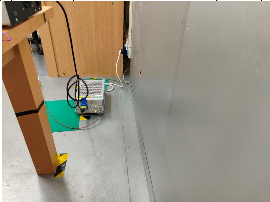
Photograph 9: Test Setup for Mains Conducted Emissions (Back View)
