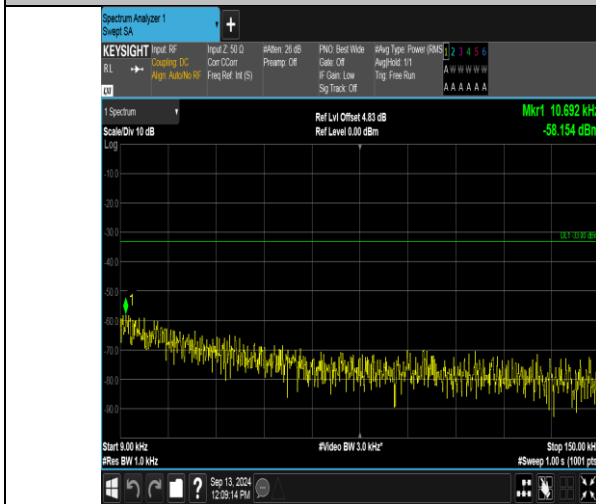
Band12_3MHz_QPSK_23165_1RB#14_0.009~0.15_0.009~0.15
