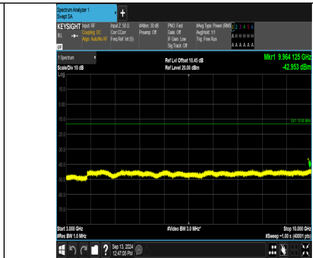
Band12_5MHz_16QAM_23095_1RB#0_3000~10000_3000~10000
