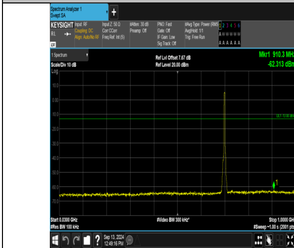
Band12_5MHz_QPSK_23095_25RB#0_30-1000_30-1000
