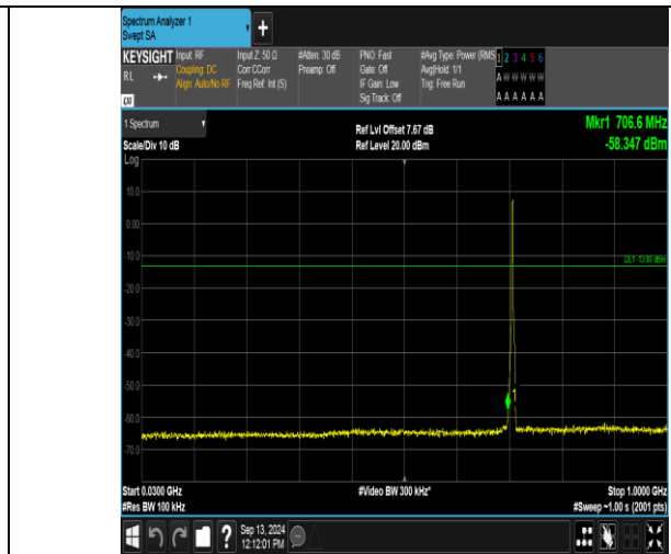
Band12_3MHz_16QAM_23165_15RB#0_30~1000_30~1000
