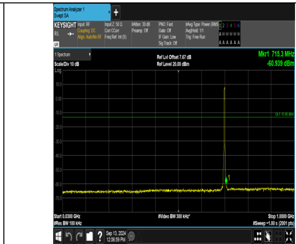
Band12_3MHz_16QAM_23095_15RB#0_30~1000_30~1000
