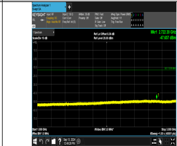
Band12_5MHz_QPSK_23095_25RB#0_1000-3000_1000-3000
