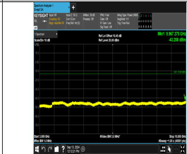
Band12_3MHz_16QAM_23165_15RB#0_3000~10000_3000~10000
