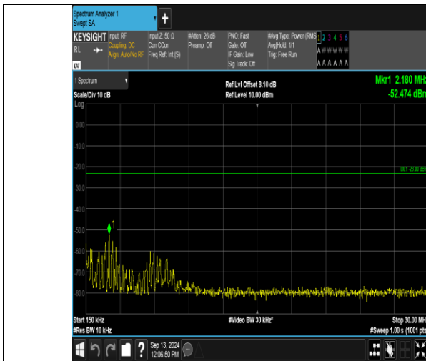
Band12_3MHz_16QAM_23095_15RB#0_0.15~30_0.15~30
