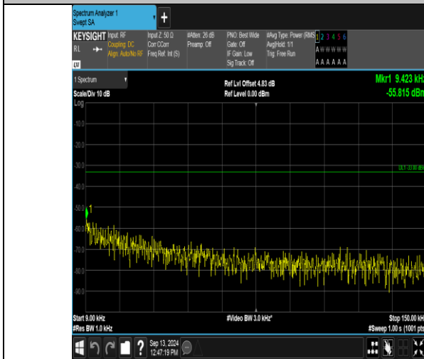
Band12_5MHz_QPSK_23095_1RB#24_0.009~0.15_0.009~0.15
