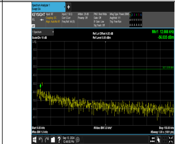
Band12_5MHz_16QAM_23095_25RB#0_0.009-0.15_0.009-0.15
