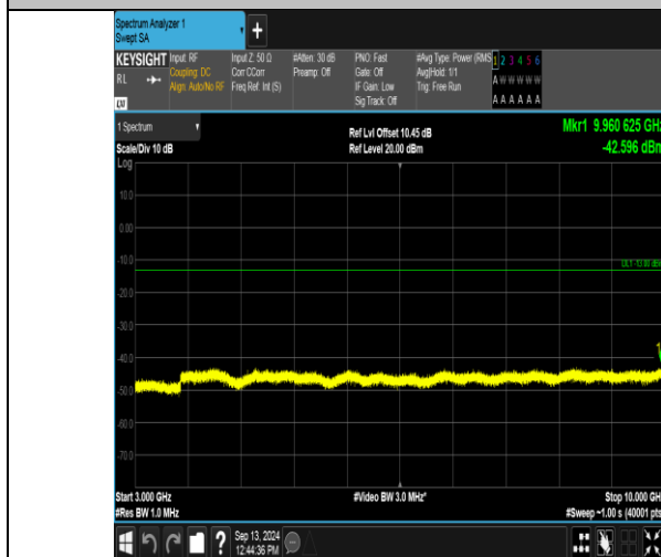
Band12_5MHz_QPSK_23035_25RB#0_3000-10000_3000-10000
