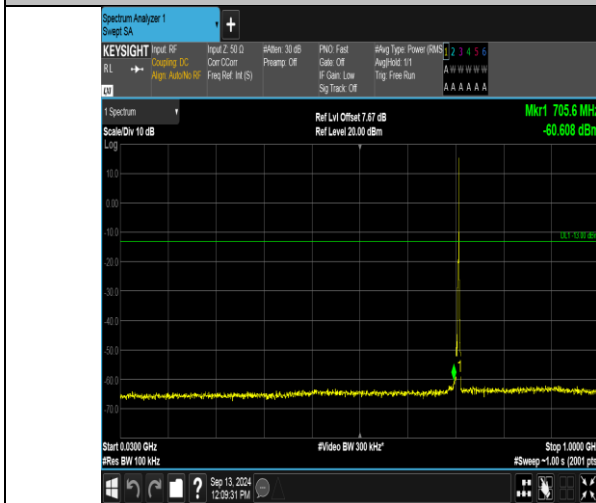
Band12_3MHz_QPSK_23165_1RB#14_30~1000_30~1000
