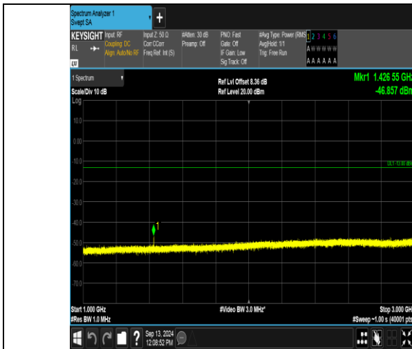
Band12_3MHz_16QAM_23165_1RB#0_1000~3000_1000~3000
