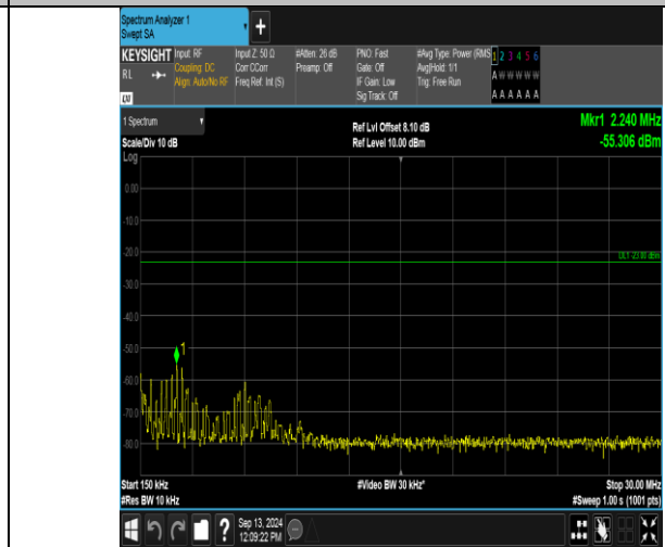
Band12_3MHz_QPSK_23165_1RB#14_0.15~30_0.15~30
