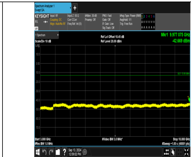
Band12_3MHz_16QAM_23165_1RB#0_3000~10000_3000~10000
