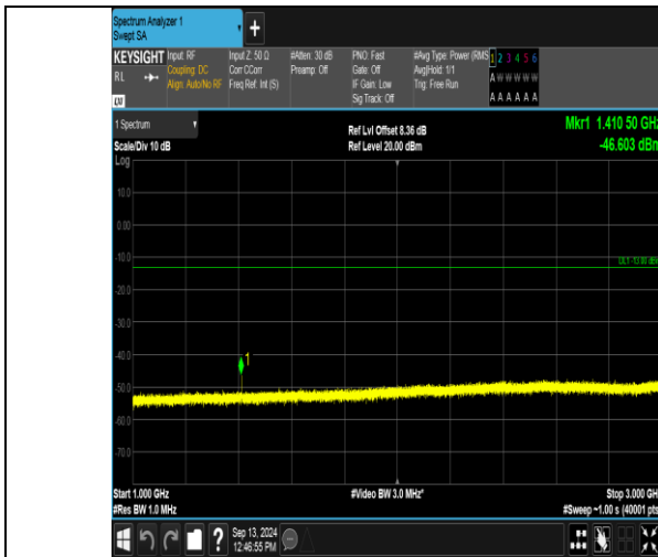
Band12_5MHz_16QAM_23095_1RB#0_1000~3000_1000~3000
