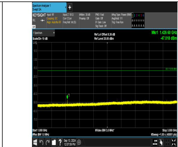
Band12_3MHz_QPSK_23165_1RB#0_1000~3000_1000~3000
