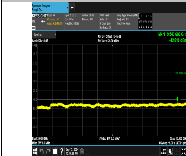
Band12_5MHz_QPSK_23095_25RB#0_3000-10000_3000-10000
