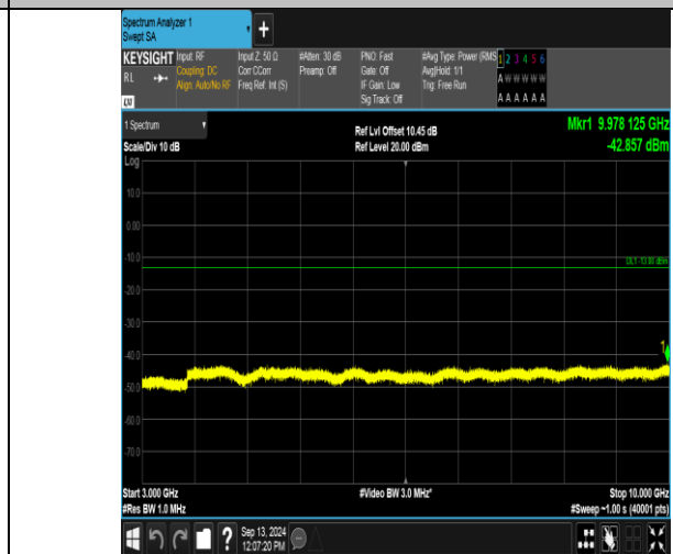
Band12_3MHz_16QAM_23095_15RB#0_3000~10000_3000~10000
