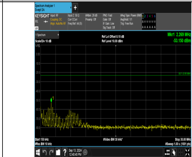
Band12_5MHz_QPSK_23035_1RB#0_0.15~30_0.15~30
