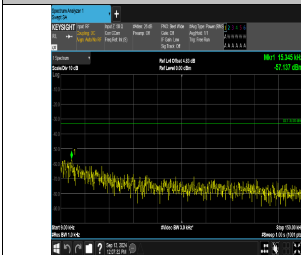
Band12_3MHz_QPSK_23165_1RB#0_0.009~0.15_0.009~0.15
