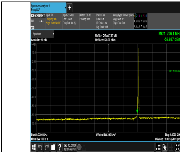
Band12_3MHz_QPSK_23165_1RB#0_30~1000_30~1000
