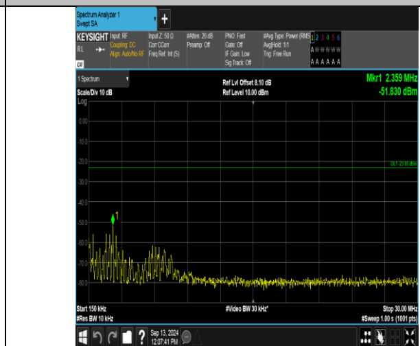
Band12_3MHz_QPSK_23165_1RB#0_0.15~30_0.15~30
