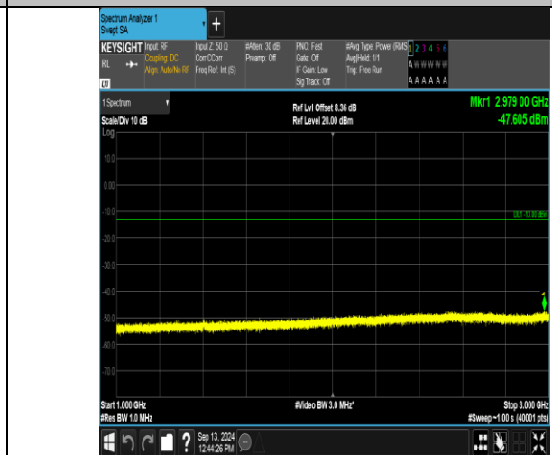
Band12_5MHz_QPSK_23035_25RB#0_1000-3000_1000-3000
