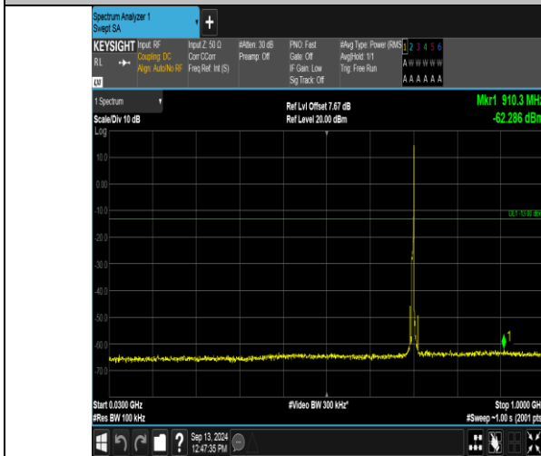
Band12_5MHz_QPSK_23095_1RB#24_30~1000_30~1000
