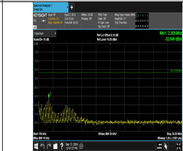
Band12_5MHz_QPSK_23095_1RB#24_0.15~30_0.15~30
