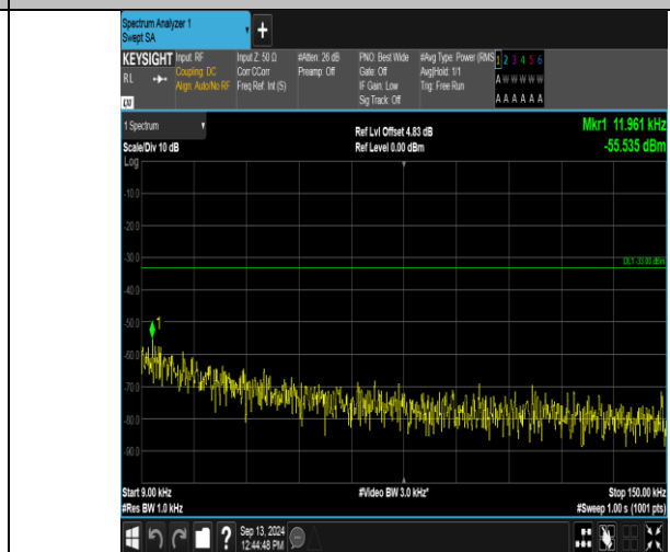
Band12_5MHz_16QAM_23035_25RB#0_0.009-0.15_0.009-0.15
