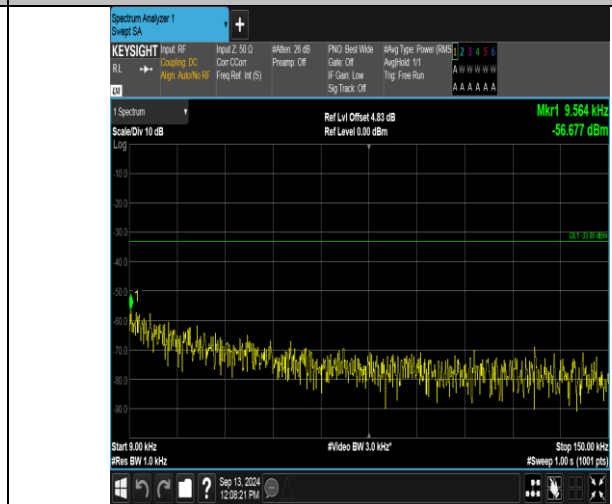
Band12_3MHz_16QAM_23165_1RB#0_0.009~0.15_0.009~0.15
