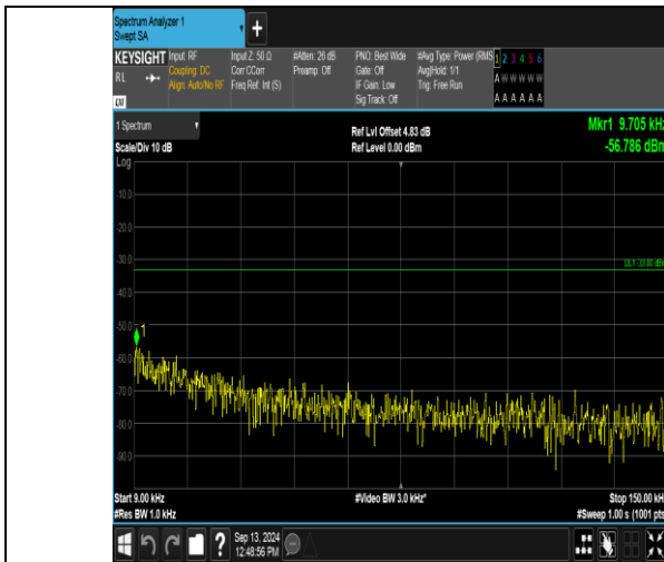
Band12_5MHz_QPSK_23095_25RB#0_0.009-0.15_0.009-0.15
