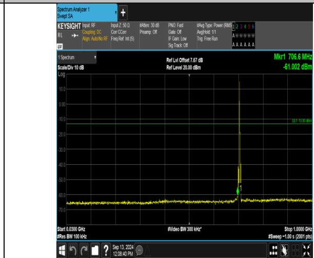
Band12_3MHz_16QAM_23165_1RB#0_30~1000_30~1000
