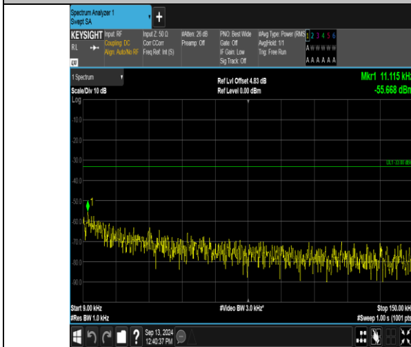
Band12_5MHz_QPSK_23035_1RB#0_0.009~0.15_0.009~0.15
