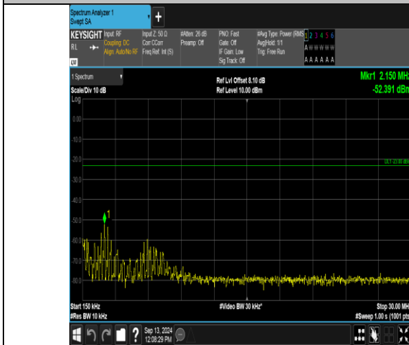
Band12_3MHz_16QAM_23165_1RB#0_0.15~30_0.15~30
