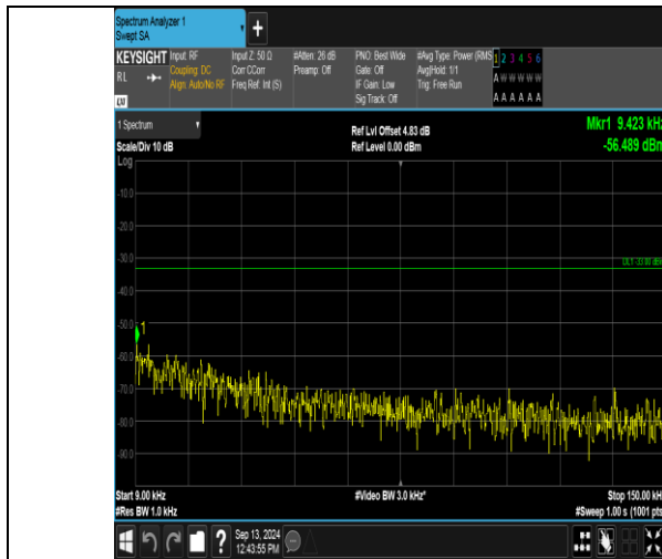
Band12_5MHz_QPSK_23035_25RB#0_0.009-0.15_0.009-0.15
