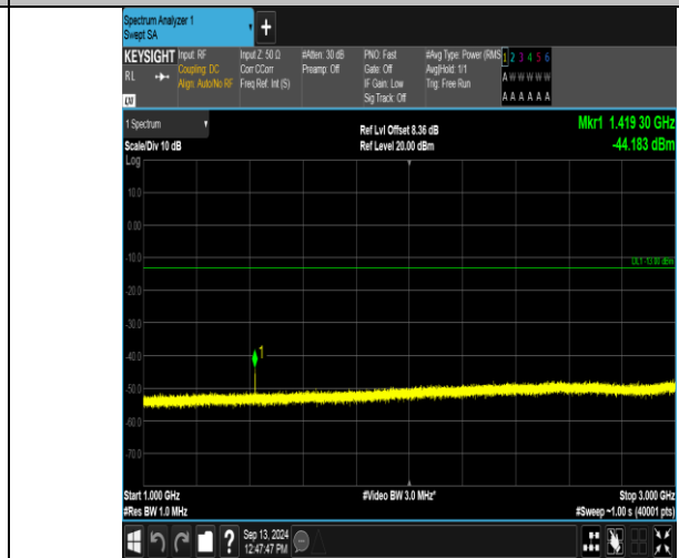
Band12_5MHz_QPSK_23095_1RB#24_1000~3000_1000~3000
