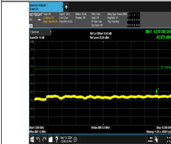
Band12_3MHz_QPSK_23165_1RB#0_3000~10000_3000~10000
