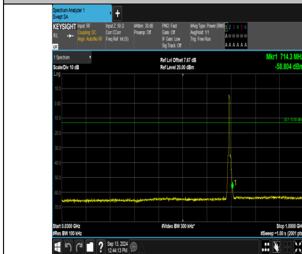
Band12_5MHz_QPSK_23035_25RB#0_30-1000_30-1000
