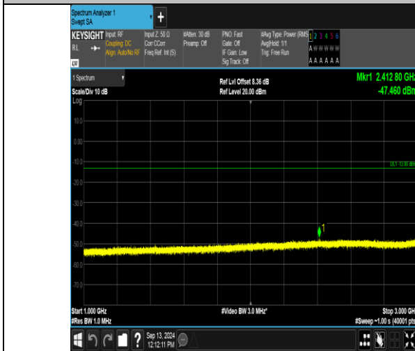
Band12_3MHz_16QAM_23165_15RB#0_1000~3000_1000~3000
