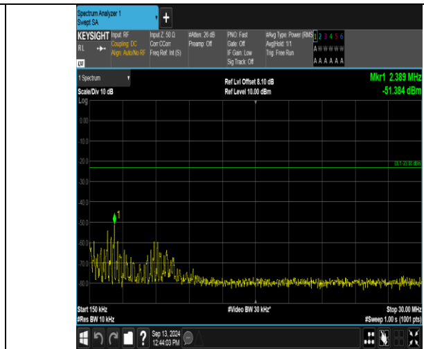
Band12_5MHz_QPSK_23035_25RB#0_0.15-30_0.15-30
