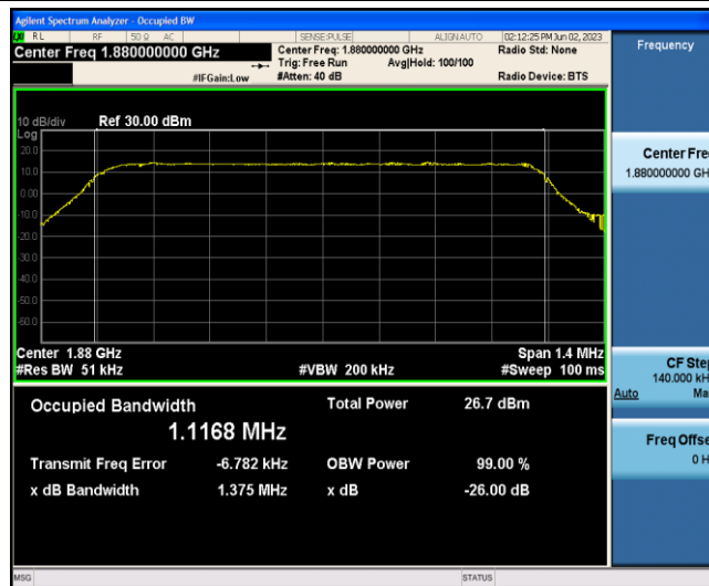
Band2-1.4MHz-QPSK-18900-6-0-Low-1.1168-1.375-PASS
