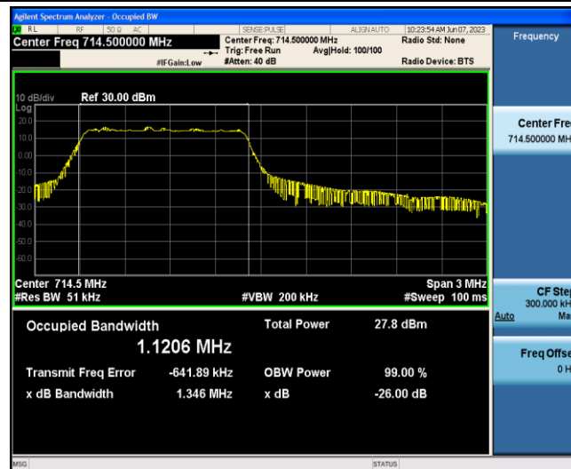
Band12-3MHz-16QAM-23165-6-0-Low-1.1206-1.346-PASS
