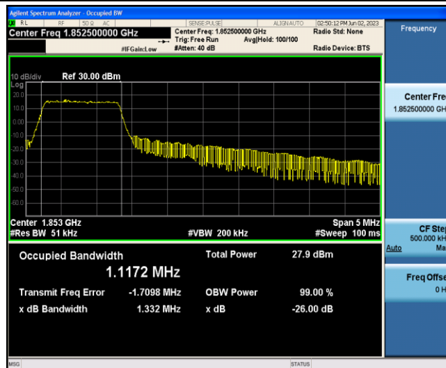
Band2-5MHz-16QAM-18625-6-0-Low-1.1172-1.332-PASS
