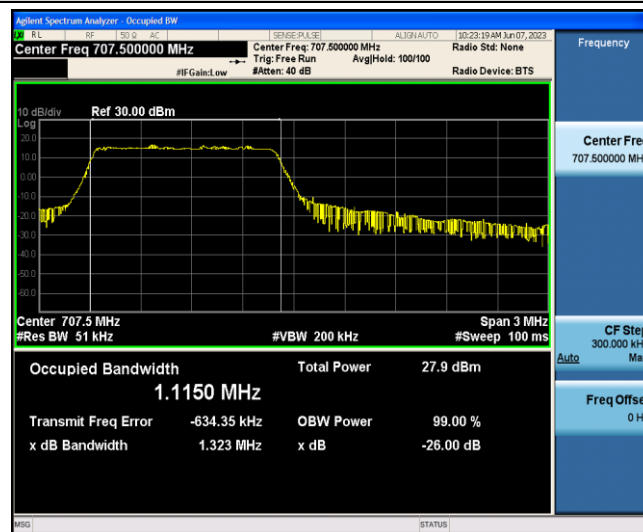
Band12-3MHz-16QAM-23095-6-0-Low-1.1150-1.323-PASS
