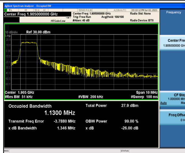
Band2-10MHz-QPSK-19150-6-0-Low-1.1300-1.346-PASS
