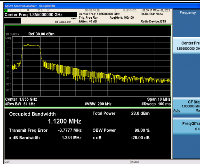
Band2-10MHz-16QAM-18650-6-0-Low-1.1200-1.331-PASS
