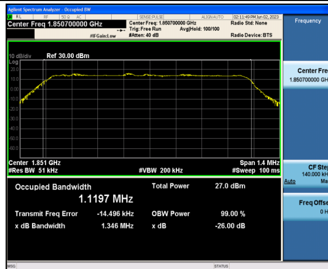
Band2-1.4MHz-QPSK-18607-6-0-Low-1.1197-1.346-PASS
