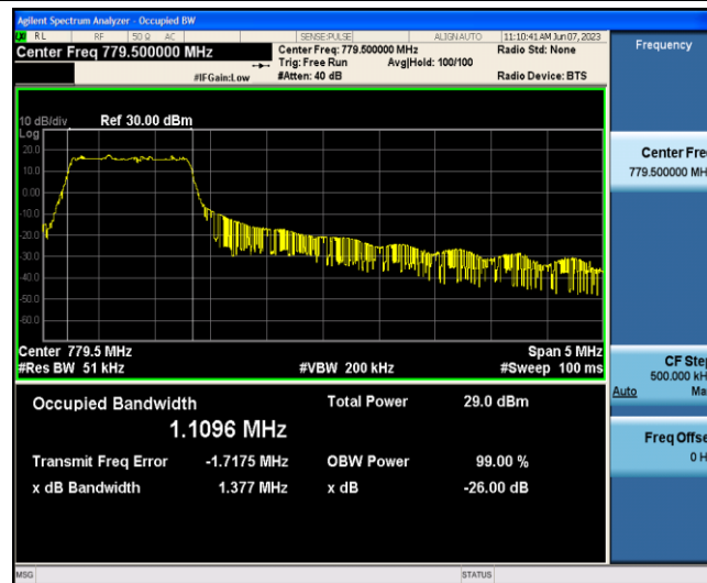
Band13-5MHz-16QAM-23205-6-0-Low-1.1096-1.377-PASS
