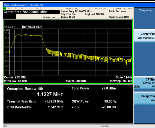
Band13-5MHz-16QAM-23230-6-0-Low-1.1227-1.342-PASS
