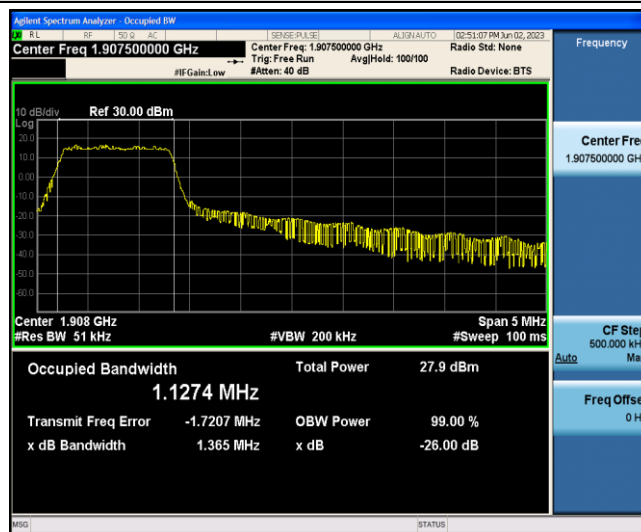
Band2-5MHz-QPSK-19175-6-0-Low-1.1274-1.365-PASS
