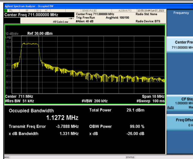
Band12-10MHz-QPSK-23130-6-0-Low-1.1272-1.331-PASS
