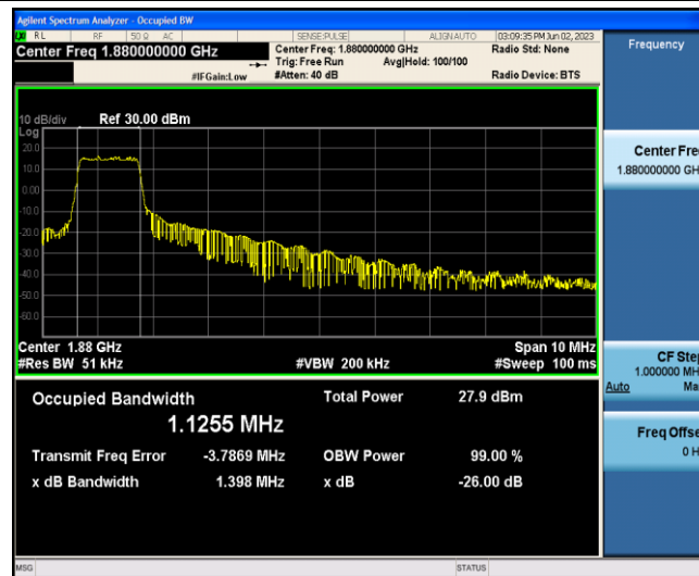
Band2-10MHz-QPSK-18900-6-0-Low-1.1255-1.398-PASS
