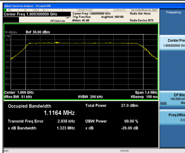
Band2-1.4MHz-QPSK-19193-6-0-Low-1.1164-1.323-PASS
