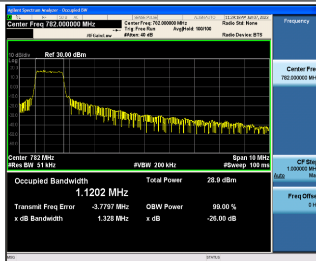
Band13-10MHz-16QAM-23230-6-0-Low-1.1202-1.328-PASS
