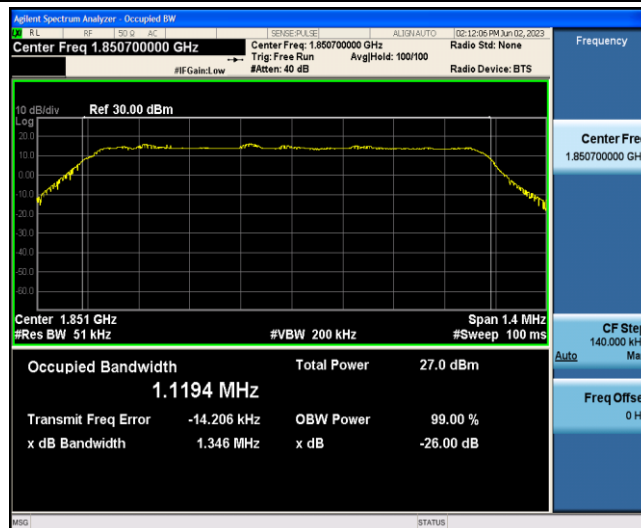
Band2-1.4MHz-16QAM-18607-6-0-Low-1.1194-1.346-PASS
