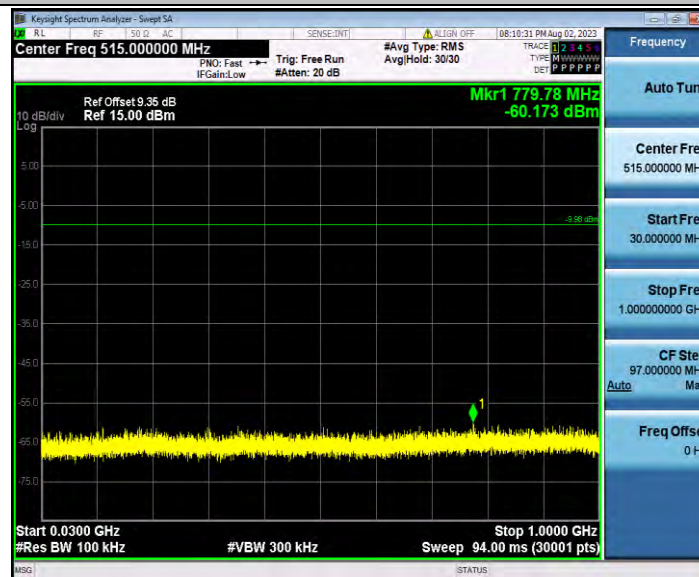
2DH1_Ant2_2441_30~1000
