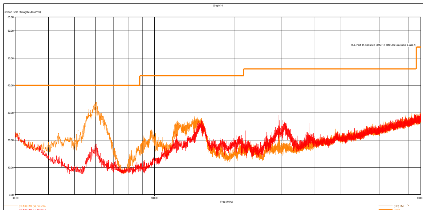
Figure 8 - Radiated Emissions Plot, GMSK 2MB
