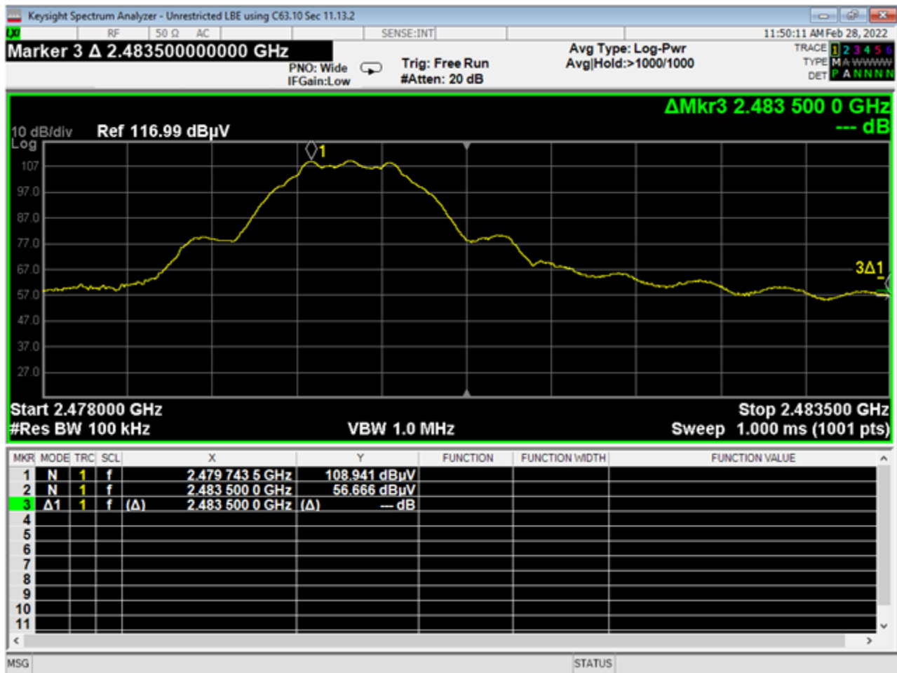
11 High Bandedge, Unrestricted, GMSK 1MB
