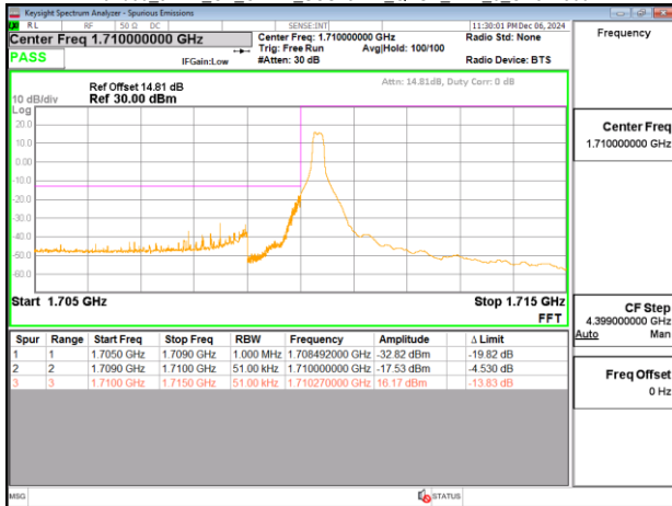
Band66_5MHz_CP_OFDM_SCS15kHz_QPSK_RB25_0_CH342500
