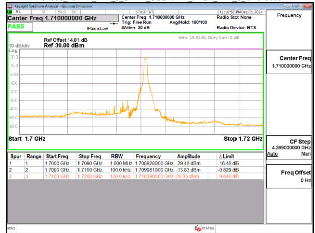
Band66_10MHz_DFT_s_OFDM_SCS15kHz_BPSK_RB50_0_CH343000
