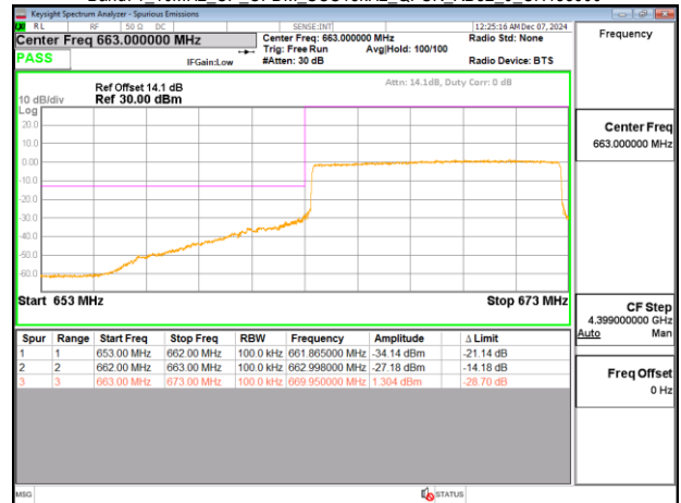
Band71_10MHz_CP_OFDM_SCS15kHz_QPSK_RB52_0_CH133600
