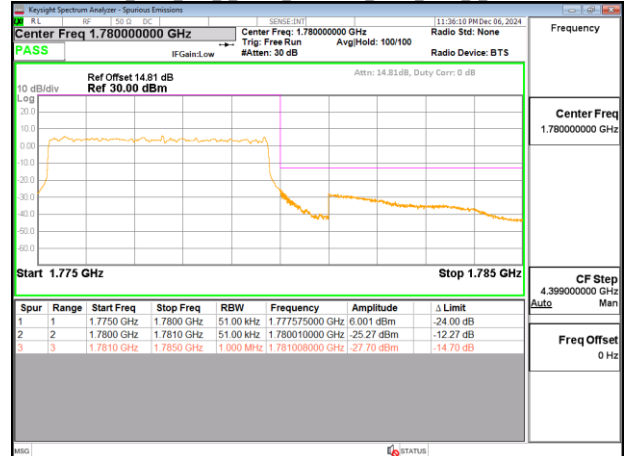
Band66_5MHz_DFT_s_OFDM_SCS15kHz_BPSK_RB25_0_CH355500
