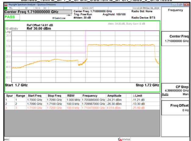
Band66_10MHz_DFT_s_OFDM_SCS15kHz_BPSK_RB50_0_CH343000
