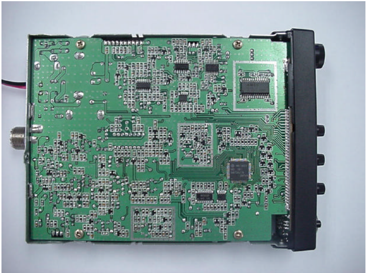
Solder Side of Board
