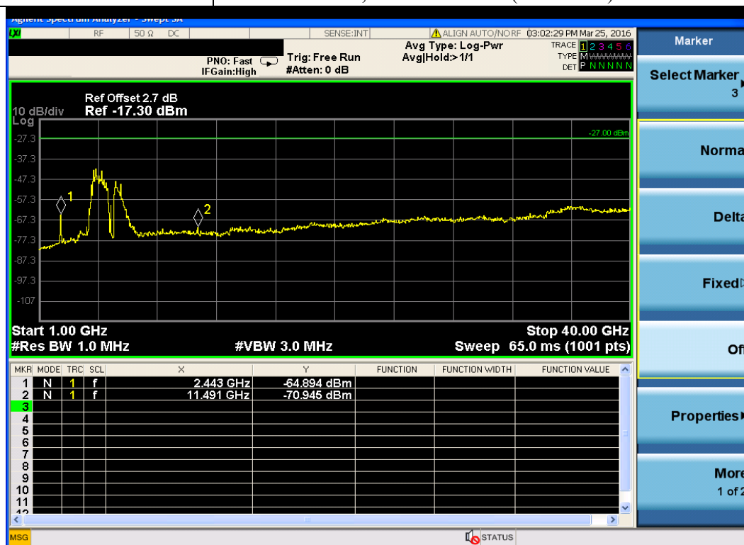
Title: TX Spurious Emissions from 1GHz-40GHz – Ch149 (5745 MHz)
