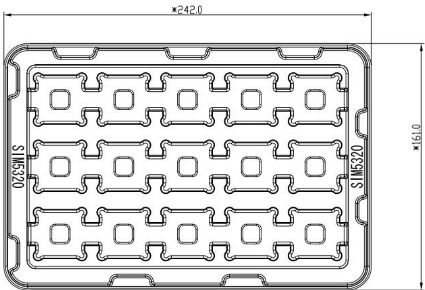
Figure 44: Tray drawing
