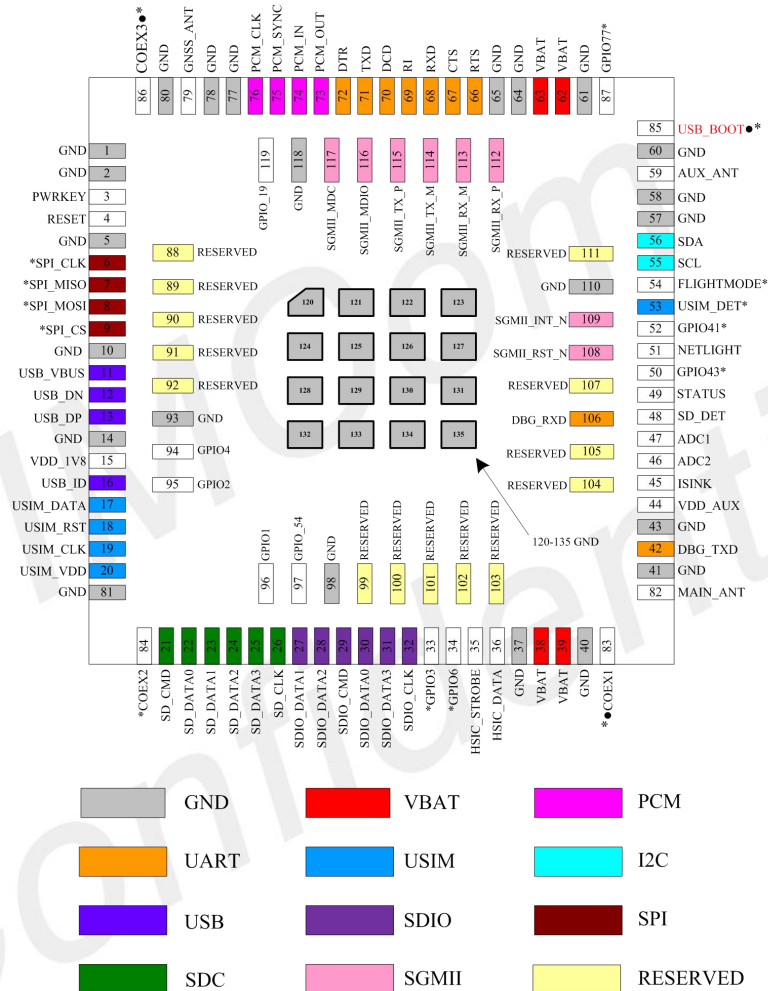
Figure 2: Pin assignment overview
