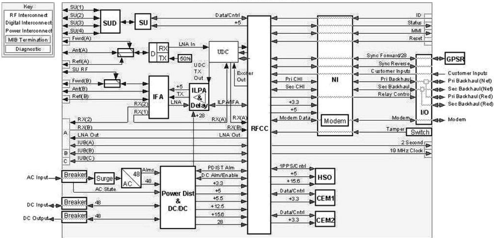
Block Diagram of SC300 @ 1.9 GHz
