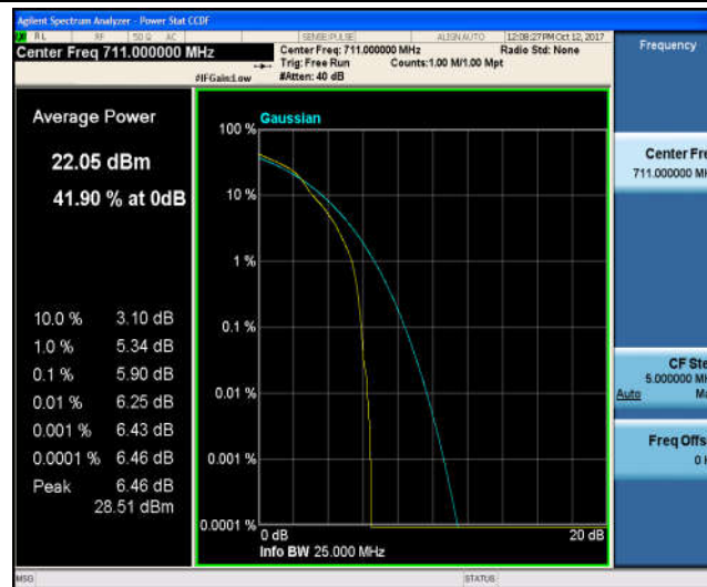
Band17_10MHz_QPSK_23800_50RB#0_5.72_13_PASS
