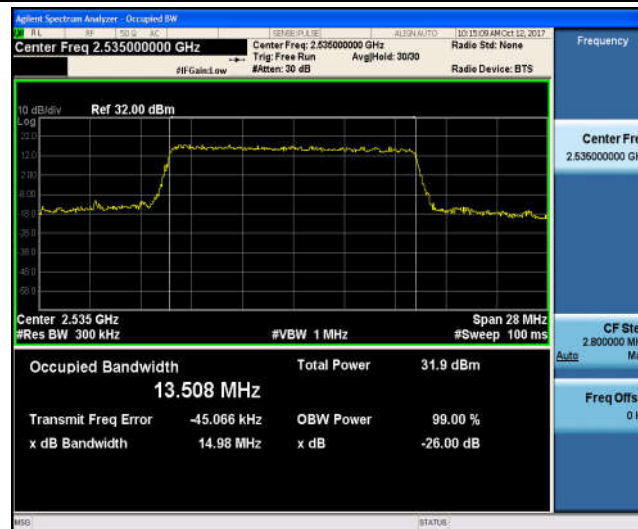
Band7_15MHz_16QAM_21100_75RB#0_13.493_14.82_PASS
