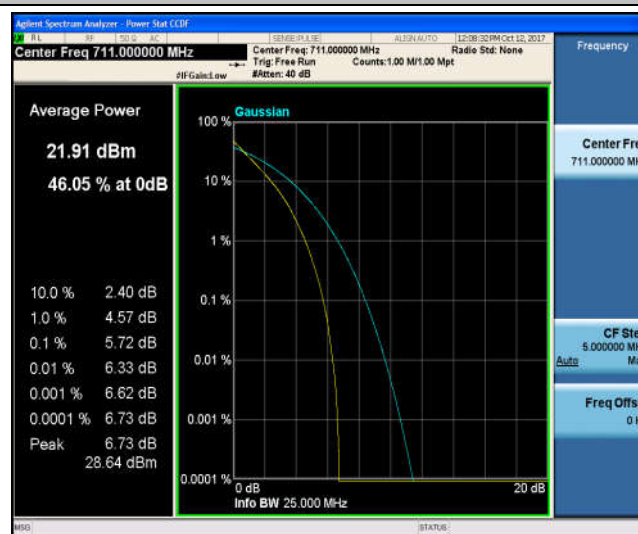
Band17_10MHz_16QAM_23800_50RB#0_6.50_13_PASS
