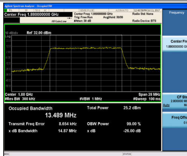
Band2_15MHz_16QAM_18900_75RB#0_13.455_14.83_PASS
