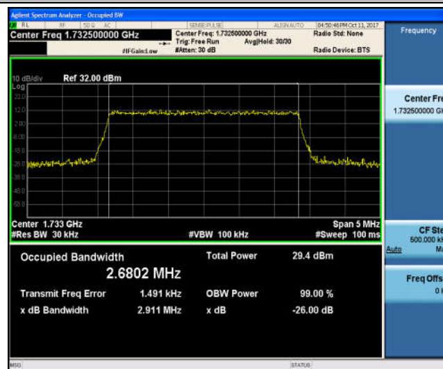
Band4_3MHz_QPSK_20385_15RB#0_2.6819_2.877_PASS
