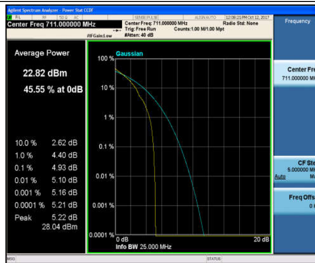
Band17_10MHz_16QAM_23800_1RB#0_5.90_13_PASS
