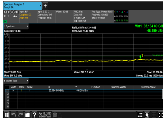
N78(100M)_DFT-s- OFDM_QPSK_Edge_1RB_Left_Low_CH
