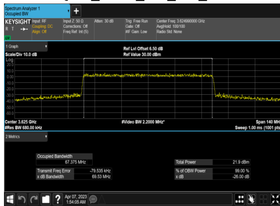
N78(70M)_CP-OFDM_16 QAM_Outer_Full_Mid_CH
