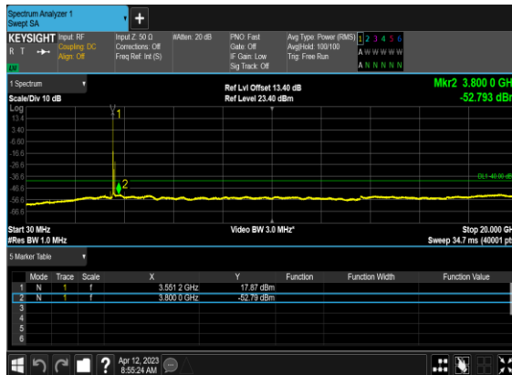
N78(100M)_DFT-s- OFDM_QPSK_Edge_1RB_Left_Low_CH
