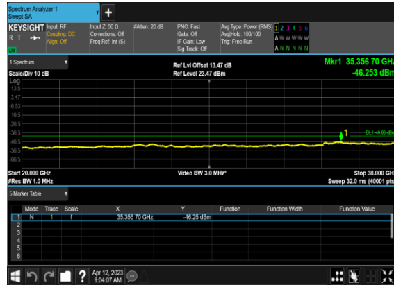
N78(100M)_DFT-s- OFDM_BPSK_Edge_1RB_Left_High_CH
