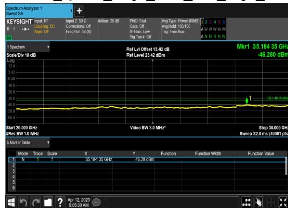
N78(100M)_DFT-s- OFDM_QPSK_Edge_1RB_Left_High_CH
