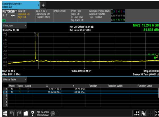
N78(100M)_DFT-s- OFDM_BPSK_Edge_1RB_Left_High_CH
