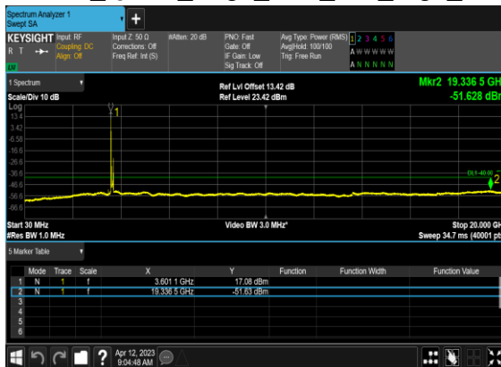
N78(100M)_DFT-s- OFDM_QPSK_Edge_1RB_Left_High_CH
