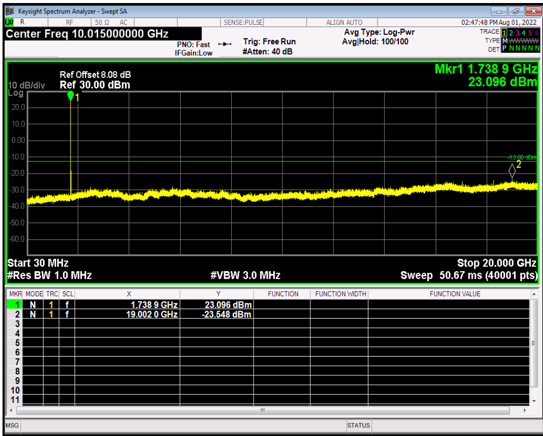
HSDPA Band4 Subtest4 Channel=1450
