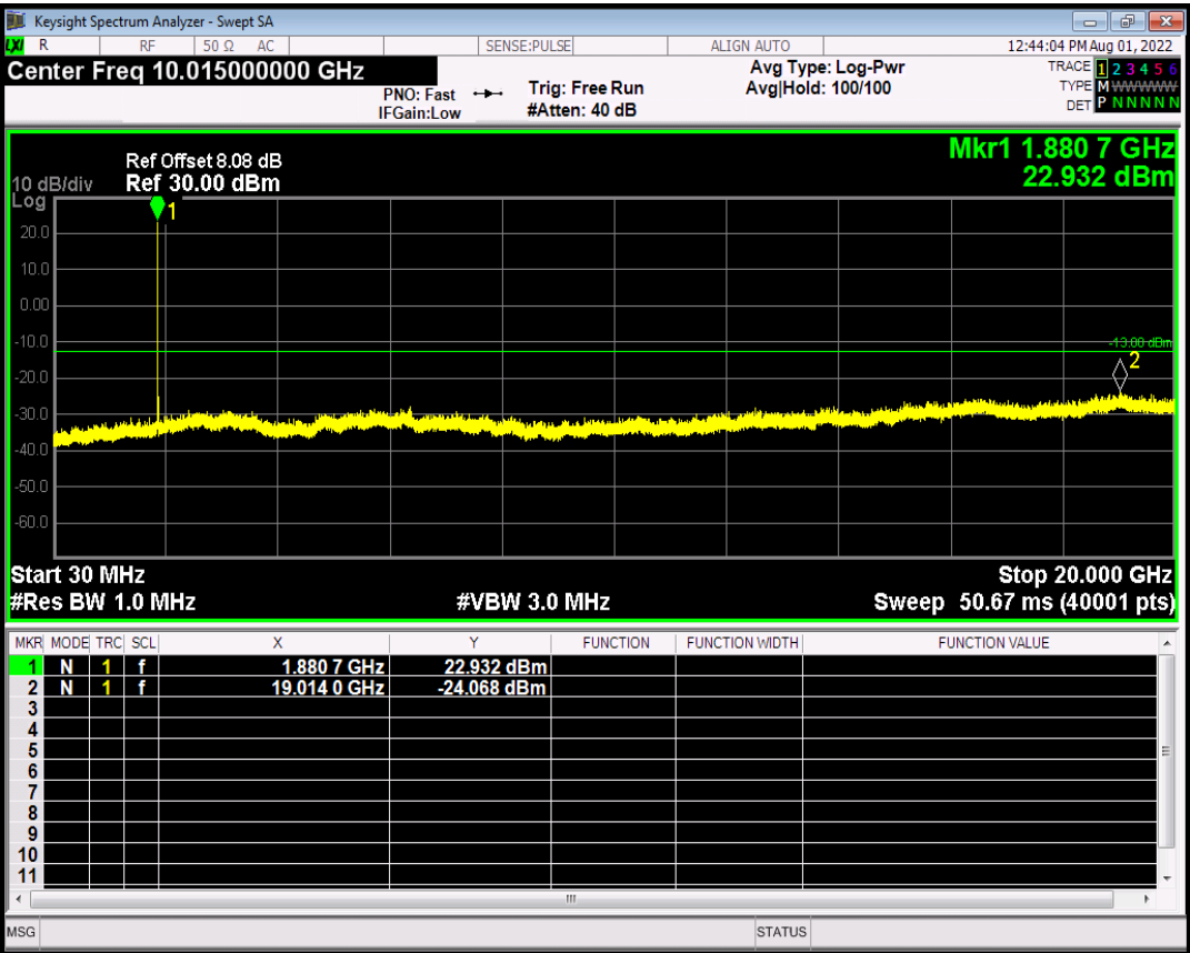
HSDPA Band2 Subtest3 Channel=9400
