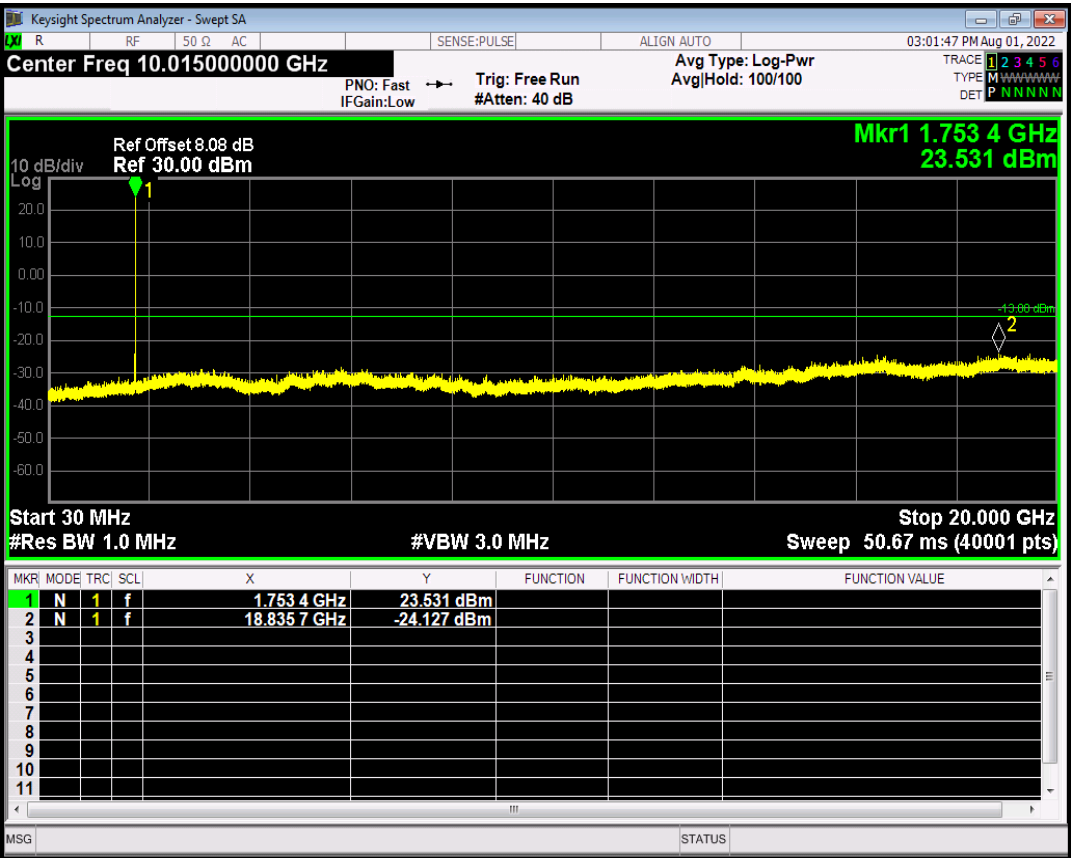
HSUPA Band4 Subtest5 Channel=1513
