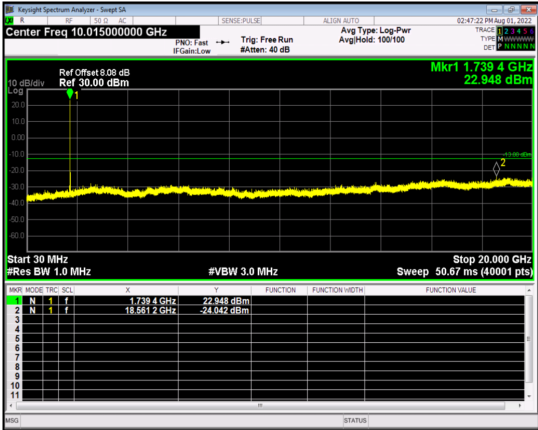
HSDPA Band4 Subtest3 Channel=1450
