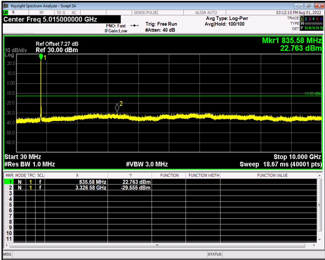
HSDPA Band5 Subtest3 Channel=4182
