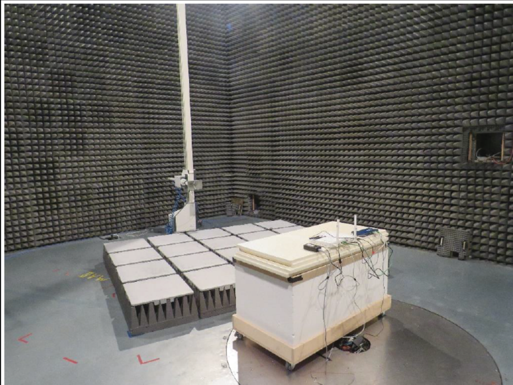
Setup for measurement above 1 GHz
