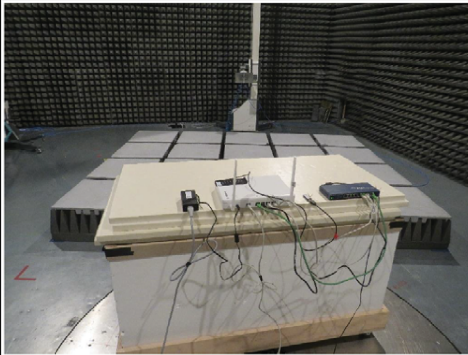
Setup for measurement above 1 GHz
