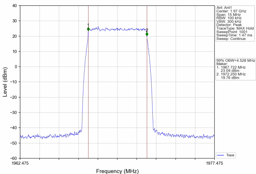
Band25_1969.975MHz_AWGN_SISO_Ant1_NTNV_AGC
