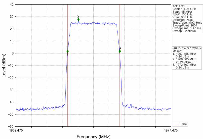
Band25_1969.975MHz_AWGN_SISO_Ant1_NTNV_AGC
