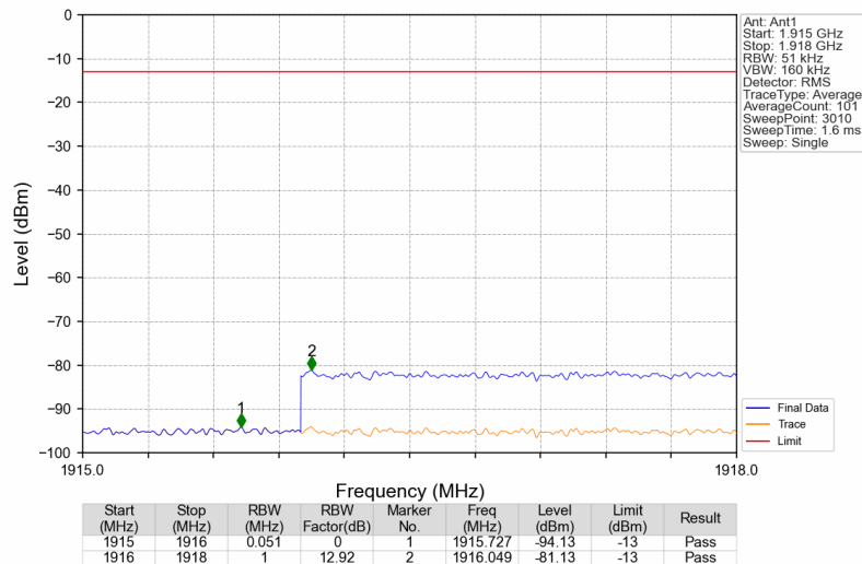
Band25_1992.5MHz_AWGN_SISO_Ant1_NTNV_AGC+3
