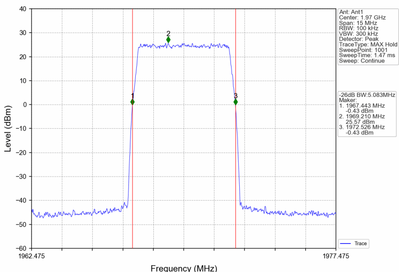
Band25_1969.975MHz_AWGN_SISO_Ant1_NTNV_AGC
