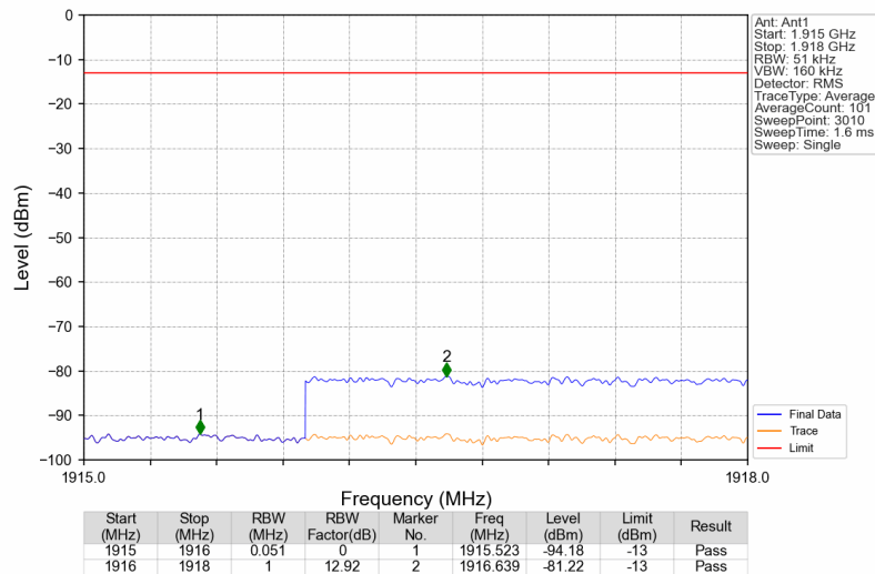
Band25_1992.5MHz_AWGN_SISO_Ant1_NTNV_AGC
