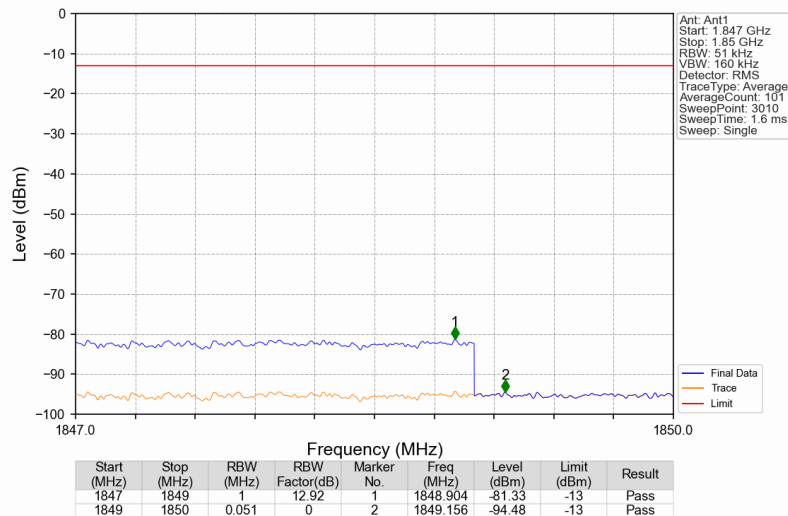
Band25_1932.5MHz_AWGN_SISO_Ant1_NTNV_AGC+3
