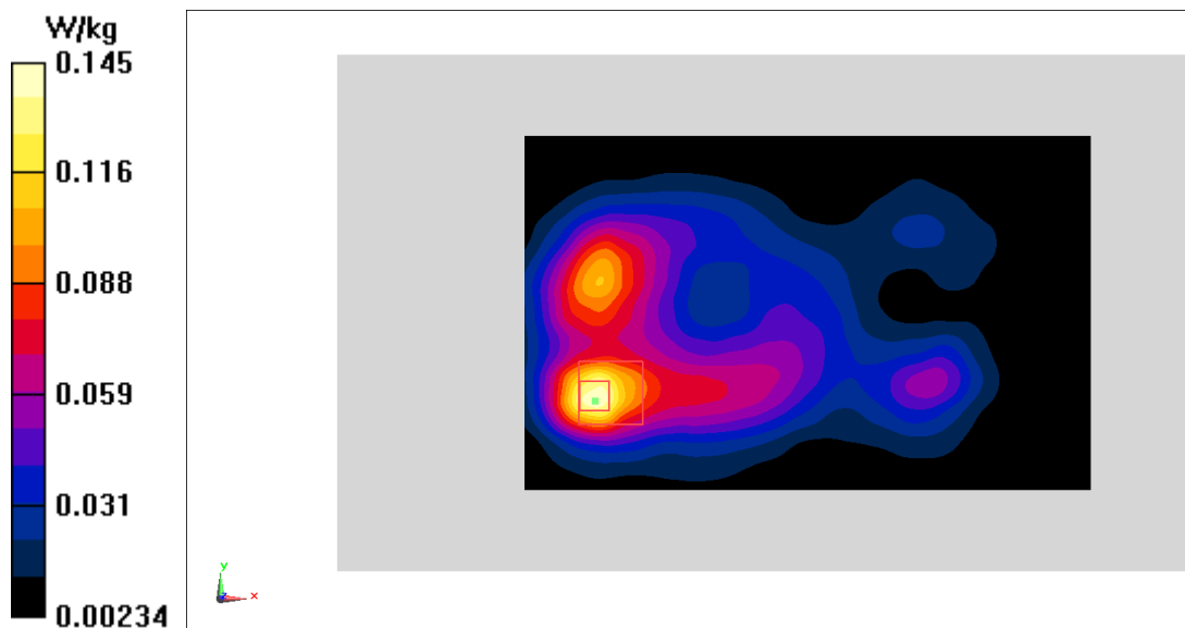
Fig.12 2450 MHz
