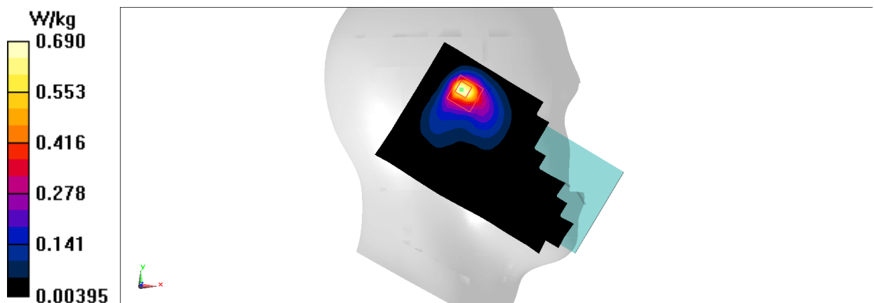
Fig.11 2450 MHz
