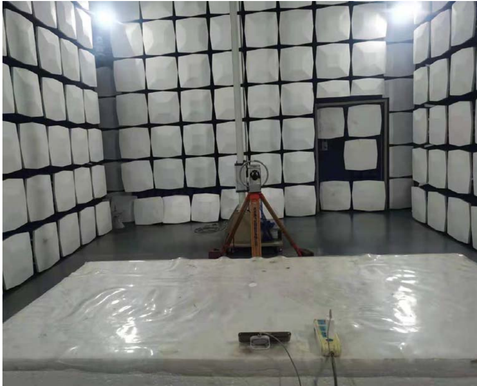
Radiated Emission Test Setup:
