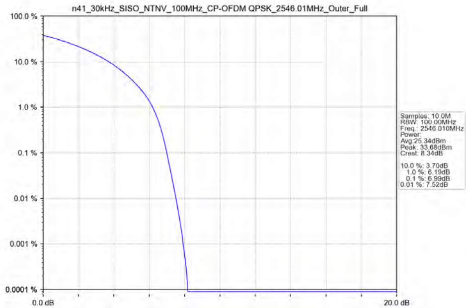
n41_30kHz_SISO_NTNV_100MHz_CP-OFDM_QPSK_2546.01MHz_Outer_Full_Ant41
