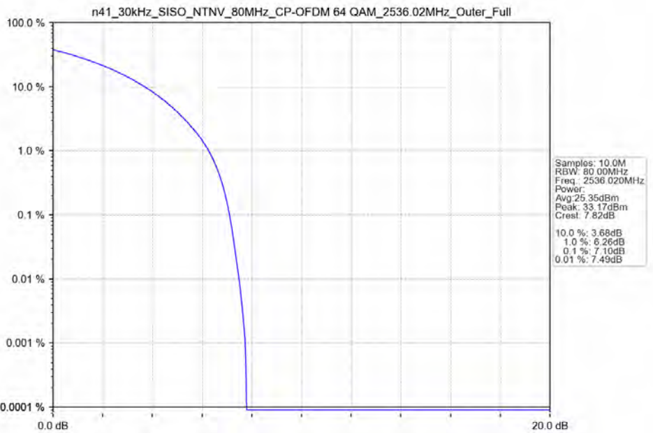
n41_30kHz_SISO_NTNV_80MHz_CP-OFDM 64 QAM 2536.02MHz_Outer_Full_Ant41
