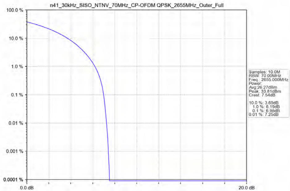
n41_30kHz_SISO_NTNV_70MHz_CP-OFDM_QPSK_2655MHz_Outer_Full_Ant41
