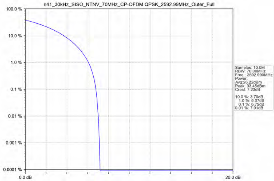
n41_30kHz_SISO_NTNV_70MHz_CP-OFDM_QPSK_2592.99MHz_Outer_Full_Ant41
