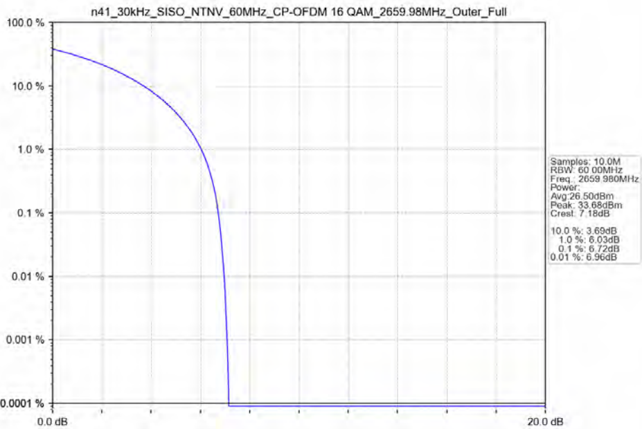
n41_30kHz_SISO_NTNV_60MHz_CP-OFDM 16 QAM_2659.98MHz_Outer_Full_Ant41
