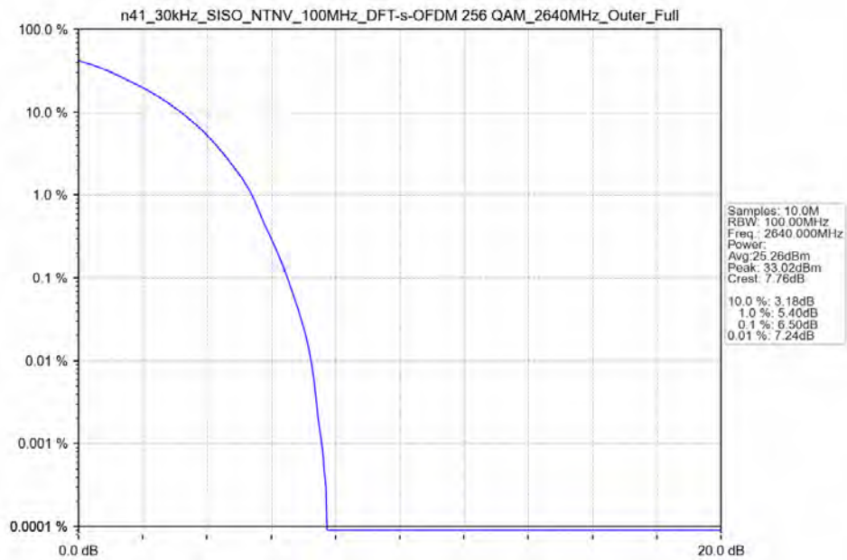
n41_30kHz_SISO_NTNV_100MHz_DFT-s-OFDM_256_QAM_2640MHz_Outer_Full_Ant41
