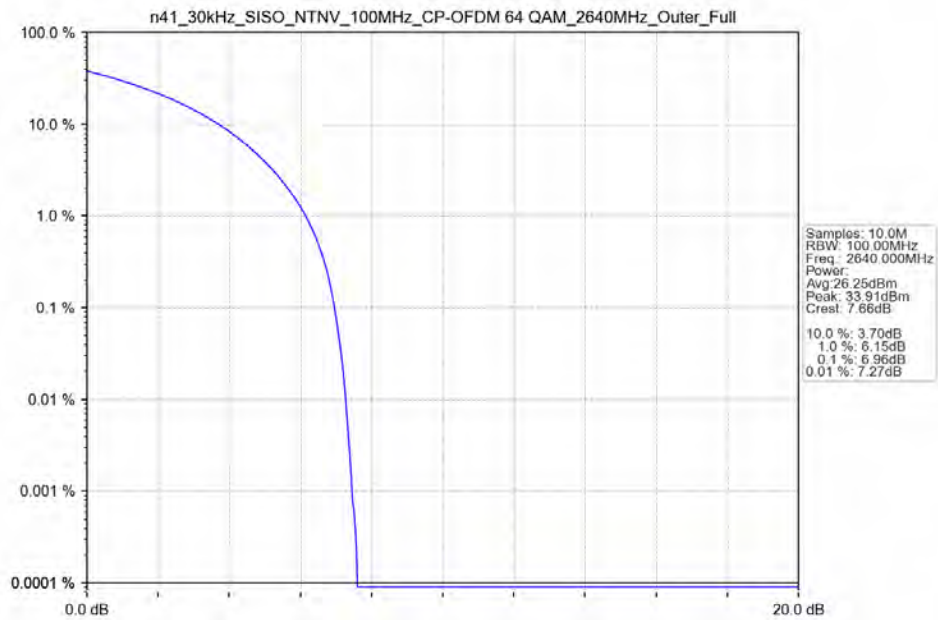
n41_30kHz_SISO_NTNV_100MHz_CP-OFDM 64 QAM_2640MHz_Outer_Full_Ant41
