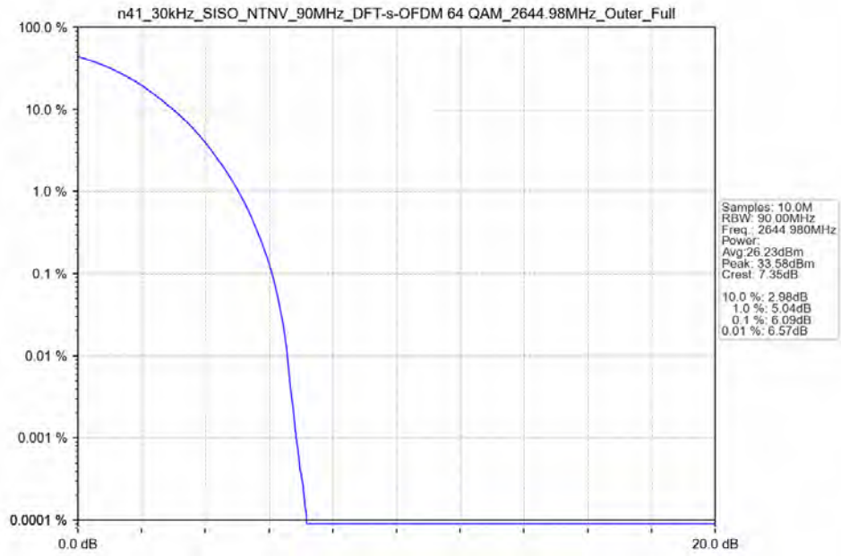
n41_30kHz_SISO_NTNV_90MHz_DFT-s-OFDM_64_QAM_2644.98MHz_Outer_Full_Ant41
