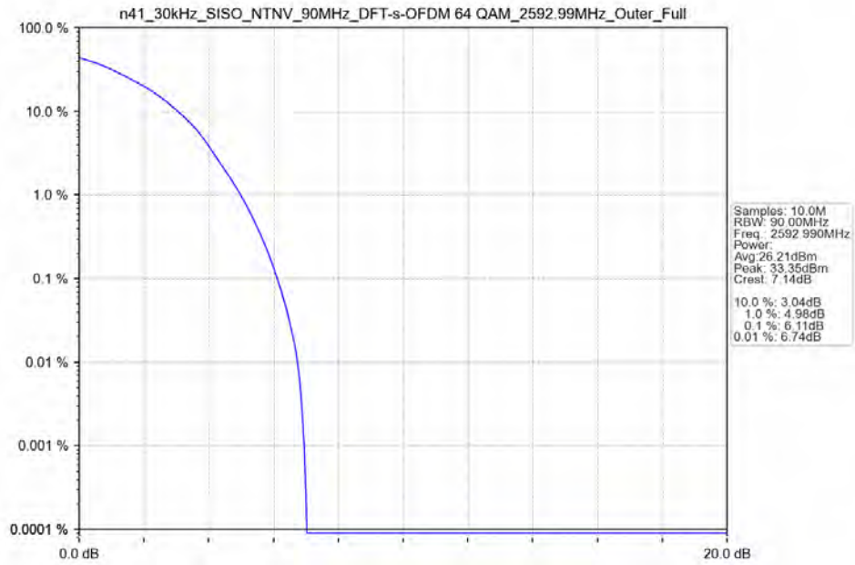
n41_30kHz_SISO_NTNV_90MHz_DFT-s-OFDM_64_QAM_2592.99MHz_Outer_Full_Ant41
