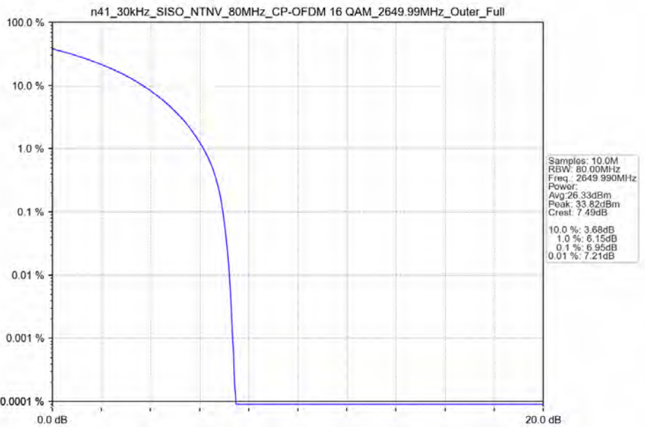
n41_30kHz_SISO_NTNV_80MHz_CP-OFDM 16 QAM 2649.99MHz_Outer_Full_Ant41
