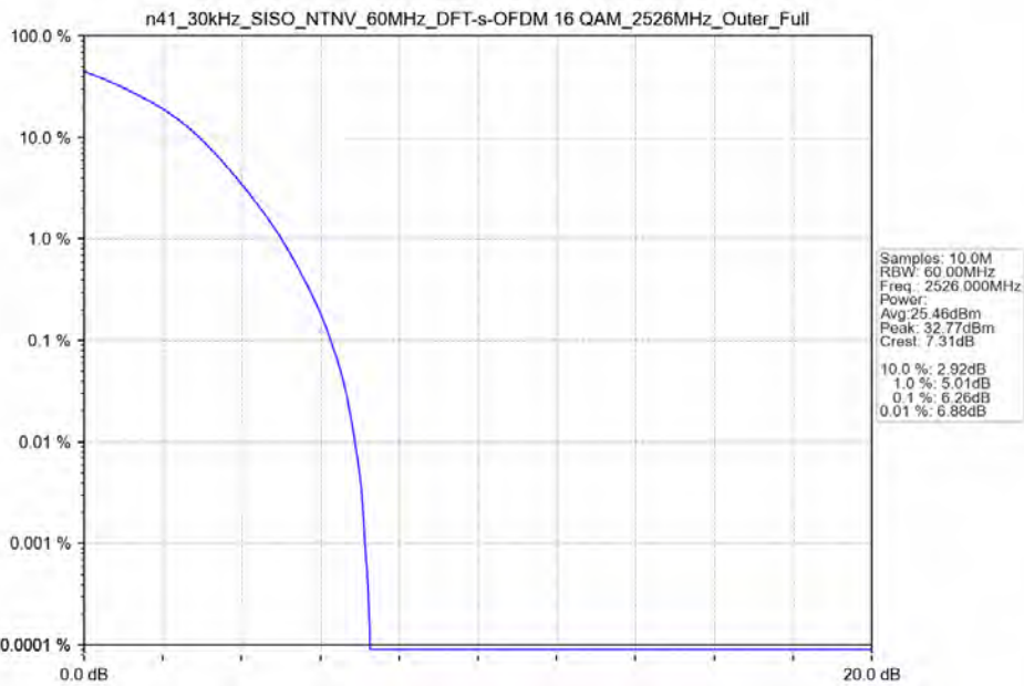
n41_30kHz_SISO_NTNV_60MHz_DFT-s-OFDM_16_QAM_2526MHz_Outer_Full_Ant41
