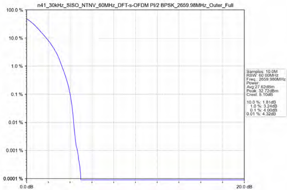
n41_30kHz_SISO_NTNV_60MHz_DFT-s-OFDM PI/2 BPSK_2659.98MHz_Outer_Full_Ant41
