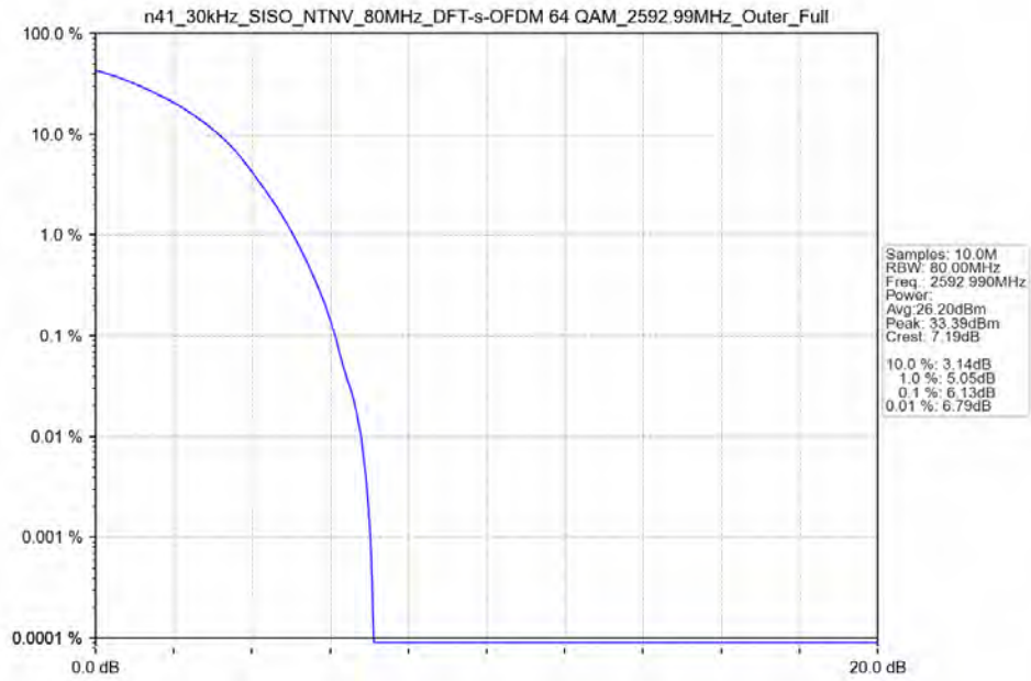
n41_30kHz_SISO_NTNV_80MHz_DFT-s-OFDM_64_QAM_2592.99MHz_Outer_Full_Ant41
