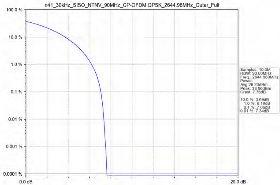
n41_30kHz_SISO_NTNV_90MHz_CP-OFDM_QPSK_2644.98MHz_Outer_Full_Ant41
