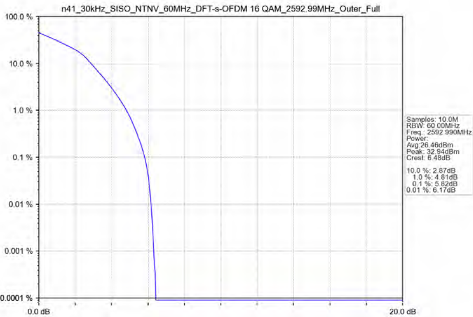
n41_30kHz_SISO_NTNV_60MHz_DFT-s-OFDM_16_QAM_2592.99MHz_Outer_Full_Ant41
