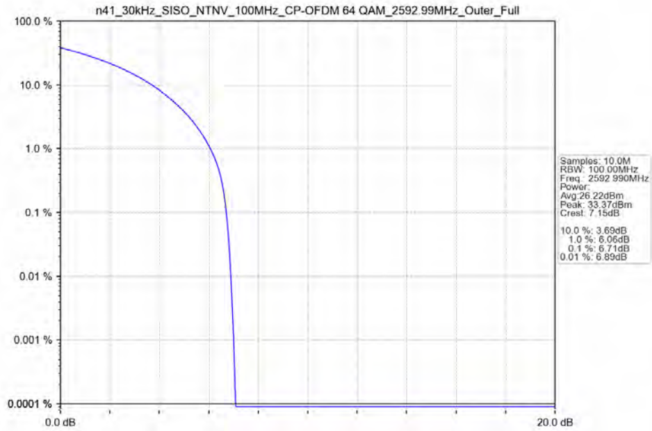
n41_30kHz_SISO_NTNV_100MHz_CP-OFDM 64 QAM_2592.99MHz_Outer_Full_Ant41
