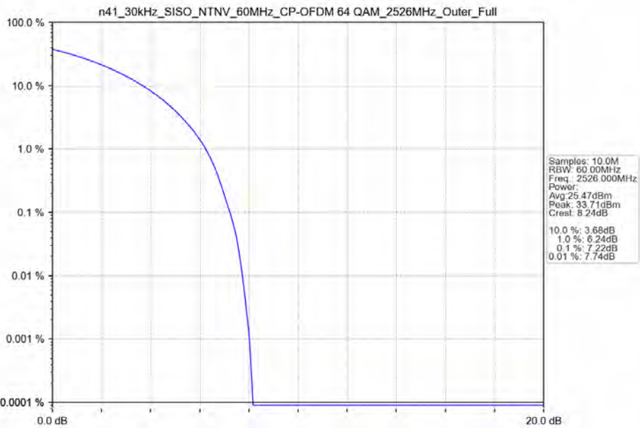
n41_30kHz_SISO_NTNV_60MHz_CP-OFDM 64 QAM_2526MHz_Outer_Full_Ant41
