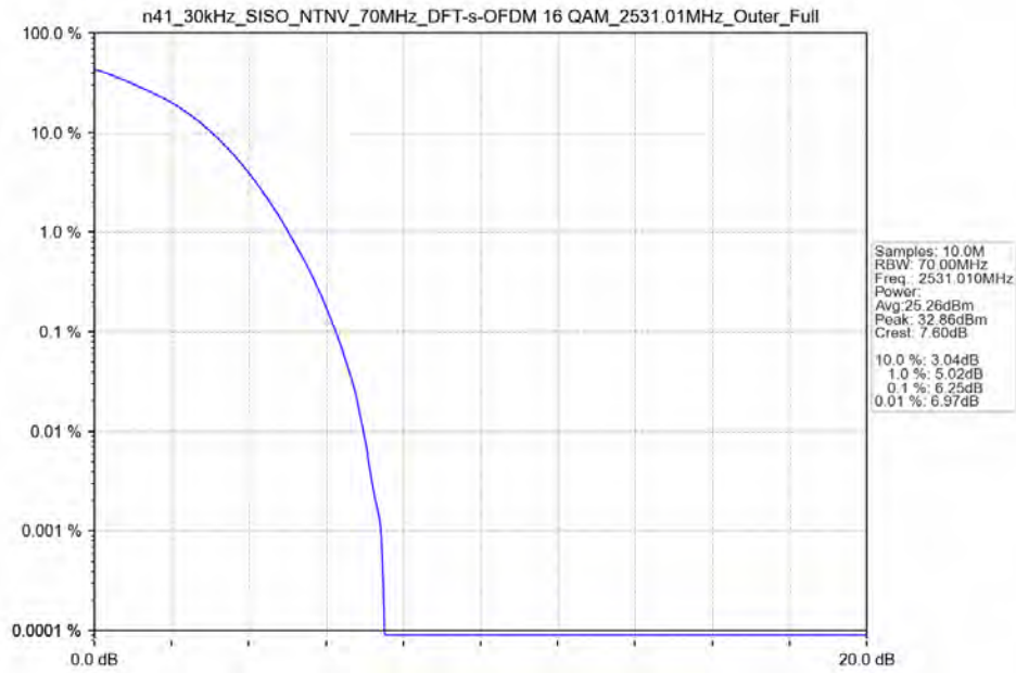
n41_30kHz_SISO_NTNV_70MHz_DFT-s-OFDM_16_QAM_2531.01MHz_Outer_Full_Ant41
