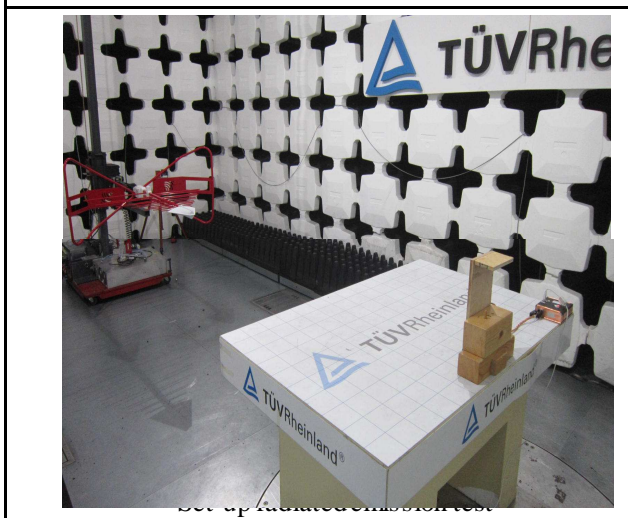
Set-up radiated emission test
