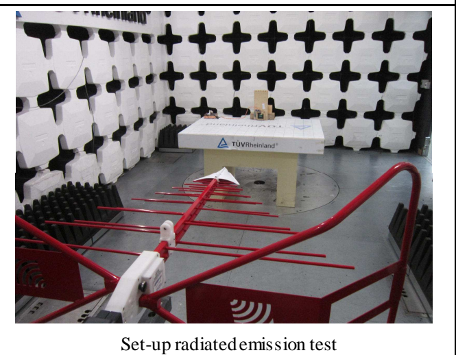
Set-up radiated emission test
