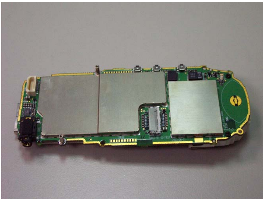
EUT SV10A/SV10B – Component View with Shield
