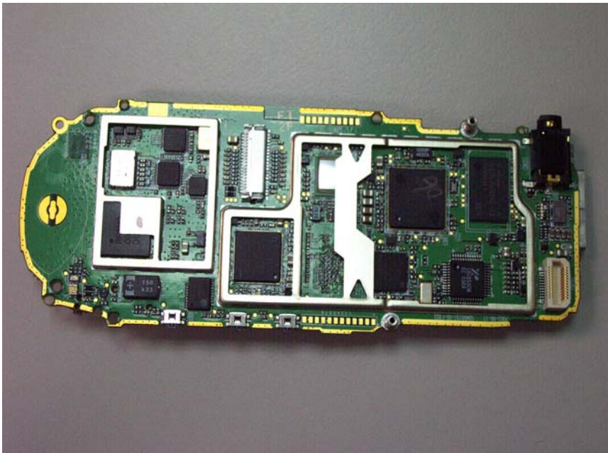
EUT SV10A/SV10B – Component View without Shield 2
