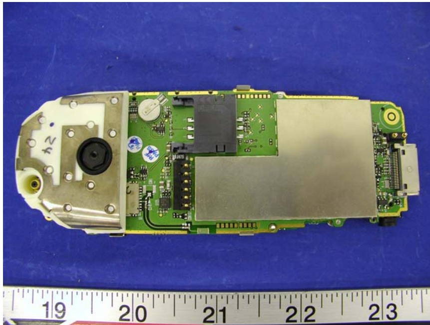
EUT SV10A/SV10B – Component View
