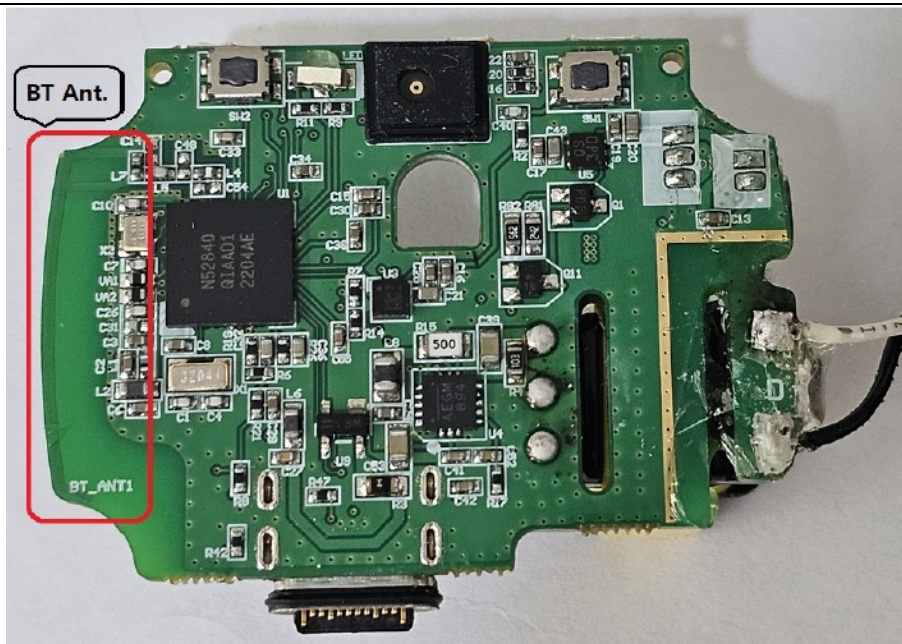
[Rear View of Main Board]
