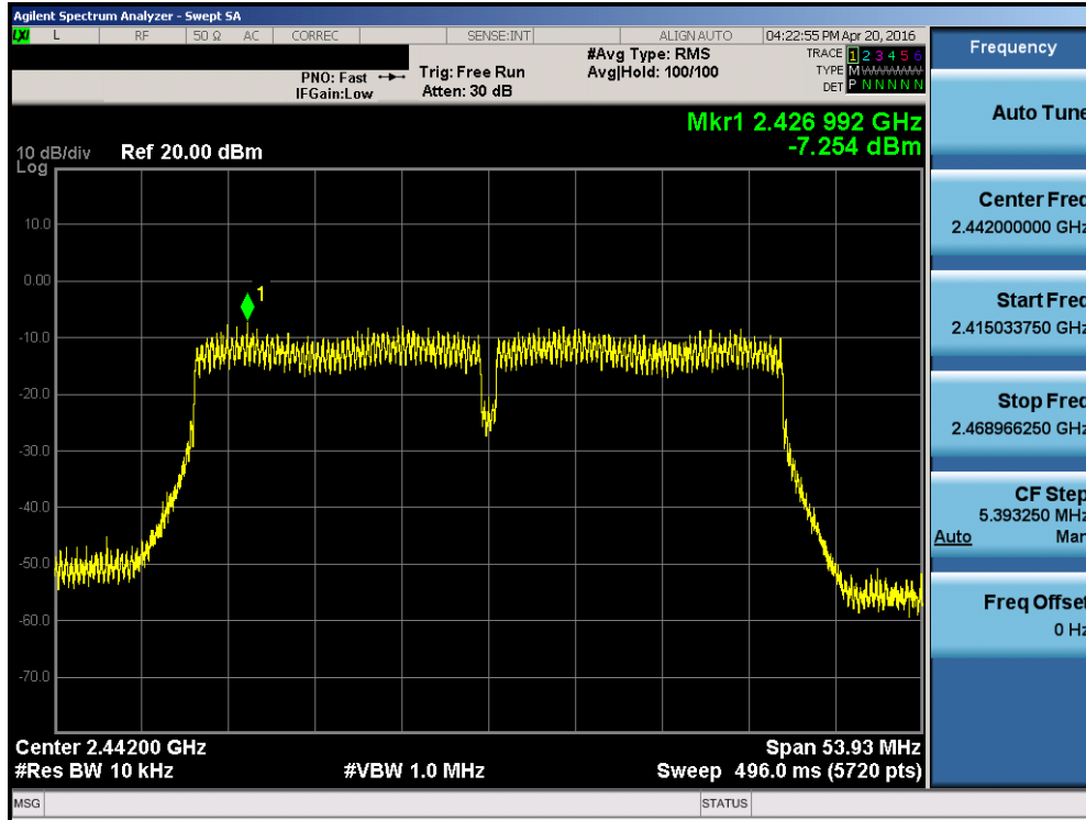
Plot 7-23. Power Spectral Density Plot (802.11n (40MHz BW) – Ch. 5 + 9)
