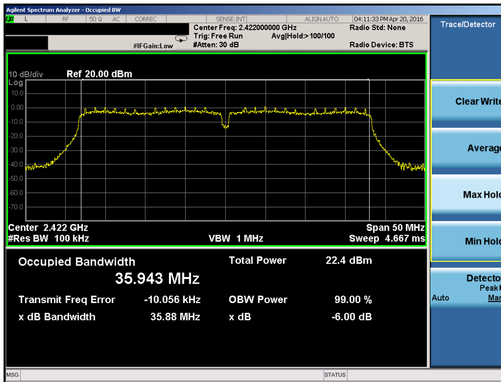
Plot 7-10. 6dB Bandwidth Plot (802.11n (40MHz BW) – Ch. 1 + 5)
