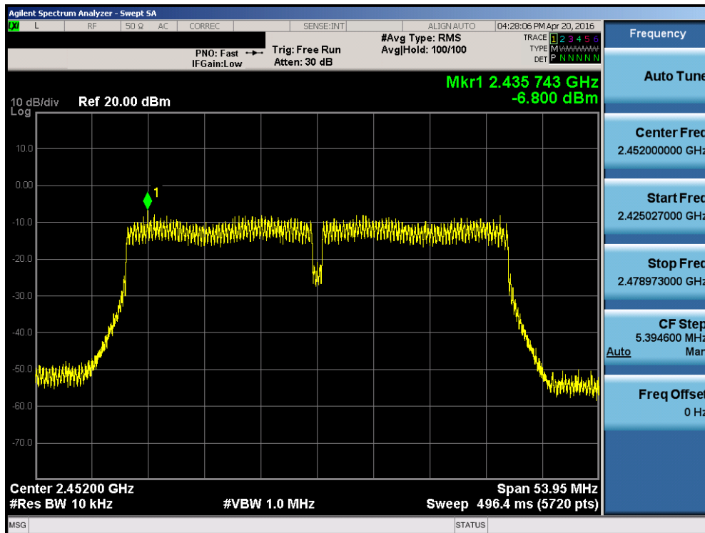
Plot 7-24. Power Spectral Density Plot (802.11n (40MHz BW) – Ch. 7 + 11)
