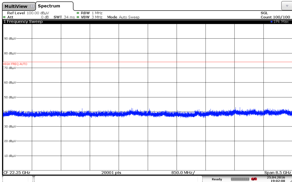
Plot 7-50. Radiated Spurious Plot above 18GHz (Pol. V)
