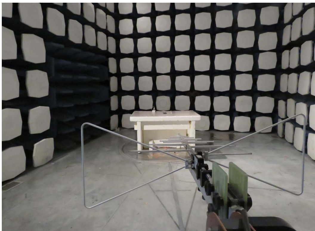
30MHz-1GHz
