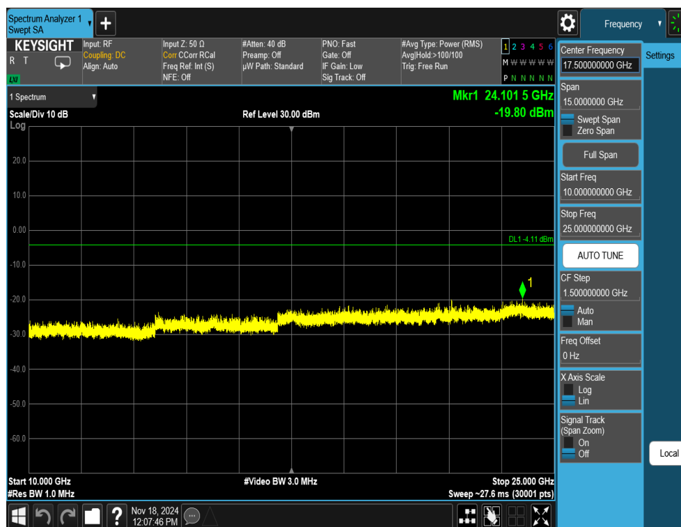
Plot 7-63. Conducted Spurious Plot Antenna WF8 (802.11ax OFDMA – RU26 – Ch. 1)
