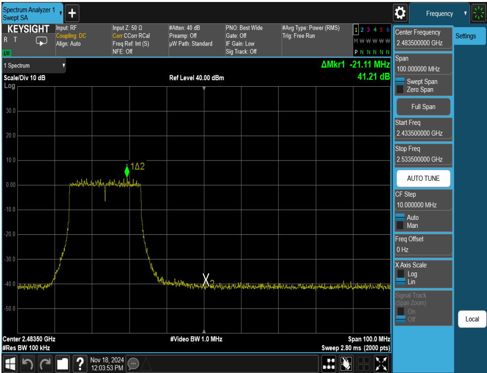
Plot 7-31. Band Edge Antenna WF8 (802.11ax OFDMA – RU242 – Ch. 10)
