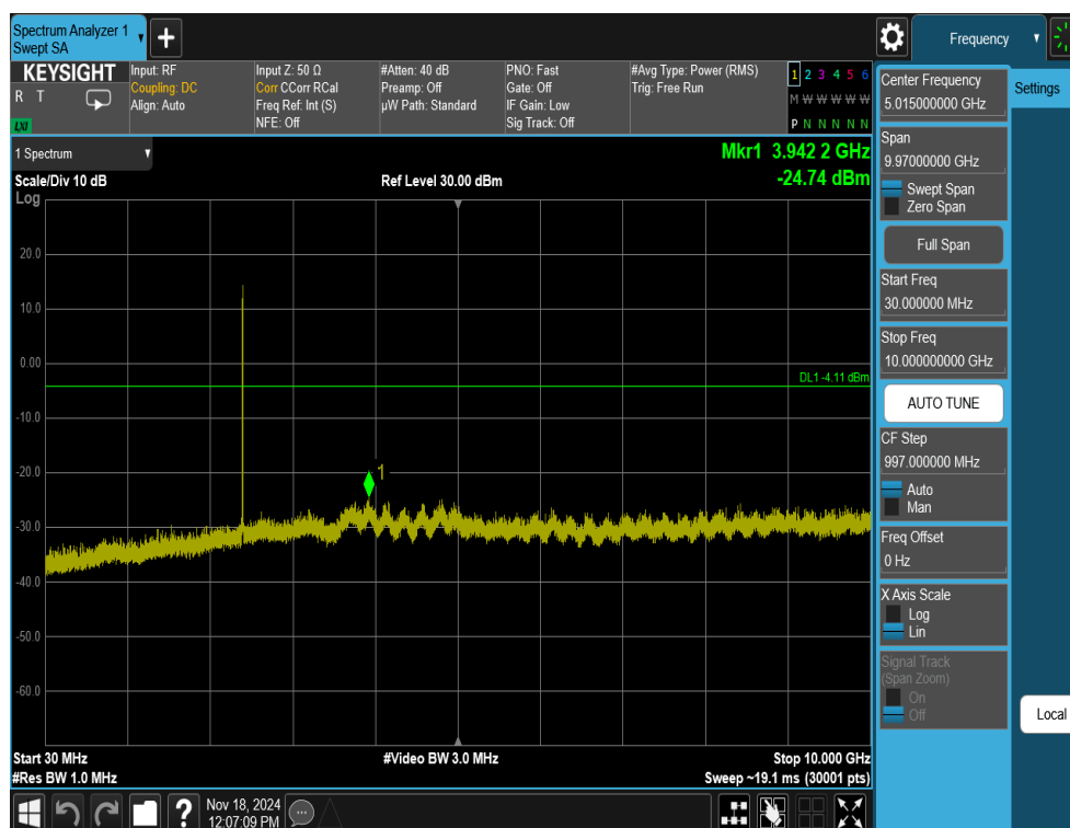
Plot 7-62. Conducted Spurious Plot Antenna WF8 (802.11ax OFDMA – RU26 – Ch. 1)
