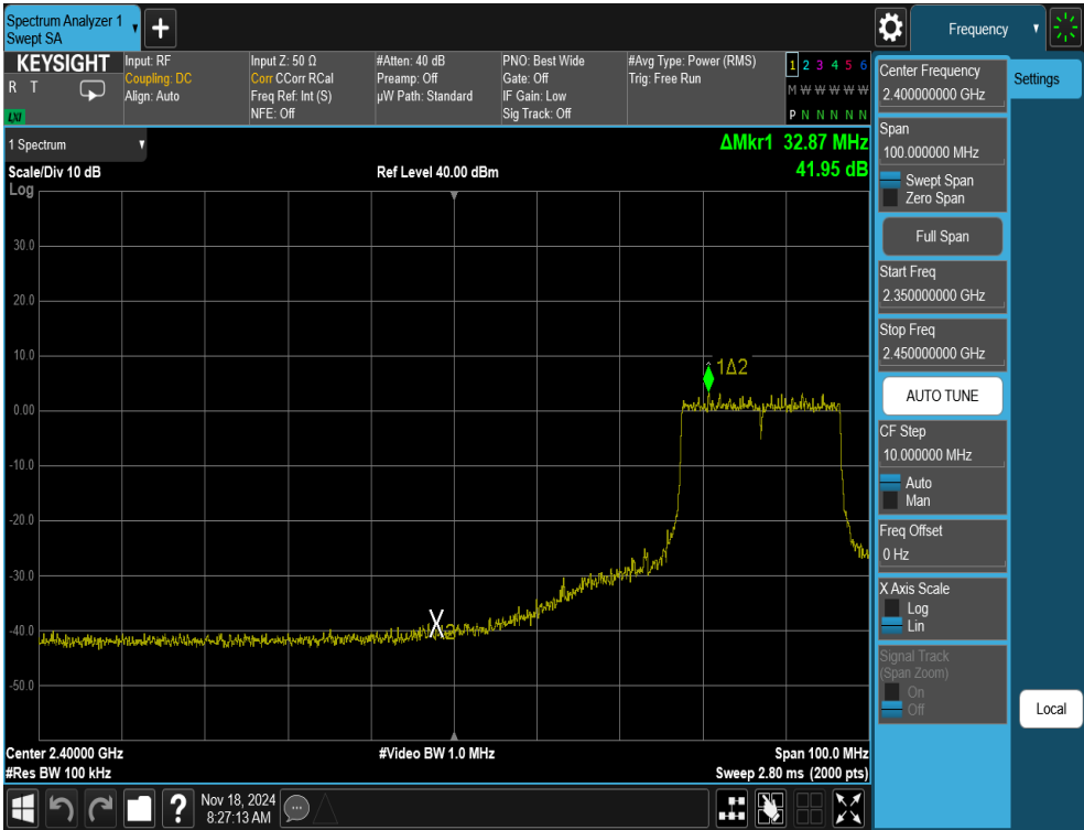
Plot 7-41. Band Edge Antenna WF8 (Common) (802.11ax OFDMA – RU242 – Ch. 6(Low Channel))
