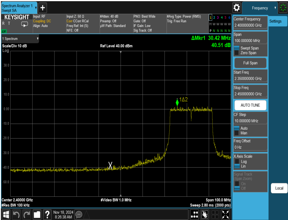
Plot 7-40. Band Edge Antenna WF8 (Common) (802.11ax OFDMA – RU242 – Ch. 5)
