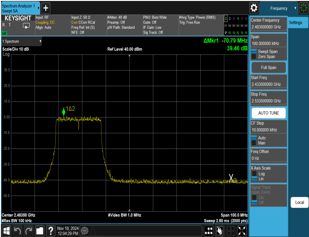
Plot 7-32. Band Edge Antenna WF8 (802.11ax OFDMA – RU242 – Ch. 11)
