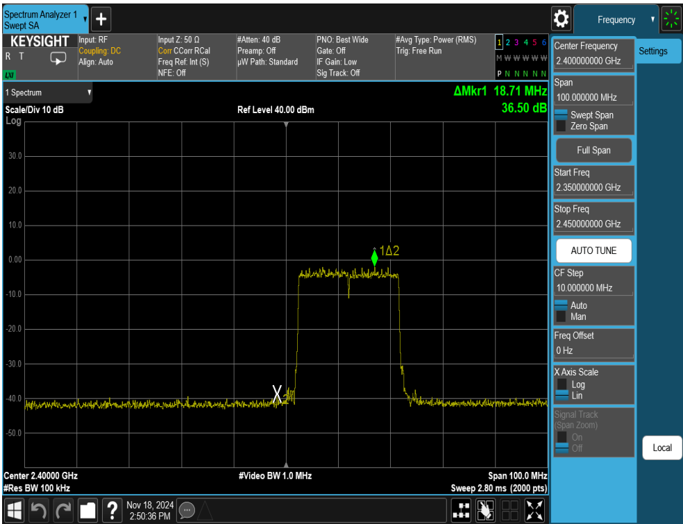
Plot 7-51. Band Edge Antenna WF7b (802.11ax OFDMA – RU242 – Ch. 1)
