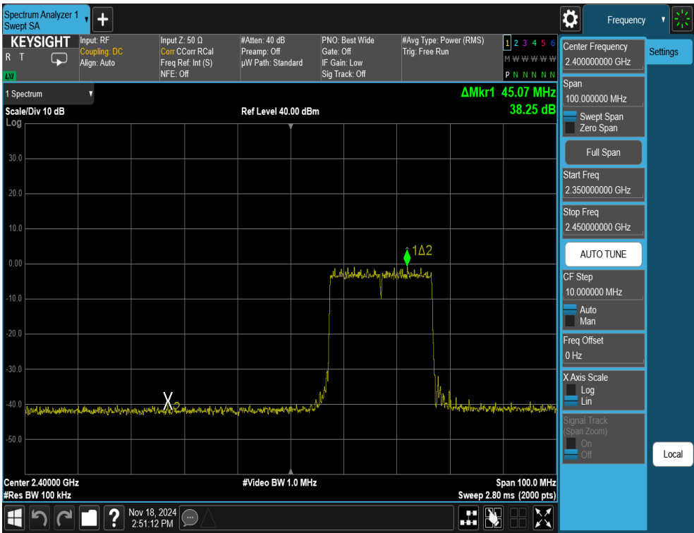
Plot 7-52. Band Edge Antenna WF7b (802.11ax OFDMA – RU242 – Ch. 2)
