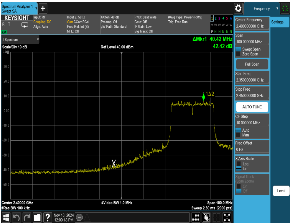
Plot 7-27. Band Edge Antenna WF8 (802.11ax OFDMA – RU242 – Ch. 5)
