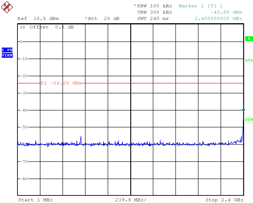
802.11g, Lowest Channel, Plot A
