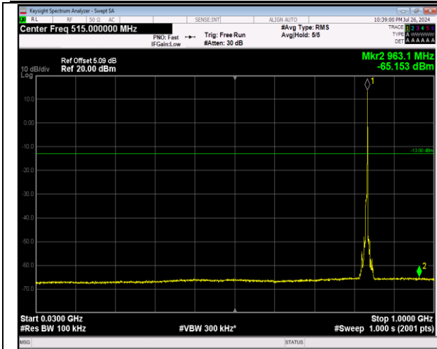
5-5-MHz-3MHz-64QAM-64QAM-20510-20549-1RB#24-ORB#0-30~1000MHz-PASS
