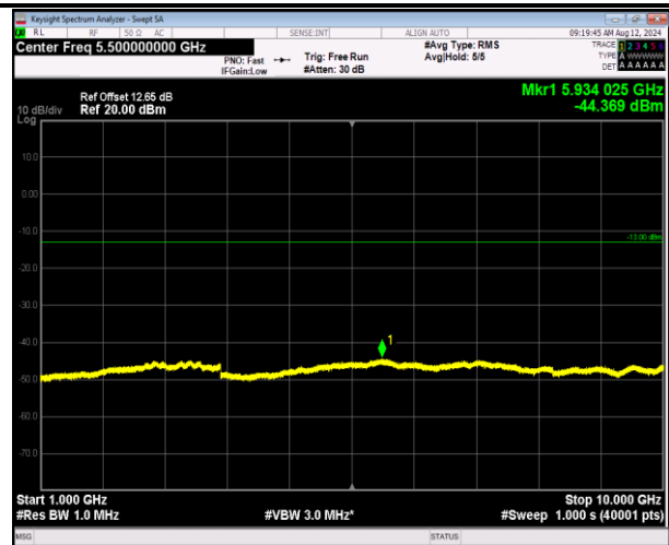
5-5-3MHz-5MHz-16QAM-16QAM-20586-20625-1RB#0-0R B#0-1000~10000MHz-PASS
