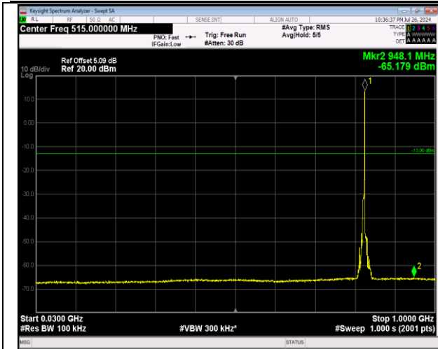
5-5-5MHz-3MHz-64QAM-64QAM-20425-20464-1RB#24-0RB#0-30~1000MHz-PASS
