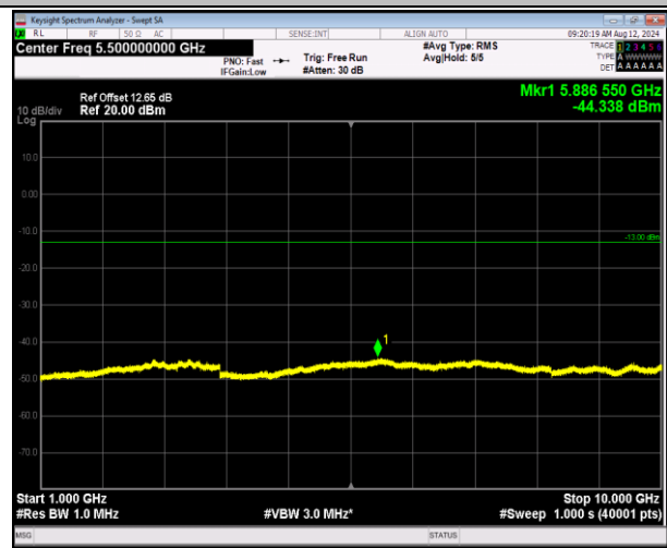
5-5-3MHz-5MHz-QPSK-QPSK-20586-20625-1RB#14-0RB# 0-1000~10000MHz-PASS
