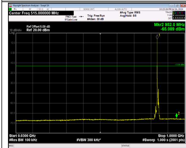
5-5-3MHz-5MHz-64QAM-64QAM-20586-20625-1RB#0-1- RB#24-30~1000MHz-PASS
