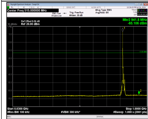
5-5-5MHz-3MHz-64QAM-64QAM-20425-20464-1RB#0-0RB#0-30~1000MHz-PASS
