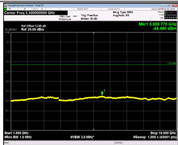
5-5-3MHz-5MHz-64QAM-64QAM-20501-20540-1RB#0-0-1000~10000MHz-PASS
