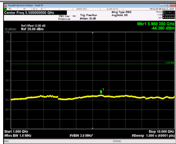
5-5-3MHz-5MHz-16QAM-16QAM-20586-20625-1RB#0-1R B#24-1000~10000MHz-PASS
