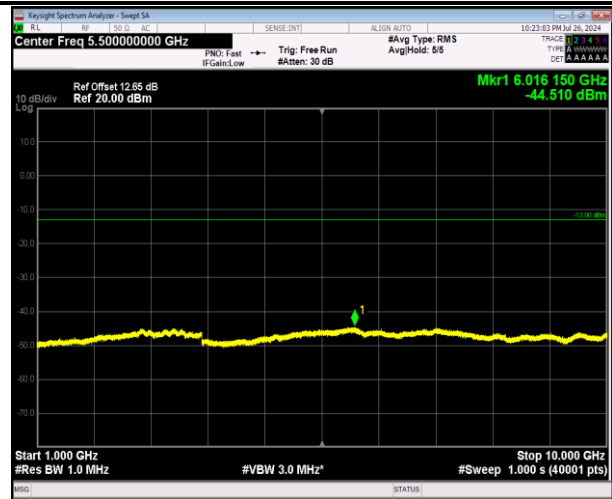
5-5-3MHz-5MHz-64QAM-64QAM-20586-20625-1RB#14-0R B#0-1000~10000MHz-PASS
