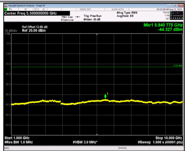
5-5-5MHz-3MHz-16QAM-16QAM-20510-20549-1RB#0-1R B#15-1000~10000MHz-PASS
