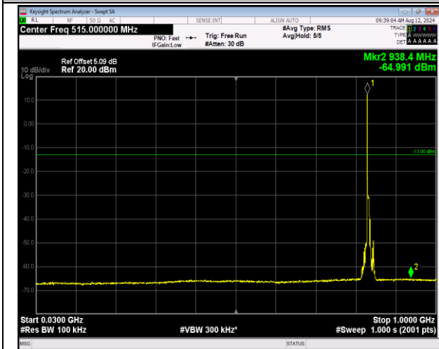
5-5-5MHz-3MHz-QPSK-QPSK-20510-20549-1RB#0-0RB #0-30~1000MHz-PASS
