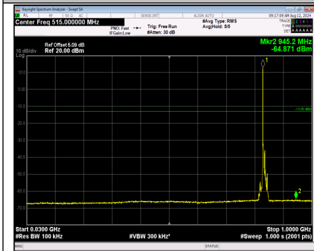
5-5-3MHz-5MHz-16QAM-16QAM-20501-20540-1RB#0-1 RB#24-30~1000MHz-PASS
