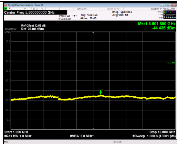
5-5-3MHz-5MHz-QPSK-QPSK-20501-20540-1RB#0-1RB#2 4-1000~10000MHz-PASS
