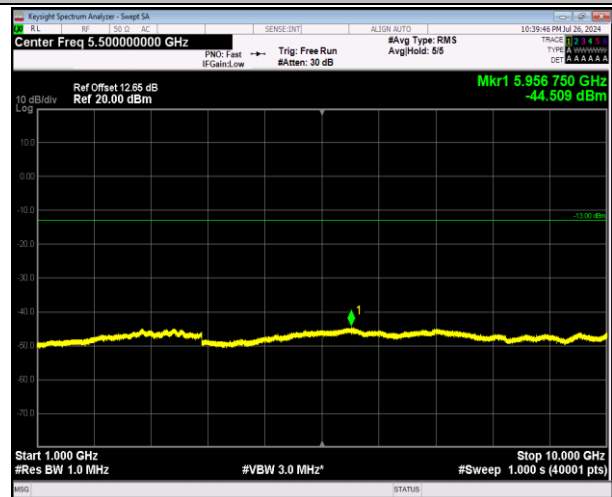
5-5-5MHz-3MHz-64QAM-64QAM-20510-20549-1RB#0-0-1RB#15-1000~10000MHz-PASS
