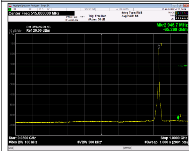
5-5-MHz-3MHz-64QAM-64QAM-20510-20549-25RB#0-15RB#0-30~1000MHz-PASS
