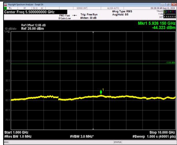
5-5-5MHz-3MHz-16QAM-16QAM-20425-20464-25RB#0-15RB#0-1000~10000MHz-PASS
