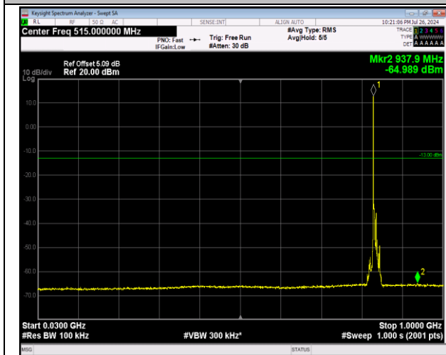
5-5-3MHz-5MHz-64QAM-64QAM-20501-20540-1RB#0-0-24~30~1000MHz-PASS
