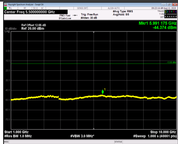
5-5-3MHz-5MHz-16QAM-16QAM-20586-20625-15RB#0-25 RB#0-1000~10000MHz-PASS
