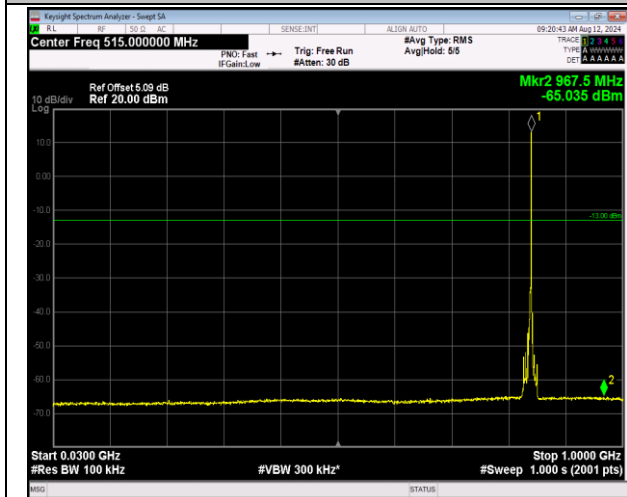
5-5-3MHz-5MHz-16QAM-16QAM-20586-20625-1RB#14-1 ORB#0-30~1000MHz-PASS
