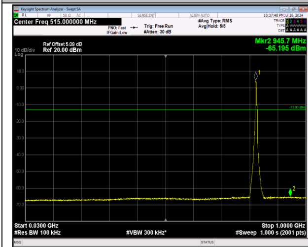
5-5-5MHz-3MHz-64QAM-64QAM-20425-20464-25RB#0-15RB#0-30~1000MHz-PASS
