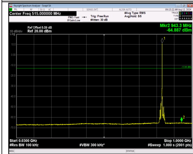
5-5-3MHz-5MHz-QPSK-QPSK-20501-20540-1RB#14-0R B#0-30~1000MHz-PASS
