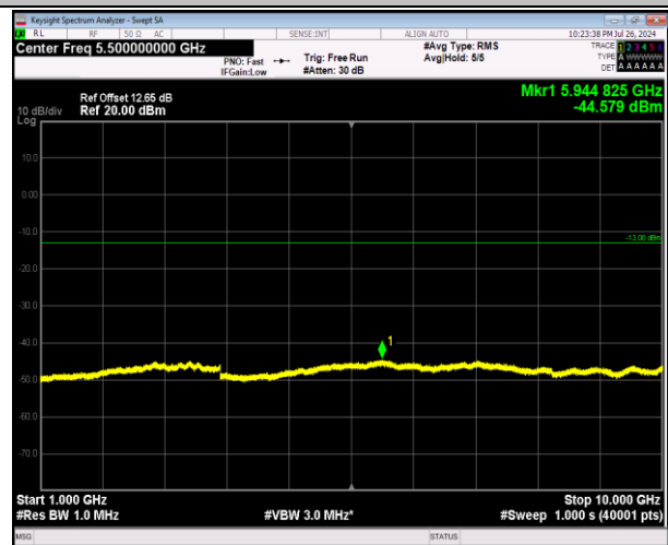
5-5-3MHz-5MHz-64QAM-64QAM-20586-20625-1RB#0-1R B#24-1000~10000MHz-PASS
