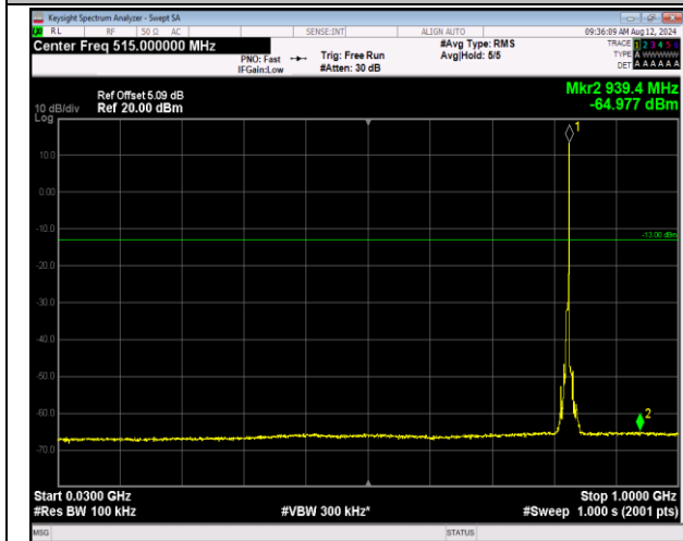
5-5-5MHz-3MHz-16QAM-16QAM-20425-20464-1RB#24- ORB#0-30~1000MHz-PASS
