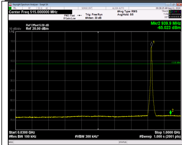
5-5-5MHz-3MHz-16QAM-16QAM-20425-20464-25RB#0-0-15RB#0-30~1000MHz-PASS
