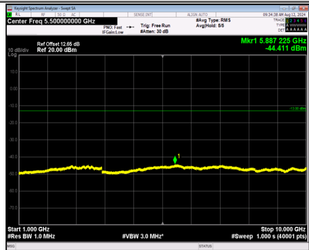
5-5-5MHz-3MHz-QPSK-QPSK-20425-20464-1RB#0-0RB#0 -1000~10000MHz-PASS
