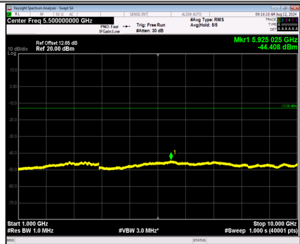
5-5-3MHz-5MHz-16QAM-16QAM-20501-20540-1RB#14-0R B#0-1000~10000MHz-PASS
