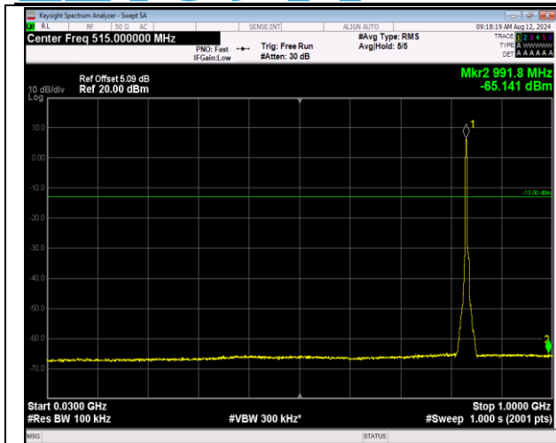
5-5-3MHz-5MHz-16QAM-16QAM-20501-20540-15RB#0-0-25RB#0-30~1000MHz-PASS
