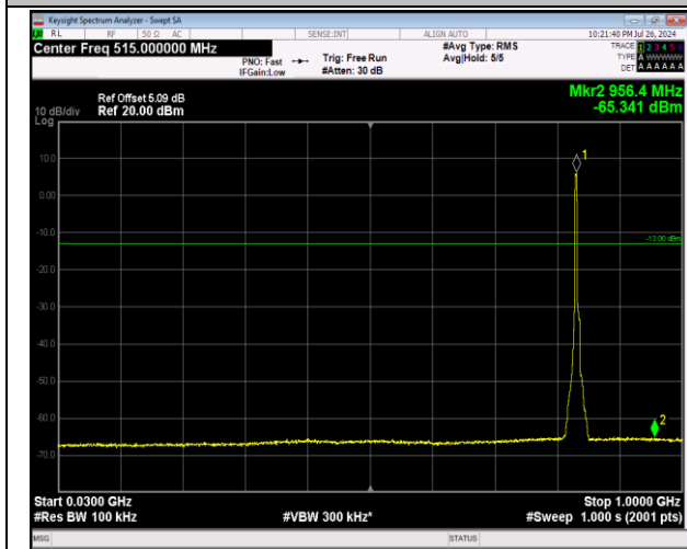
5-5-3MHz-5MHz-64QAM-64QAM-20501-20540-15RB#0- 25RB#0-30~1000MHz-PASS
