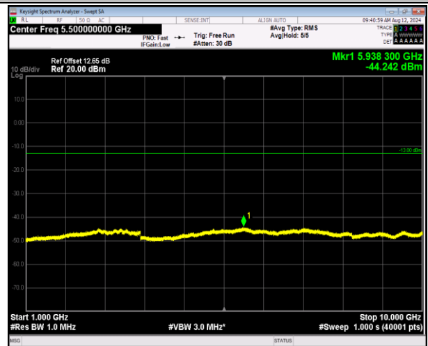
5-5-5MHz-3MHz-16QAM-16QAM-20510-20549-1RB#24-0R B#0-1000~10000MHz-PASS
