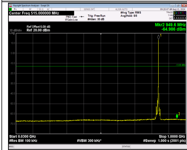
5-5-3MHz-5MHz-QPSK-QPSK-20586-20625-1RB#14-0RB B#0-30~1000MHz-PASS
