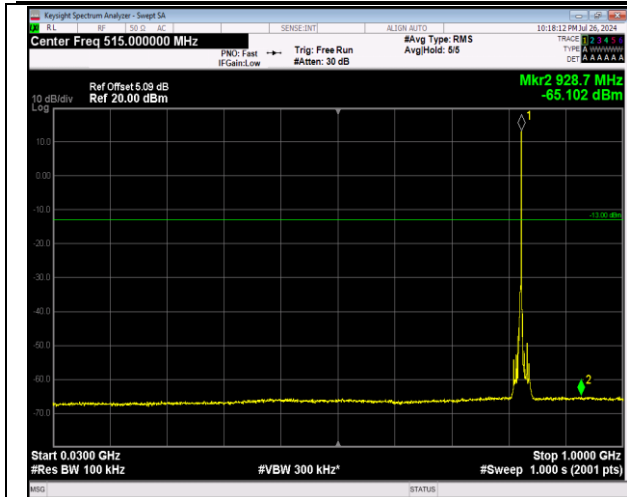
5-5-3MHz-5MHz-64QAM-64QAM-20416-20455-1RB#14-ORB#0-30~1000MHz-PASS
