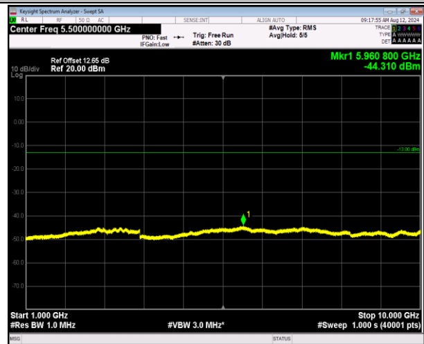
5-5-3MHz-5MHz-QPSK-QPSK-20501-20540-15RB#0-25RB #0-1000~10000MHz-PASS
