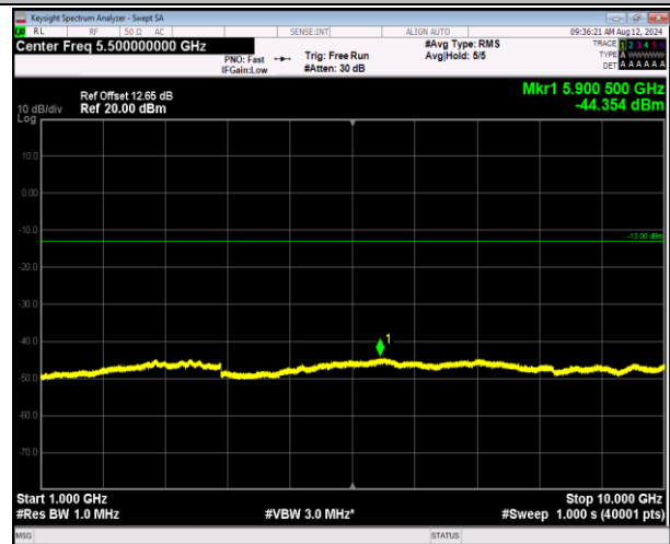
5-5-5MHz-3MHz-16QAM-16QAM-20425-20464-1RB#24-0R B#0-1000~10000MHz-PASS
