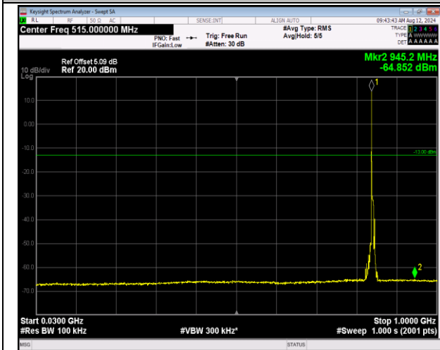
5-5-MHz-3MHz-QPSK-QPSK-20595-20634-1RB#0-0RB#0-30~1000MHz-PASS
