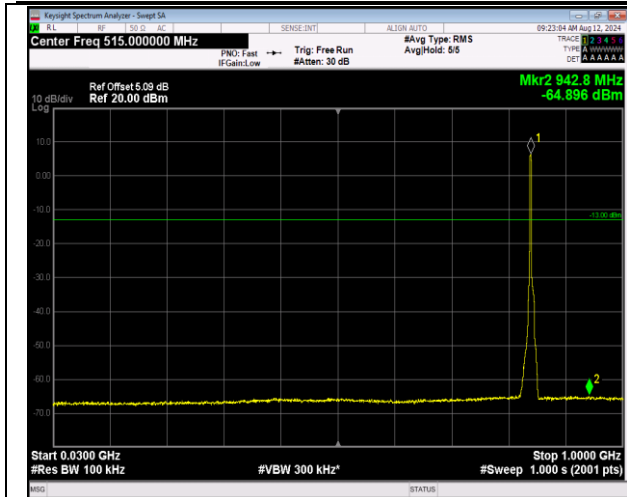
5-5-3MHz-5MHz-16QAM-16QAM-20586-20625-15RB#0-0- 25RB#0-30~1000MHz-PASS
