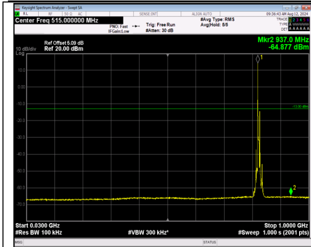
5-5-5MHz-3MHz-QPSK-QPSK-20425-20464-1RB#0-1RB #15-30~1000MHz-PASS
