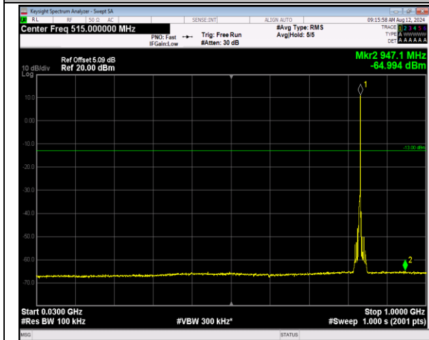
5-5-3MHz-5MHz-16QAM-16QAM-20501-20540-1RB#14-1 ORB#0-30~1000MHz-PASS
