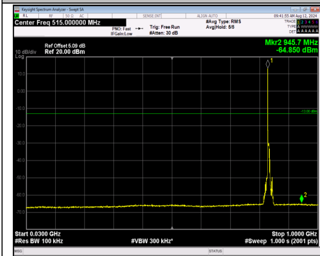
5-5-5MHz-3MHz-16QAM-16QAM-20510-20549-1RB#0-1 RB#15-30~1000MHz-PASS
