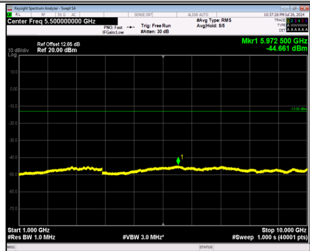
5-5-5MHz-3MHz-64QAM-64QAM-20425-20464-1RB#0-1RB#15-1000~10000MHz-PASS
