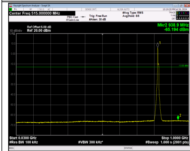
5-5-3MHz-5MHz-64QAM-64QAM-20416-20455-15RB#0-25RB#0-30~1000MHz-PASS
