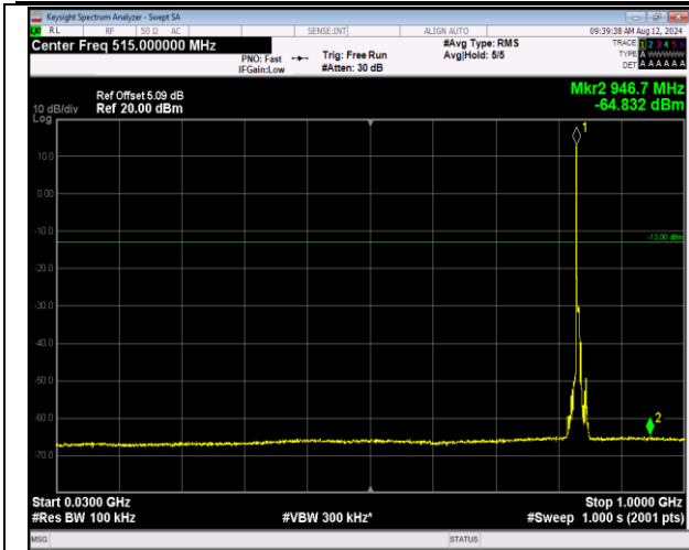
5-5-5MHz-3MHz-16QAM-16QAM-20510-20549-1RB#0-0 RB#0-30~1000MHz-PASS
