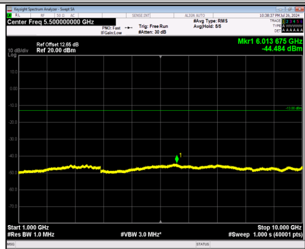
5-5-5MHz-3MHz-64QAM-64QAM-20510-20549-1RB#0-0-0RB#0-1000~10000MHz-PASS
