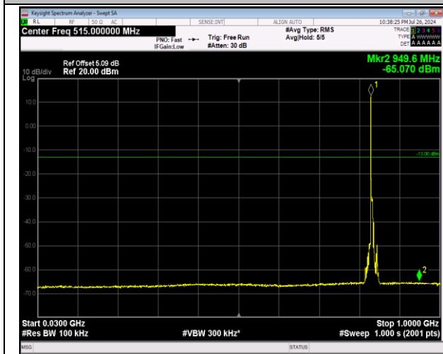
5-5-5MHz-3MHz-64QAM-64QAM-20510-20549-1RB#0-0-0RB#0-30~1000MHz-PASS
