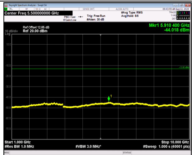
5-5-MHz-3MHz-QPSK-QPSK-20595-20634-1RB#0-0RB#0-1000~10000MHz-PASS
