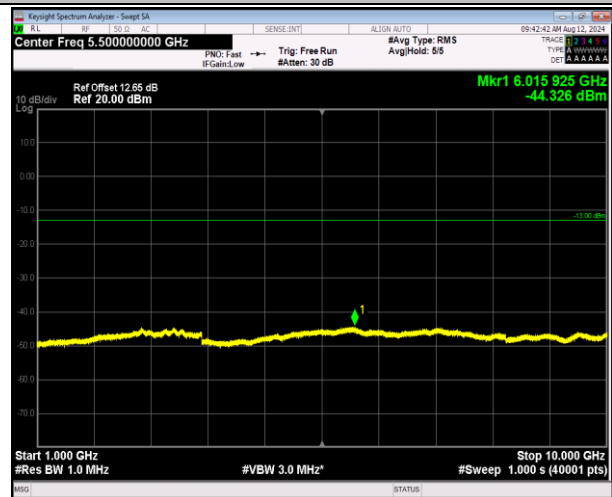
5-5-5MHz-3MHz-QPSK-QPSK-20510-20549-25RB#0-15RB #0-1000~10000MHz-PASS
