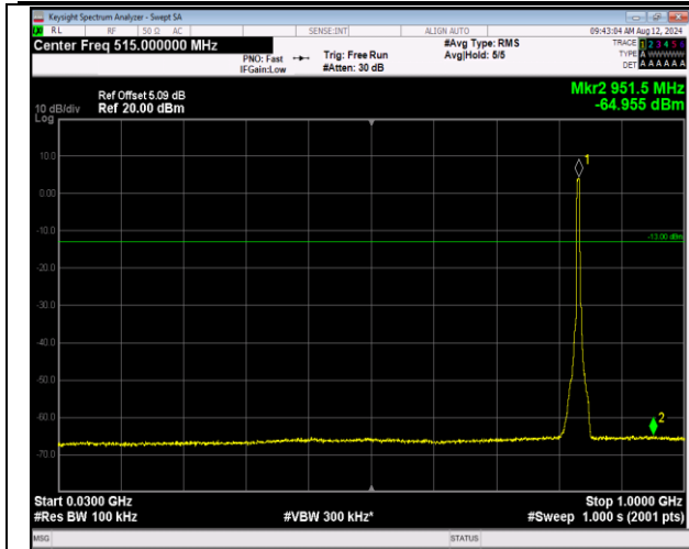
5-5-5MHz-3MHz-16QAM-16QAM-20510-20549-25RB#0-0-15RB#0-30~1000MHz-PASS
