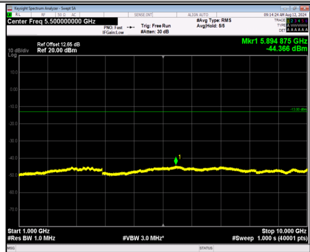
5-5-3MHz-5MHz-QPSK-QPSK-20501-20540-1RB#0-0RB#0-1000~10000MHz-PASS
