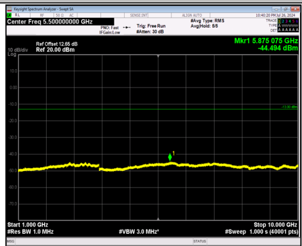
5-5-MHz-3MHz-64QAM-64QAM-20510-20549-25RB#0-15RB#0-1000~10000MHz-PASS
