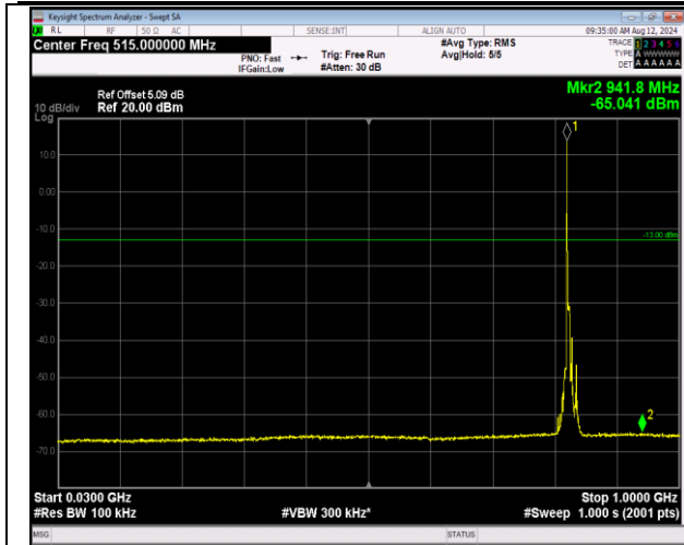
5-5-5MHz-3MHz-16QAM-16QAM-20425-20464-1RB#0-0 RB#0-30~1000MHz-PASS
