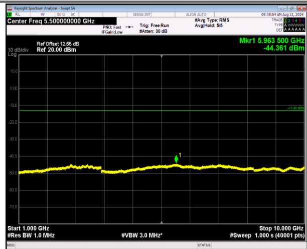
5-5-5MHz-3MHz-QPSK-QPSK-20425-20464-25RB#0-15RB #0-1000~10000MHz-PASS
