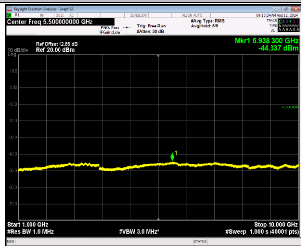
5-5-3MHz-5MHz-QPSK-QPSK-20501-20540-1RB#14-0RB# 0-1000~10000MHz-PASS
