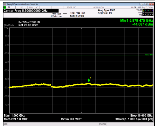
5-5-5MHz-3MHz-QPSK-QPSK-20510-20549-1RB#0-0RB#0 -1000~10000MHz-PASS
