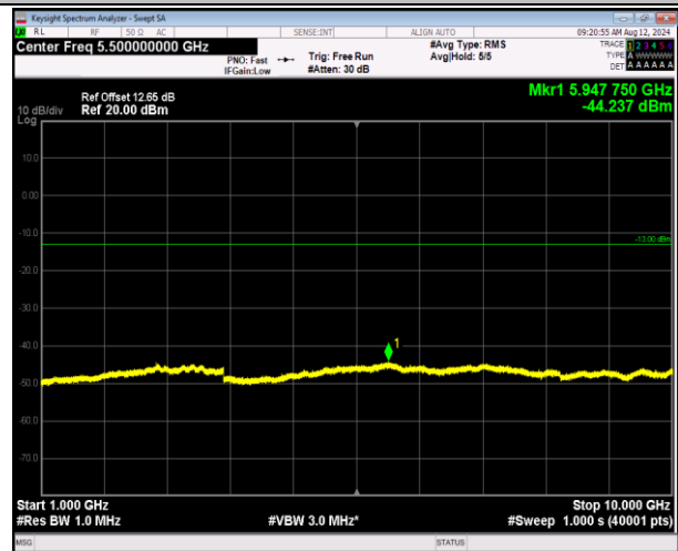
5-5-3MHz-5MHz-16QAM-16QAM-20586-20625-1RB#14-0R B#0-1000~10000MHz-PASS
