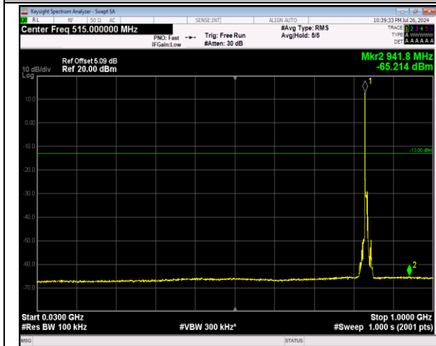
5-5-5MHz-3MHz-64QAM-64QAM-20510-20549-1RB#0-0-1RB#15-30~1000MHz-PASS
