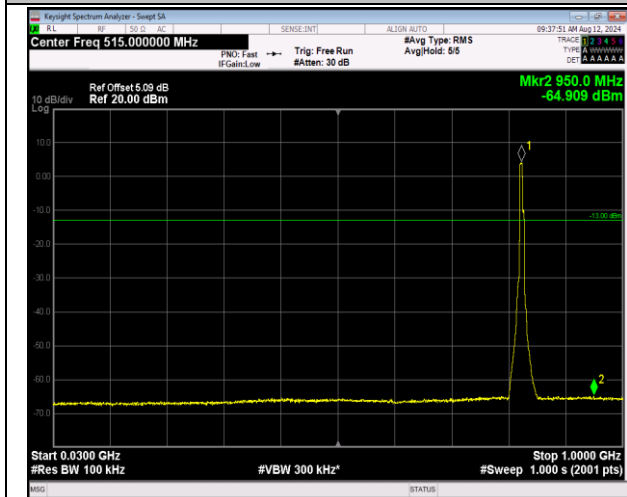
5-5-5MHz-3MHz-QPSK-QPSK-20425-20464-25RB#0-15 RB#0-30~1000MHz-PASS
