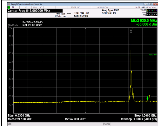
5-5-5MHz-3MHz-64QAM-64QAM-20425-20464-1RB#0-1RB#15-30~1000MHz-PASS
