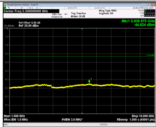
5-5-5MHz-3MHz-64QAM-64QAM-20425-20464-1RB#0-0RB#0-1000~10000MHz-PASS
