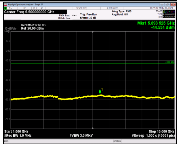
5-5-MHz-3MHz-64QAM-64QAM-20510-20549-1RB#24-ORB#0-1000~10000MHz-PASS
