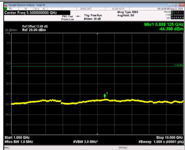
5-5-3MHz-5MHz-QPSK-QPSK-20586-20625-1RB#0-ORB#0 -1000~10000MHz-PASS
