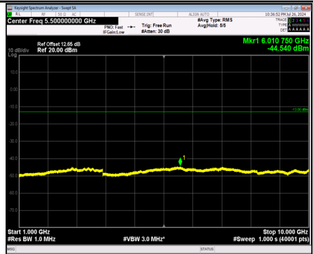
5-5-5MHz-3MHz-64QAM-64QAM-20425-20464-1RB#24-0R B#0-1000~10000MHz-PASS
