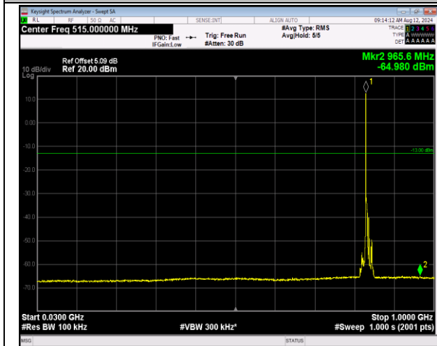
5-5-3MHz-5MHz-QPSK-QPSK-20501-20540-1RB#0-0RB#0-30~1000MHz-PASS
