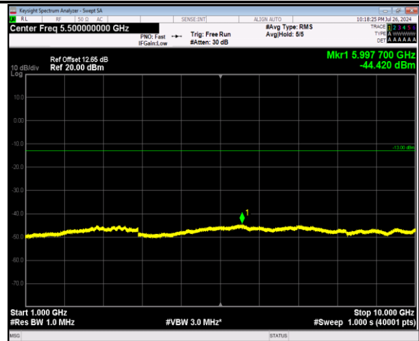
5-5-3MHz-5MHz-64QAM-64QAM-20416-20455-1RB#14-ORB#0-1000~10000MHz-PASS
