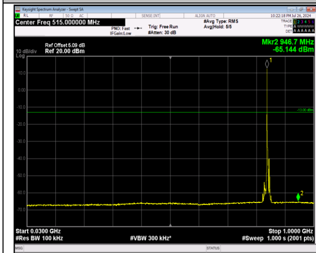
5-5-3MHz-5MHz-64QAM-64QAM-20586-20625-1RB#0-0- RB#0-30~1000MHz-PASS
