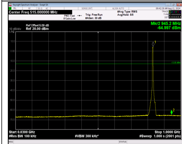
5-5-5MHz-3MHz-QPSK-QPSK-20510-20549-25RB#0-15 RB#0-30~1000MHz-PASS
