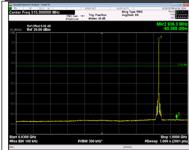
5-5-3MHz-5MHz-64QAM-64QAM-20501-20540-1RB#14- ORB#0-30~1000MHz-PASS
