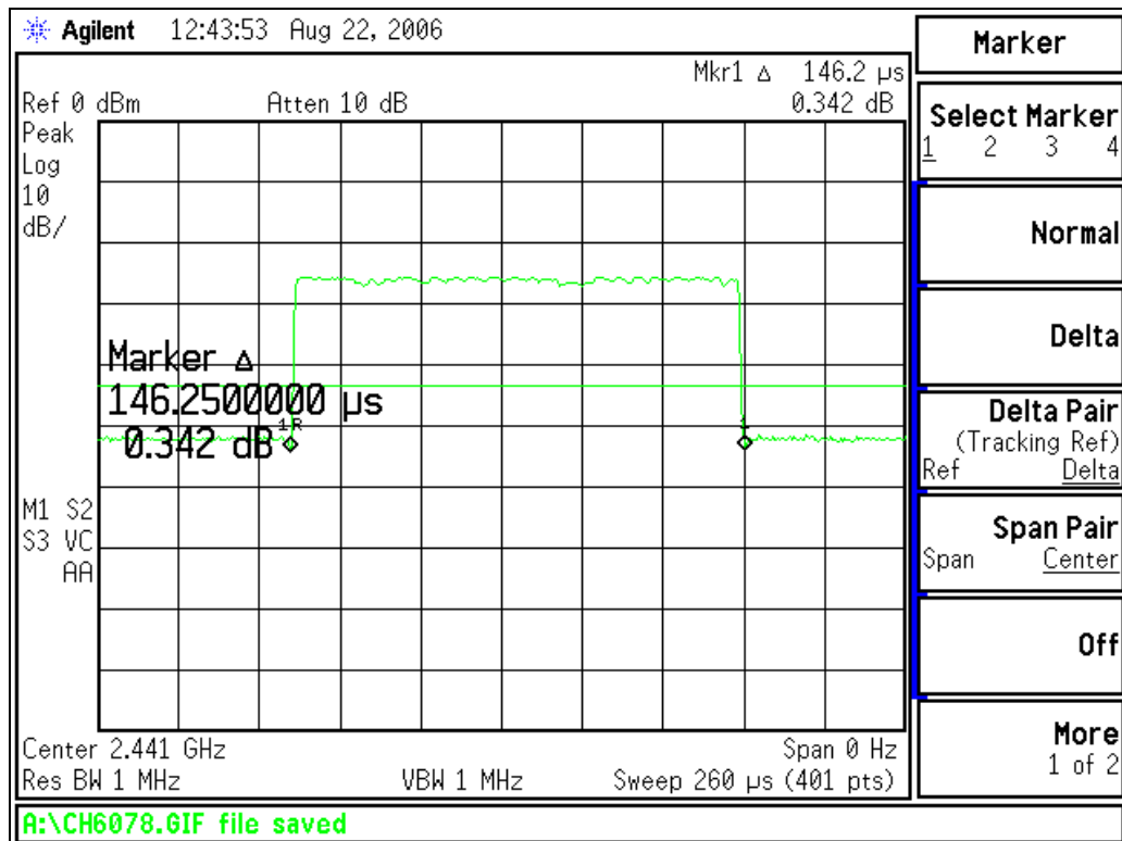
Channel occupancy
