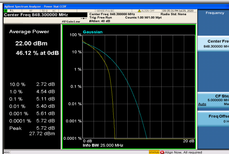
Band5-1.4MHz-QPSK-20643-6RB#0
