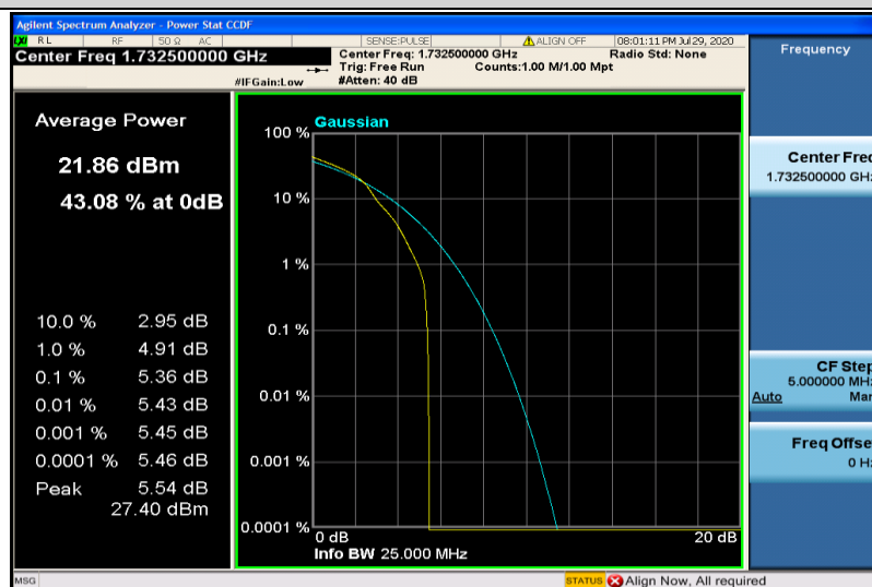
Band4-5MHz-16QAM-20175-1RB#0
