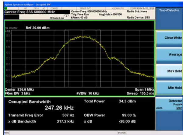
WCDMA Band V CH-Middle
