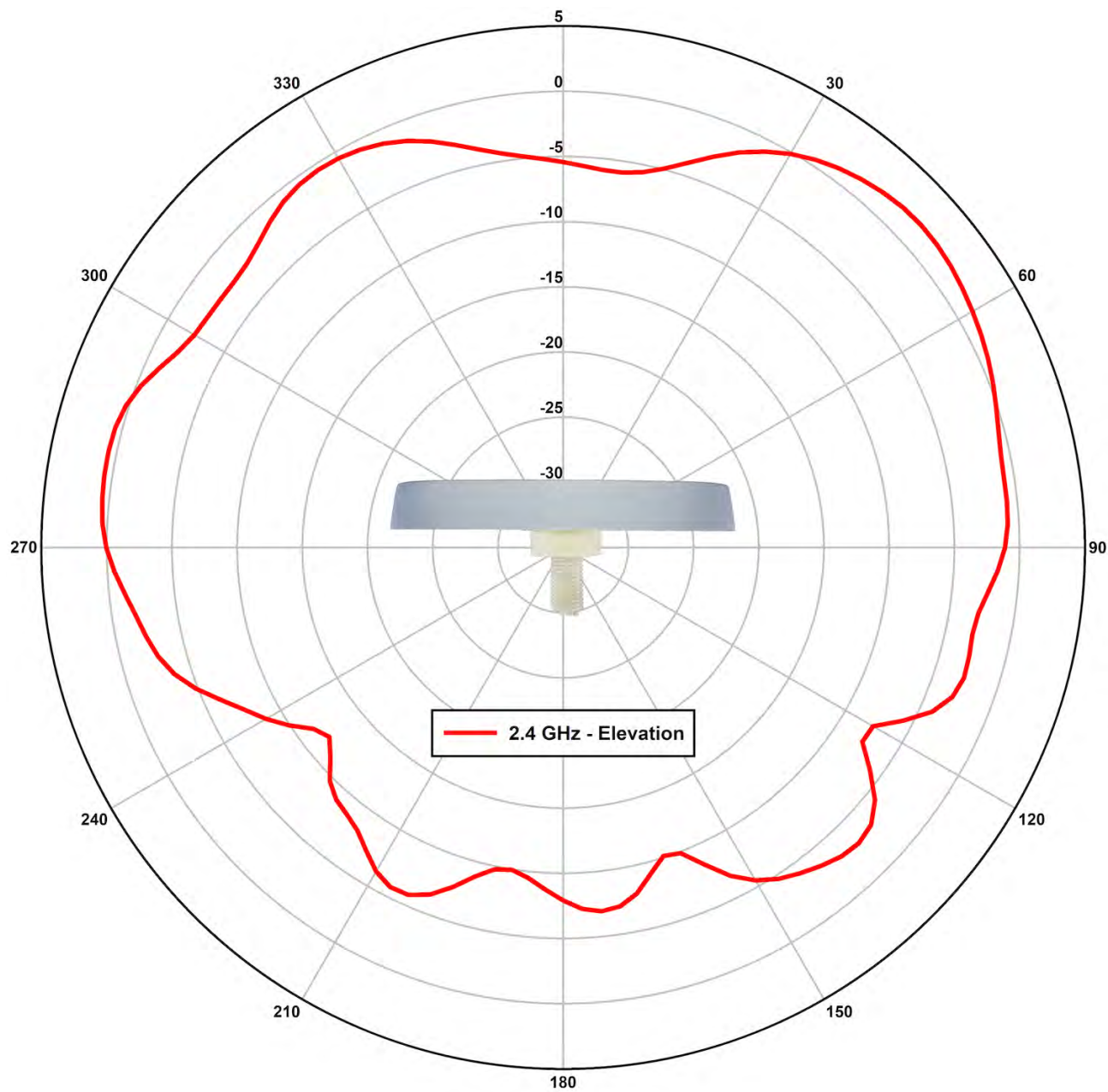
Figure 22 2.4 GHz - Elevation - Port F
