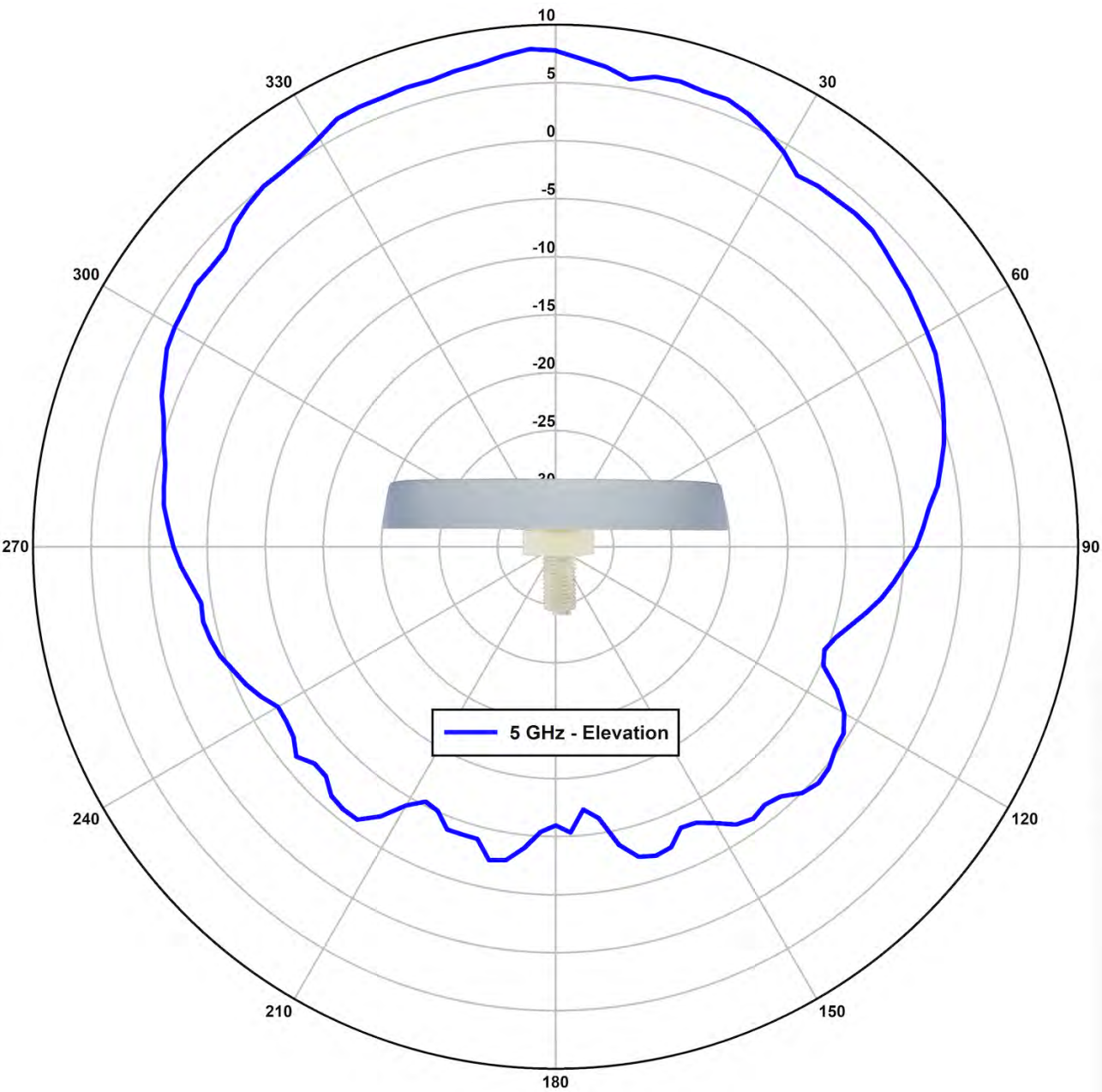
Figure 6 5 GHz - Elevation - Port C
