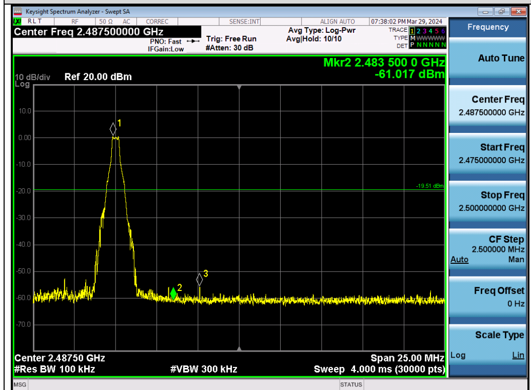
Test_Graph_BR_Chain A_2480_1Mbps_Higher Band Edge Emissions
