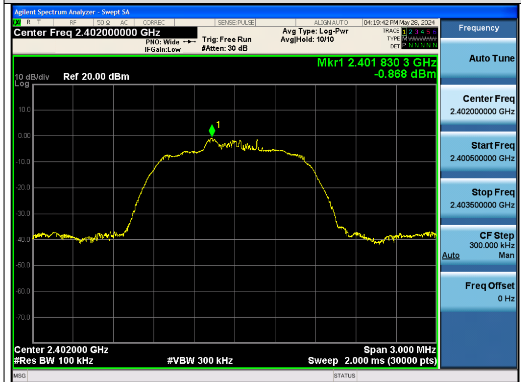
Test_Graph_EDR_Chain A_2402_2Mbps_Reference Level
