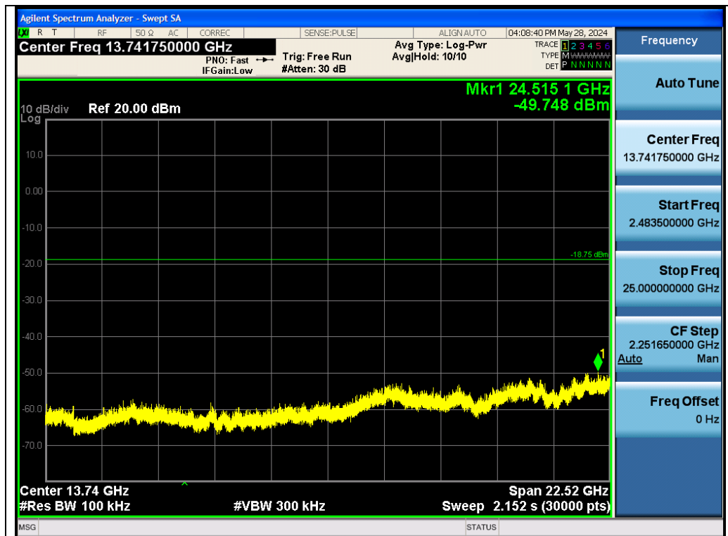
Test_Graph_BR_Chain A_2402_1Mbps_Higher Band Emissions
