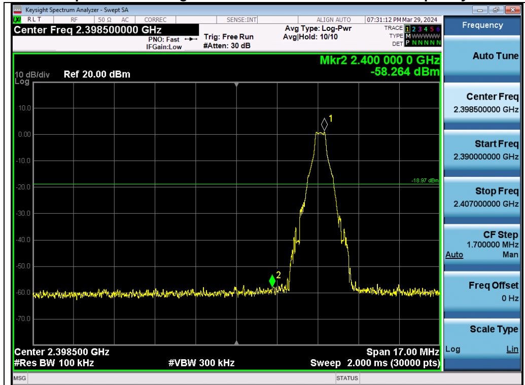
Test_Graph_BR_Chain A_2402_1Mbps_Lower Band Edge Emissions
