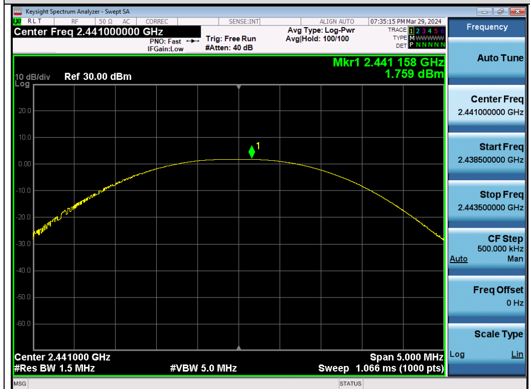
Test_Graph_BR_Chain A_2441_1Mbps_Peak Power
