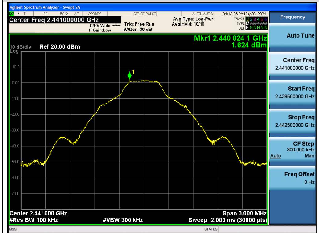
Test_Graph_BR_Chain A_2441_1Mbps_Reference Level
