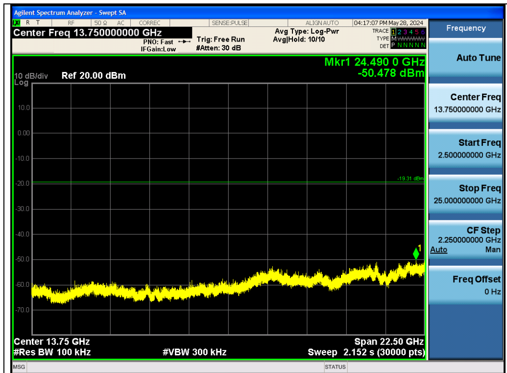
Test_Graph_BR_Chain A_2480_1Mbps_Higher Band Emissions
