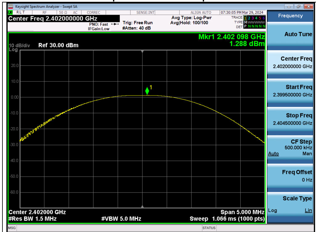
Test_Graph_BR_Chain A_2402_1Mbps_Peak Power
